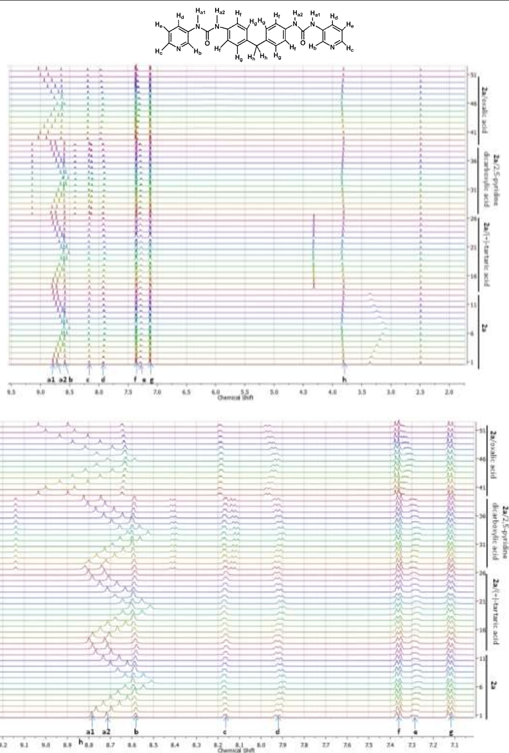
Figure S17 Temperature-dependent ^1\text{H} NMR spectra of 2a /oxalic acid, 2, 5-pyridinedicarboxylic acid and (+)-tartaric acid in d^6 -DMSO (ratio is 1:1, temperature is change 25 °C to 80 °C, and then down to 25 °C)
