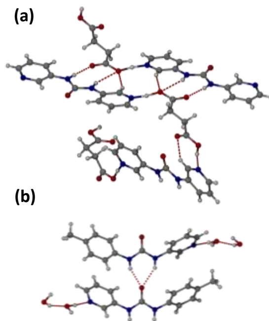
Fig. 8 (a) X-ray crystal structure of the neutral co-crystal of di-3-pyridyl urea and succinic acid 40 showing acid-pyridyl and urea acid hydrogen bonding motifs; (b) X-ray structure of the dihydrate of 3-pyridyl-4-tolyl urea showing the rotation of the aryl group out of the plane of the urea functionality to give a urea \alpha -tape hydrogen bonding motif. 37
