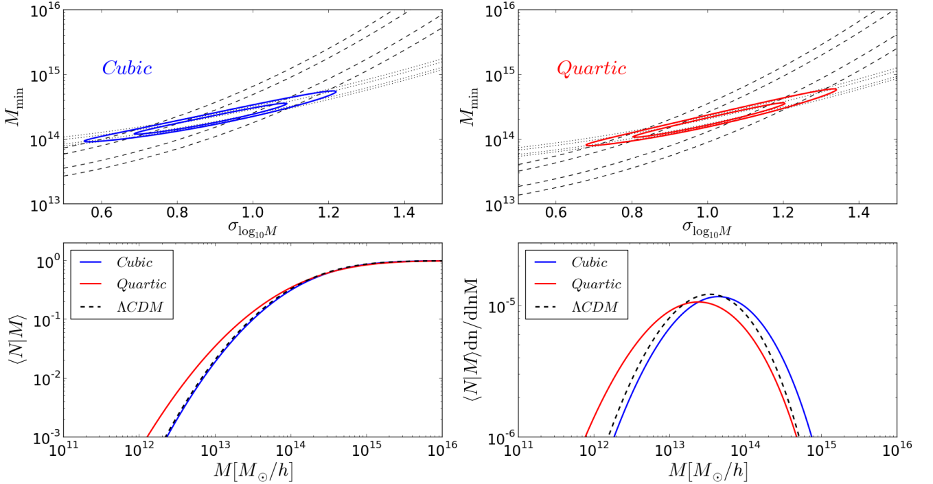
FIG. 5. The upper panels show the 68% and 95% confidence contours on the M_{\min} and \sigma_{\log_{10} M} parameters of Eq. (24) obtained using Eq. (25) for the full variants of the Cubic (left) and Quartic (right) Galileon models. The black dashed and dotted contours indicate the constraints derived by using only \chi^2_{b_g} and only \chi^2_{n_g} in Eq. (25), respectively. The solid contours show the combined constraints. The lower left and lower right panels show, respectively, the best-fitting \langle N|M \rangle and \langle N|M \rangle dn/d\ln M for the full Cubic (blue) and Quartic (red) Galileon models, and \Lambda CDM with WMAP9 parameters [23] (black dashed). The quantity plotted in the lower right panel shows the contribution from haloes of different mass to the galaxy number density.
