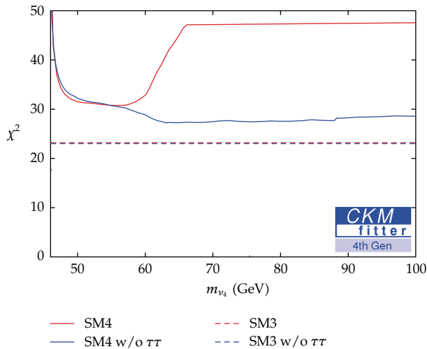
FIGURE 9: Best fit results in dependence of the mass of the fourth neutrino. As soon as H \rightarrow \tau^+ \tau^- is included, the only remaining possibility for the SM4 is to open up the decay channel H \rightarrow \nu_4 \nu_4 . Figure from [18].
