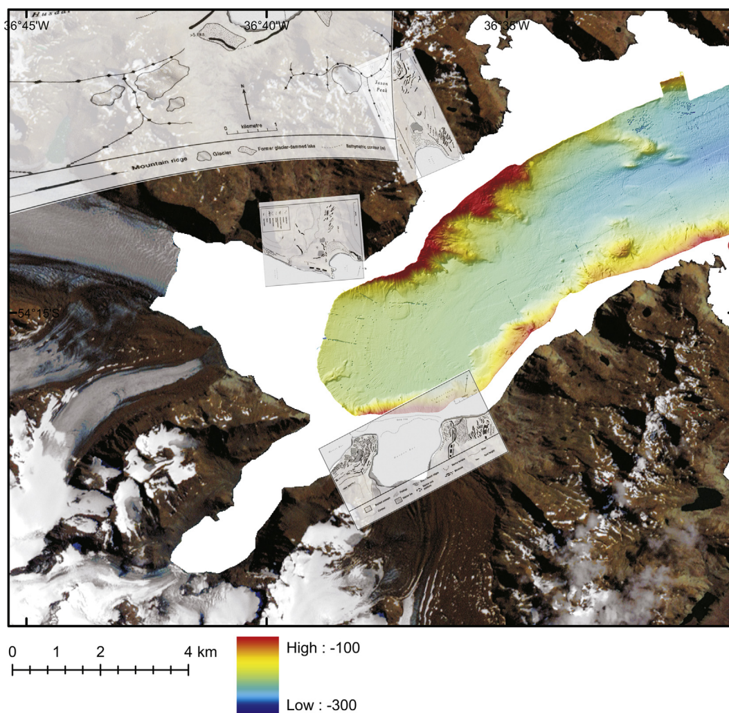
Appendix Fig. A2. Multibeam swath bathymetry of Cumberland Bay West, South Georgia combined with Fig. 8a (Mercer Bay, Harpon Bay and Sphagnum Valley); 8b (Carlita Bay); 8c (Enten Bay); and the lower part of Fig. 10b from Bentley et al. (2007). Although a shallow inner basin is not present on this image it is possible that it may occur just south of Carlita Bay where Fig. 8b of Bentley et al. (2007) documents a series of moraines and lake shorelines associated with an advance of the Neumayer Glacier. These are undated.
