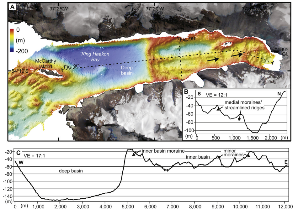
Fig. 9. (A) Multibeam swath bathymetry and geomorphological features of King Haakon Bay, South Georgia. Inset boxes show (B) a transverse cross-section of the medial moraines and (C) a cross section along the fjord.
