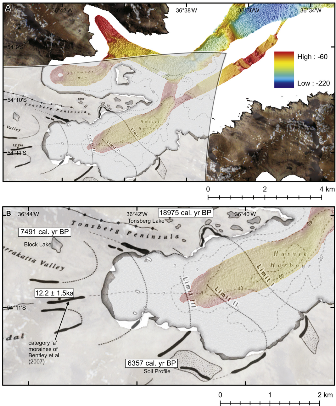
Appendix Fig. A3. Multibeam swath bathymetry of Stromness (upper image) and Husvik (lower image) Harbours combined with Fig. 18 of Bentley et al. (2007) which shows an overview of the geomorphology of Husvik Harbour, its major moraine locations and interpreted ice marginal positions (Limits I–III) that document significant still stands during ice recession from the centre of the fjord. Combined, these figures show the relationship between the onshore and offshore glacial geomorphology including features from which age constraints from cosmogenic isotope exposure age dating and the onset of lake sedimentation are available. Radiocarbon ages from Tønsberg Lake, Block Lake and a soil profile south of Limit III are reported as the mean of the two-sigma range, calibrated using Calib 14C program v7.0 and the SHcal13 calibration curve. The terrestrial moraines in the inner basin of Husvik Harbour are interpreted as marking the oldest mapped ice advance on South Georgia based on cosmogenic ^{10}\text{Be} exposure ages of between 14.2 and 10.6 ka BP, mean 12.2 \pm 1.5 ka BP, from the Husvik medial moraine (Bentley et al., 2007, 'category a' moraine). These 'category a' moraines have been correlated on geomorphological grounds with the oldest terrestrial moraine ridges in Antarctic Bay, Possession Bay and Moraine Fjord (Zenker Ridge) to the west of Cumberland Bay East (Appendix Figs. A4, A5, and A1, respectively).
