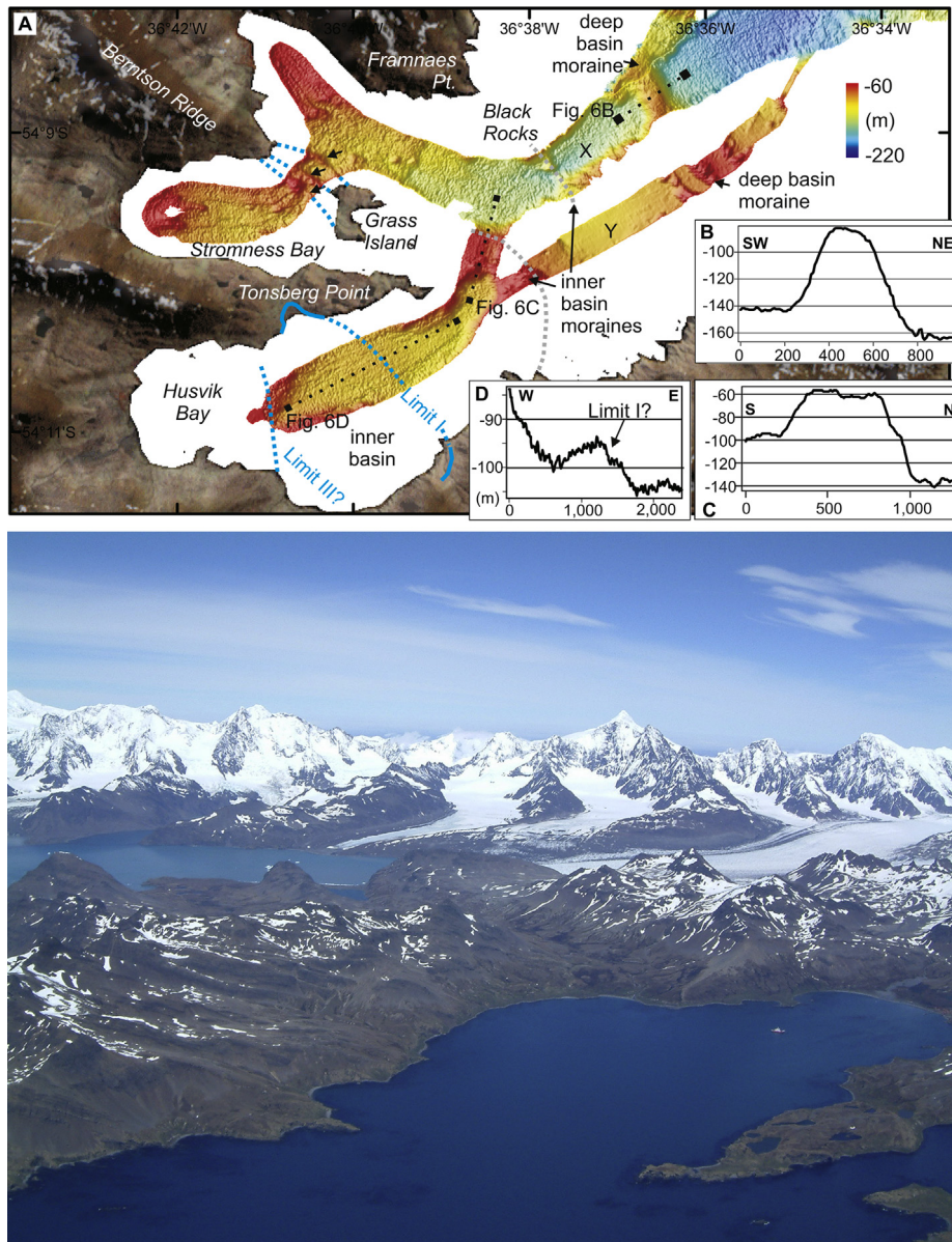
Fig. 6. (A, upper panel). Multibeam swath bathymetry and geomorphological features of Stromness and Husvik Bays, South Georgia. Inset boxes show (B) a cross section of the inner basin moraine (C) a cross section of the outer deep basin moraine, and (D) the moraine associated with Limit I. Fig. 6 (lower panel). Oblique aerial photograph of Husvik Bay and Tønsberg Point facing approximately south west. HMS Endurance is present in Husvik Harbour (to the right of the image) for scale.
