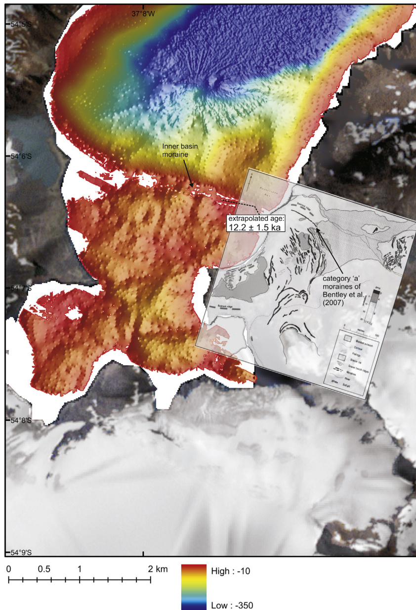
Appendix Fig. A5. Multibeam swath bathymetry of Possession Bay combined with Fig. 16a of Bentley et al. (2007) which is a geomorphological map of the valley on the south east shore of Possession Bay. This shows the outermost of a series of latero-frontal terrestrial moraine loops deposited by mountain ice to the south coalescing with the outer latero-frontal moraines of the former fjord ice and a prominent inner basin moraine in the fjord. This is a 'category a' moraine correlated on geomorphological grounds with the oldest terrestrial moraine ridges in Husvik Harbour, Antarctic Bay and Moraine Fjord (Zenker Ridge) to the west of Cumberland Bay East (Appendix Figs. A3, A4, and A1, respectively).
