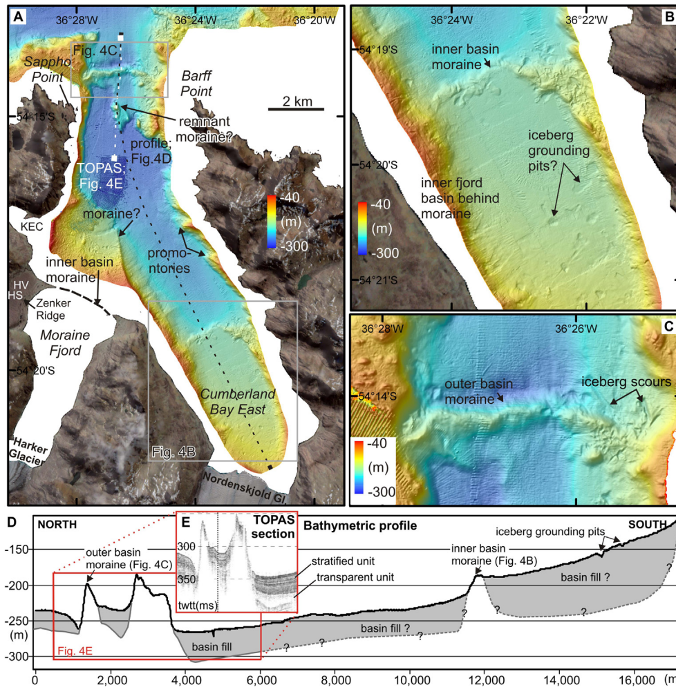
Fig. 4. (A) Multibeam swath bathymetry of Cumberland Bay East, South Georgia. HV: Hamburg Valley; HS: Hestlesletten; KEC: King Edward Cove. Inset boxes show (B) an enlarged image of the inner basin and inner basin moraine, (C) an enlarged image of the outer basin moraine, (D) a cross section along the fjord and (E) a TOPAS sub-bottom profile collected on the RRS James Clark Ross cruise JR224 shows cross-sections of both the outer deep basin moraine as well as the second remnant moraine landward of this feature.
