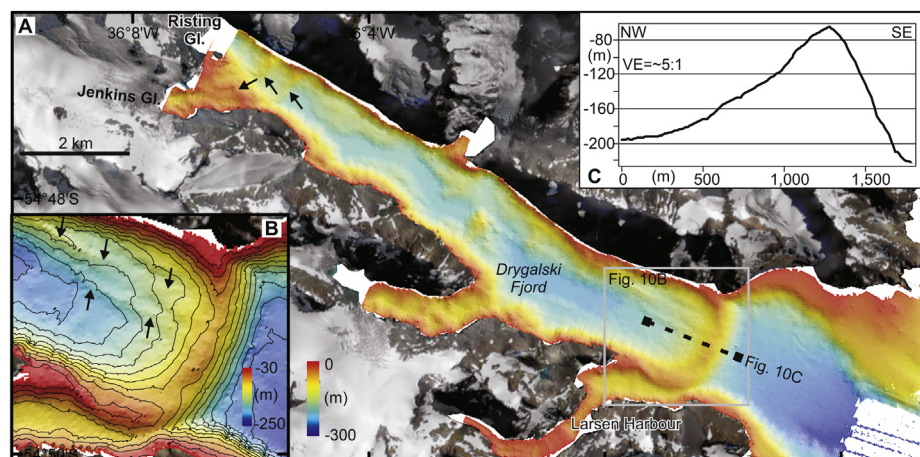
Fig. 10. (A) Multibeam swath bathymetry and geomorphological features of Drygalski Fjord, South Georgia. Inset boxes show (B) an enlarged image of the inner basin moraine showing the erosional grooves that characterise the back slope of the moraine (black arrows) and (C) a cross section of the inner basin moraine.
