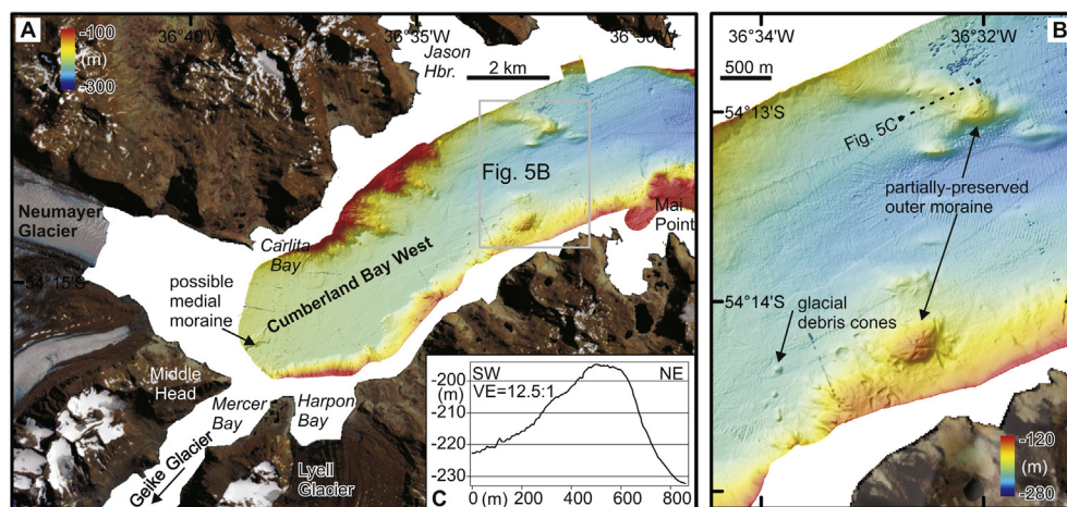
Fig. 5. (A) Multibeam swath bathymetry of Cumberland Bay West, South Georgia. Inset boxes show (B) an enlarged image of the partially-preserved outer basin moraine, and (C) a cross section of the outer basin moraine.
