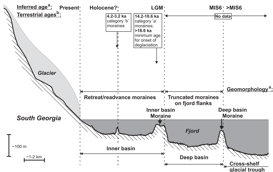
Fig. 11. Cross-section schematic of a typical South Georgia glaciated fjord, showing main geomorphic features, correlation to onshore chronological constraints, and inferred ages from this study. In our model, features seaward of the deep basin moraine on the continental shelf (not shown) are proposed as older than the penultimate glacial episode, MIS6. a this study; b ages from terrestrial studies of Bentley et al. (2007) and Rosqvist et al. (1999).
