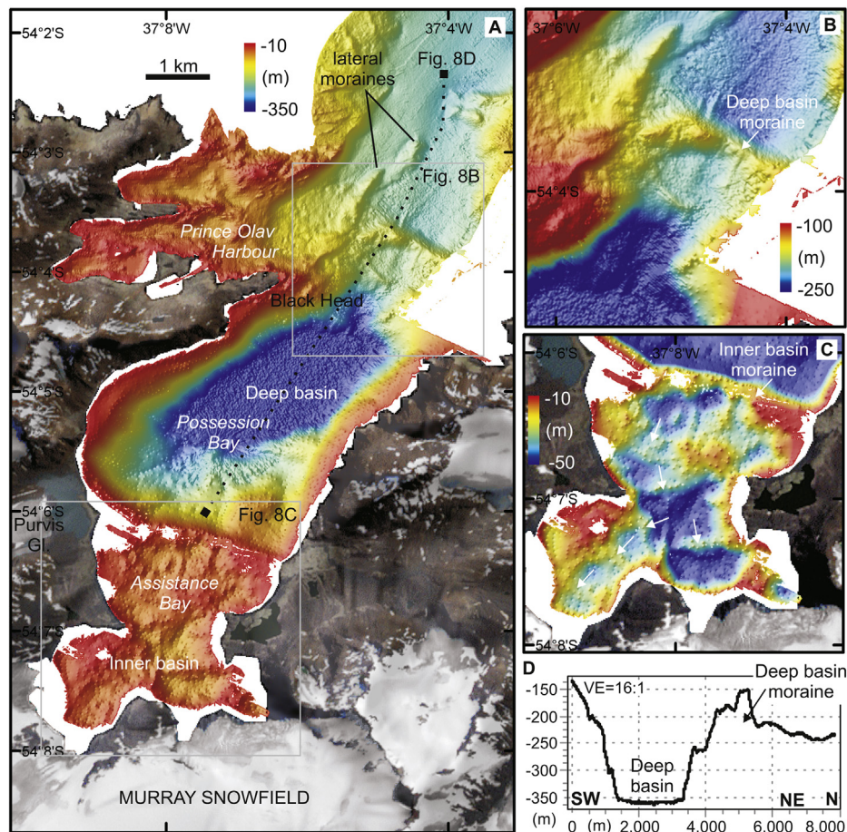
Fig. 8. (A) Multibeam swath bathymetry and geomorphological features of Possession Bay, South Georgia. Inset boxes show (B) an enlarged image of the deep basin moraine, (C) an enlarged image of the inner basin moraine, and (D) a cross section of the deep basin and deep basin moraine. Note differences in depth scales.
