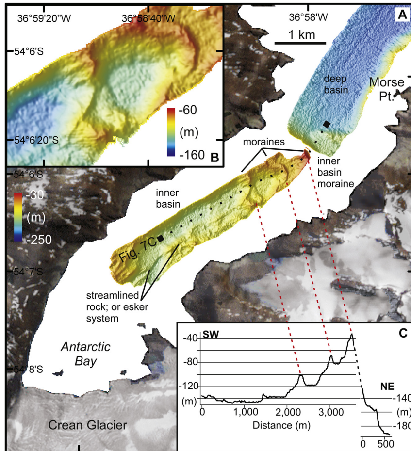
Fig. 7. (A) Multibeam swath bathymetry and geomorphological features of Antarctic Bay, South Georgia. Inset boxes show (B) an enlarged image and (C) cross-section of the moraine complex at the seaward end of the inner basin, comprising at least three ice-marginal limits.
