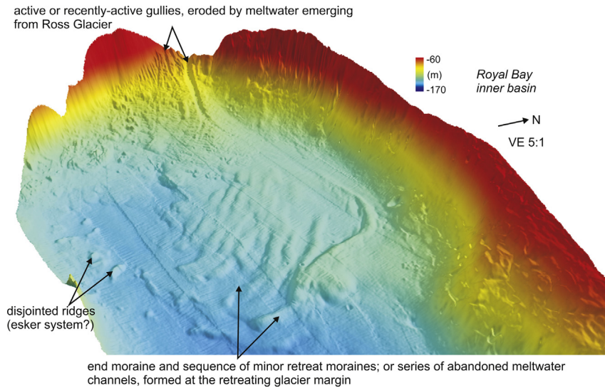
Fig. 3. Oblique perspective image of multibeam swath bathymetry from the inner basin, Royal Bay, showing sea-floor geomorphic features including sets of small ridges and an active or recently-active meltwater gully. Glacier flow, today, is towards the reader. Image is approximately 3 km across in the forefield.
