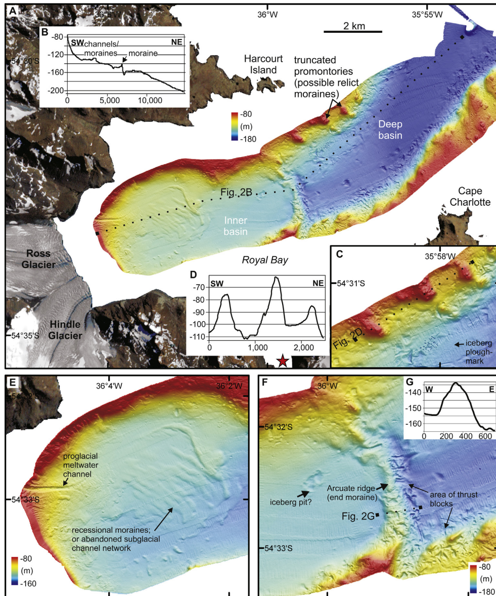
Fig. 2. (A) Multibeam swath bathymetry and geomorphological features of Royal Bay, South Georgia. Inset boxes show (B) a cross section along the fjord, (C) an enlarged image of the truncated ridges or moraines, (D) cross-section of the truncated ridges or moraines (E) an enlarged image of the inner basin, and (F) an enlarged image of the inner basin moraine.
