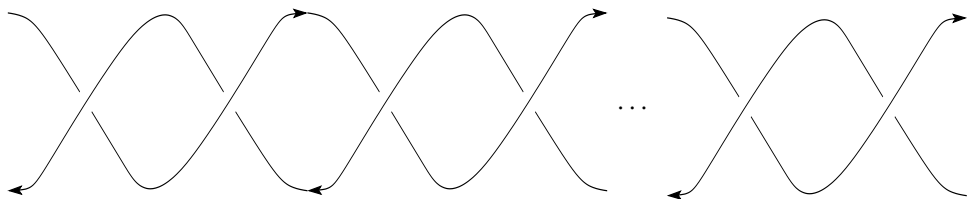
Figure 3: The complex T_k = \bigotimes^k T_1 is the \mathfrak{sl}(n) Khovanov–Rozansky complex corresponding to the diagram above with 2k crossings.
