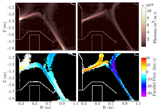
FIG. 9. Tomographically inverted C III (465 nm) emissivity (top) and v_{\parallel} (bottom) profiles in the lower divertor, in L-mode (left) and inter-ELM H-mode (right) phases of MAST single null divertor shot 29 541. Each emissivity/flow profile pair is obtained from a single 1 ms exposure.
