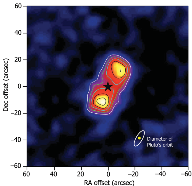
Figure 17. SCUBA-2 image of the debris disc around Fomalhaut at 850\ \mu\text{m} . Contours start at 3\sigma and increase in steps of 2\sigma . The ‘star’ symbol shows the position of Fomalhaut with respect to the disc. The diameter of Pluto’s orbit in our Solar system is also shown, indicating that the disc may represent a Kuiper belt like structure around the star. Image provided courtesy of the SONS Legacy Survey team.
