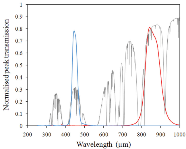
Figure 3. The measured SCUBA-2 bandpass filter profiles at 450 (blue curve) and 850 µm (red), superimposed on the atmospheric transmission curve for Mauna Kea for 1 mm of precipitable water vapour (PWV; grey curve). The atmospheric transmission data are provided courtesy of the Caltech Submillimeter Observatory.
