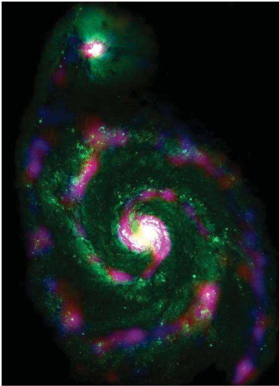
Figure 19. A composite image of the famous Whirlpool Galaxy with SCUBA-2 colours (blue for 450 \mu\text{m} ; red for 850) superimposed on a green-scale HST image. The SCUBA-2 traces star formation via the emission from cold dust in the outer most regions of galaxy. The SCUBA-2 image is provided courtesy of Todd MacKenzie, and the HST image is accredited to NASA, ESA, S. Beckwith (STScI) and the Hubble Heritage Team (STScI/AURA).
