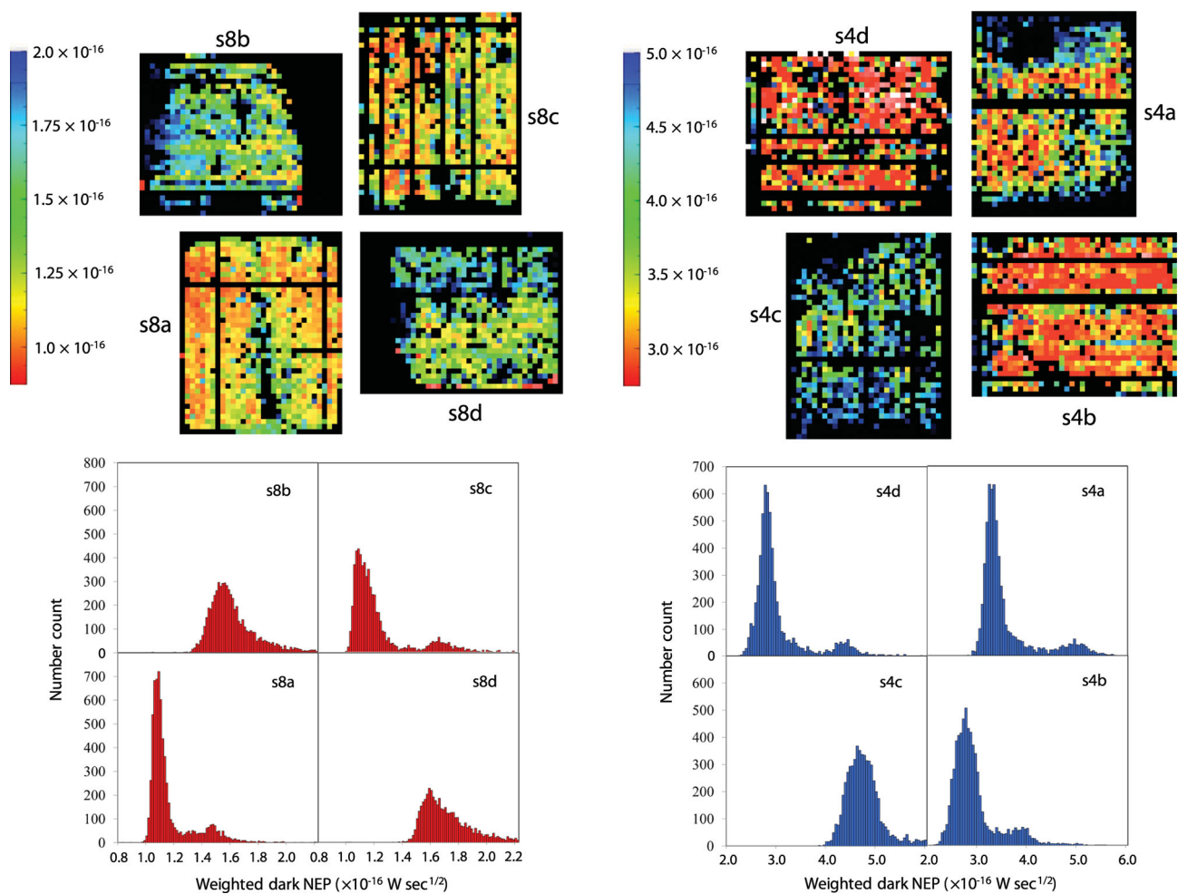
Figure 9. Top: typical dark NEP images recorded with the shutter closed for each of the SCUBA-2 sub-arrays. These are derived from a ‘dark noise’ measurements of \sim 10 s at the start of each observation. The colour scale on each image represents the NEP in units of W s^{1/2} . Bottom: dark NEP histograms for each sub-array, each on the same scale for ease of comparison.
