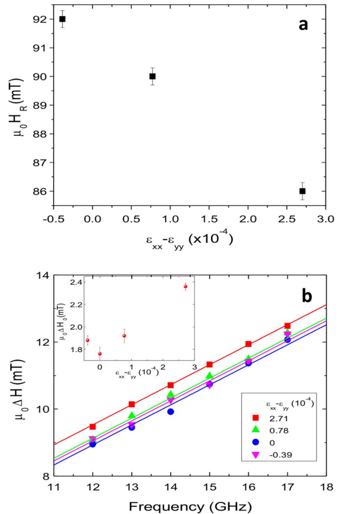
Figure 4 | Strain dependence of FMR resonance field and linewidth. (a) The resonance field ( \mu_0 H_R ) along the [100] axis as a function of the strain at an RF frequency of 15 GHz. (b) The FMR linewidth vs resonant frequency for different applied strain (points). Fits to the data using Eq. (6) are shown by solid lines. Inset: The intercept, \mu_0 \Delta H as a function of the applied strain.
