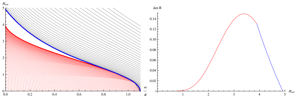
Figure 6. The panel on the left shows the possible values of H_{\text{ext}} and m . The red region corresponds to ball branes, while the grey region (above the the blue line) corresponds to Minkowski branes, which are all uniquely specified give the values (H_{\text{ext}}, m) . The curves are just an artifact of the discrete steps which were used to scan the full parameter space. The panel on the right shows the behaviour of the “mass gap” in the full parameter space as a function of the external magnetic field. The gap begins to develop as soon as H_{\text{ext}} > 0 and it closes again at H_{\text{ext}} = \hat{H}_2 \approx 5 .
