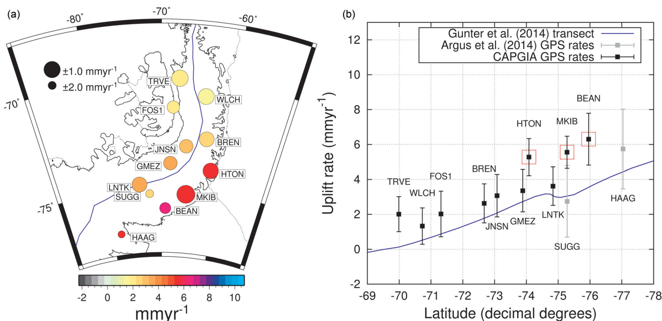
Figure 2. Vertical GPS rates after elastic deformation correction. (a) Map view. The symbol size is scaled by the inverse of the 1\sigma uncertainties of the vertical GPS rates. (b) Vertical rates by latitude with red squares highlighting the SE sites (see text for detail). The empirically-derived uplift rates of Gunter et al. (2014; solution CSR RL05 DDK5, corrected for 1.9 mm yr -1 GIA bias) are also shown, extracted along the blue transect line in panel (a).
