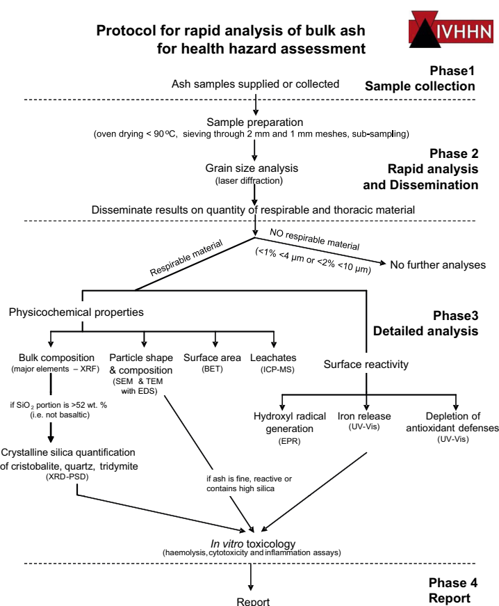
Fig. 1. Protocol used for rapid assessment of health hazard of volcanic ash, adapted from Le Blond et al. (2010) and Damby et al. (2013). The report on the initial analyses (end of Phase 2) was disseminated to local agencies at the end of May 2010 for Eyjafjallajökull ash, with the full report available from the International Volcanic Health Hazard Network website in September 2010.
