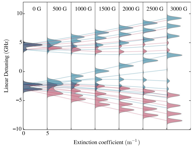
Fig. 4. (Colour online) The extinction coefficient as a function of linear detuning ( \Delta/2\pi ) for a ^{87}\text{Rb} vapour on the D_1 line (795 nm) and at a temperature of 20 °C. There are seven plots of the extinction coefficient at magnetic field values ranging from 0 to 3000 G in increments of 500 G. Each plot is placed on its side, displaced to the right for clarity, with the extinction coefficient ranging from 0 to 5 \text{m}^{-1} in each one. The area under each curve has been coloured either translucent red or blue, representing \sigma^- and \sigma^+ transitions. Overlaying the plots are curves showing the transition frequencies as a function of magnetic field. Notice that the strong \sigma^- transitions move to lower energies while the strong \sigma^+ ones move to higher energies. A video showing the evolution of the extinction coefficients for a Caesium vapour is available from http://www.jqc.org.uk/research/project/electsus/12683 .
