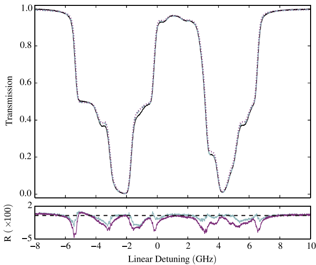
Fig. 6. (Colour online) Transmission as a function of linear detuning on the D 1 line (795 nm) for a 87 Rb cell (99.0% 87 Rb, 1.0% 85 Rb) with a length of 1 mm. The solid (black) curve shows the experimental data while the dashed (blue) and dotted (purple) curves show fits to the theory using the RR and ML fitting routines, rms deviations from the experimental data of 0.5% and 1% were found for the RR and ML fits respectively. The fit parameters were the magnetic field, cell temperature, and increased Lorentzian broadening due to buffer gases.
