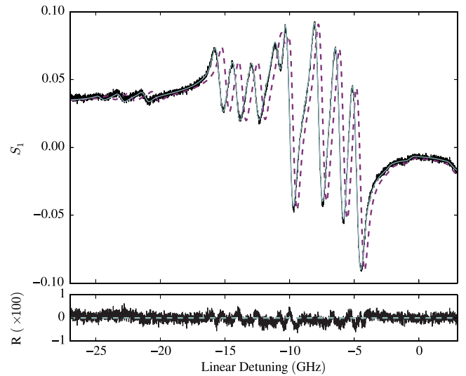
Fig. 7. (Colour online) S_1 Stokes parameter as a function of linear detuning on the D 2 line (780 nm) for a 87 Rb cell (99.0% 87 Rb, 1.0% 85 Rb) with a length of 1 mm. The solid (black) line is the experimental data while the solid (blue) and dashed (purple) lines are the fits to theory using the SA and ML techniques respectively. The ML fit is clearly poor; shown underneath are the residuals for the SA fit. The rms deviations of the ML and SA fits were 2.2% and 0.16% respectively.
