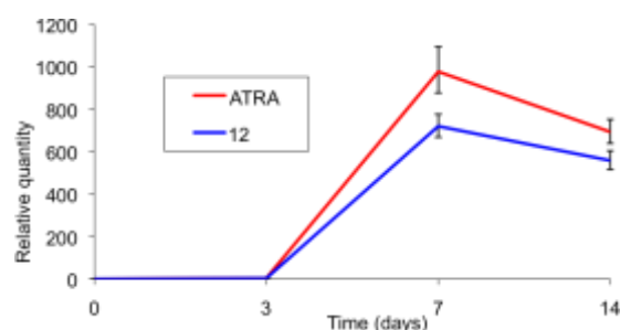
Fig. 6 RT-PCR analysis of the induction of TERA2.cl.SP12 cell differentiation in response to retinoids. Genes associated with
