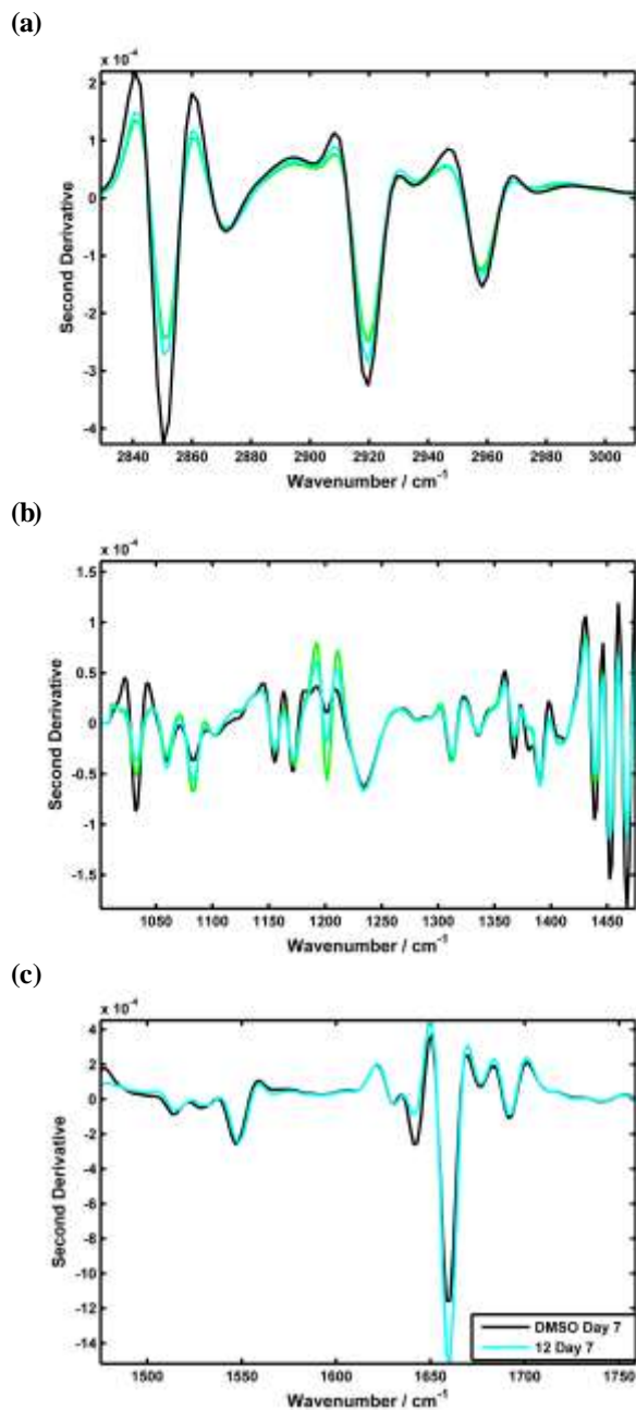
Fig. 9 Mean spectral comparisons of ATRA, 12 and DMSO treated TERA2.cl.SP12 cells: (a) Lipid spectral range (2830 – 3010 cm -1 ); (b) Fingerprint spectral range (1000 – 1475 cm -1 ) (c) Protein spectral range (1475 – 1760 cm -1 ).
