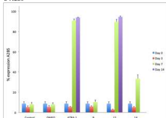
Fig. 5 Flow cytometric analysis of the induction of TERA2.cl.SP12 cell differentiation in response to retinoids. Markers of stem cells (SSEA-3 and TRA-1-60, A and B respectively) and neural differentiation (A2B5, C ) were differentially regulated during the 14 day culture period in response to 10 \mu M ATRA, 9 , 12 and 14 . Both ATRA and 12 (AH61) resulted in a rapid decrease in expression of the stem cell markers and reciprocal increase in neural marker expression after 14 days. Treatment with 9 and 14 did not induce differentiation; cells continued to proliferate and the experiment was terminated after 7 days as a results of being over-confluent. Data represent mean \pm SEM, n = 3.
