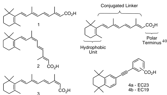
Fig. 1 Structures for ATRA 1 , 9CRA 2 , 13CRA 3 , generic retinoid structure, EC23 and EC19.
