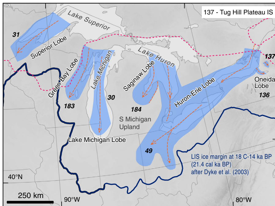
Fig. 11. Ice streams in the region of the Great Lakes (see Fig. 2 for location). Ice flow pattern of this ice sheet sector is described in Section 4.3 and more information about individual ice streams is available in Supplementary data. Boundary of the Canadian Shield is marked by a pink stippled line (medium grey if viewing a black and white version of the manuscript). (For interpretation of the references to colour in this figure legend, the reader is referred to the web version of this article.)
