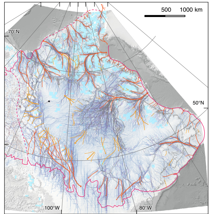
Fig. 17. A composite of meltwater drainage pathways (blue to purple thin lines [medium grey if viewing a black and white version of the manuscript]) derived from the calculation of the hydraulic potential surface at the ice-sheet bed for 293 modelled ice-surface geometries during the period of 32–6 ka BP (Livingstone et al., 2013; reproduced with permission) alongside reconstructed ice streams (Margold et al., 2015) drawn in orange/darker grey (LGM) and yellow/lighter grey (deglacial). Identified subglacial lake evidence in Christie Bay, Great Slave Lake (Christoffersen et al., 2008), is marked by a black star. Simplified LGM ice sheet margin is in pink (medium grey if viewing a black and white version of the manuscript). Note the correspondence between the modelled drainage locations and reconstructed ice stream tracks at times of maximum ice extent. However, ice streaming conditioned by the presence of meltwater cannot be directly inferred from this because topography plays a large role both in the modelled meltwater drainage pathways and in the location of ice streams. (For interpretation of the references to colour in this figure legend, the reader is referred to the web version of this article.)
