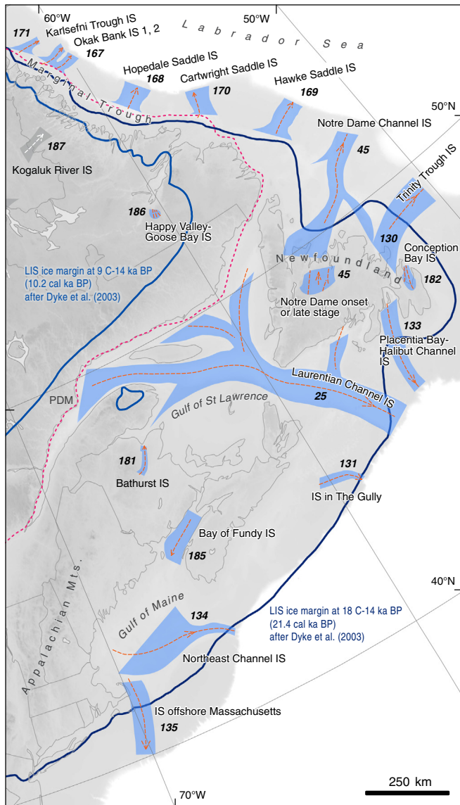
Fig. 12. Ice streams in the region of the Atlantic seaboard (see Fig. 2 for location). Ice flow pattern of this ice sheet sector is described in Section 4.4 and more information about individual ice streams is available in Supplementary data. Boundary of the Canadian Shield is marked by a pink stippled line (medium grey if viewing a black and white version of the manuscript). LIS extent is shown for the Last Glacial Maximum (LGM) and for 10.2 cal ka BP after Dyke et al. (2003), but note that a greater LGM extent has recently been inferred for the continental shelf (Shaw et al., 2006). PDM – Pointe-des-Monts (see Table 1). (For interpretation of the references to colour in this figure legend, the reader is referred to the web version of this article.)
