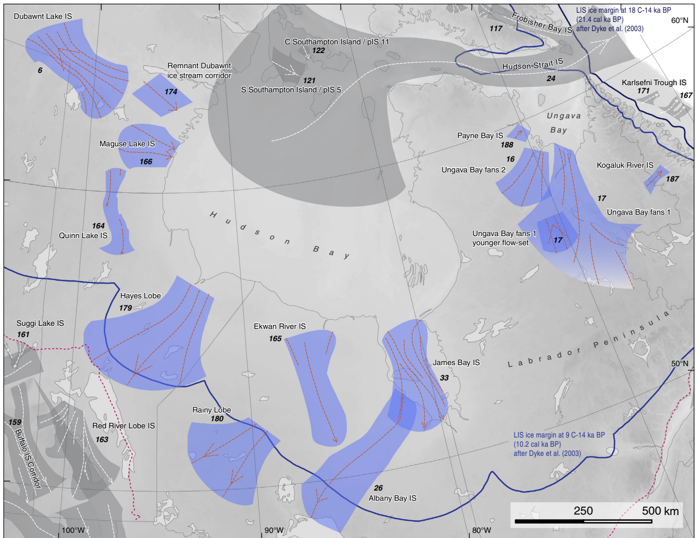
Fig. 13. Ice streams in the region of the Canadian Shield (see Fig. 2 for location). Ice flow pattern of this ice sheet sector is described in Section 4.5 and more information about individual ice streams is available in Supplementary data. Boundary of the Canadian Shield is marked by a pink stippled line (medium grey if viewing a black and white version of the manuscript). (For interpretation of the references to colour in this figure legend, the reader is referred to the web version of this article.)
