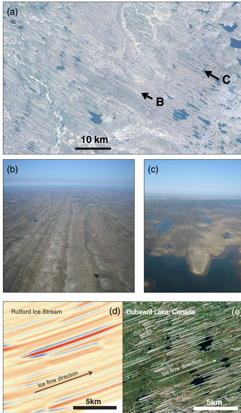
Fig. 5. Highly elongated mega-scale glacial lineations (MSGL) on the bed of the Dubawnt Lake Ice Stream. (a) Landsat imagery (path 039, row 015) of a portion of a central trunk of the ice stream, (b and c) oblique aerial photographs of parts of the image in panel (a); photographs: C. R. Stokes, panels (a)–(c) reprinted from Stokes et al. (2013) with authors' permission. (d) MSGL identified on the bed of the Rutford Ice Stream in Antarctica (see Fig. 1 for location) compared to MSGL on the bed of the Dubawnt Lake Ice Stream (e); panels (d)–(e) reprinted from King et al. (2009) with authors' permission.
