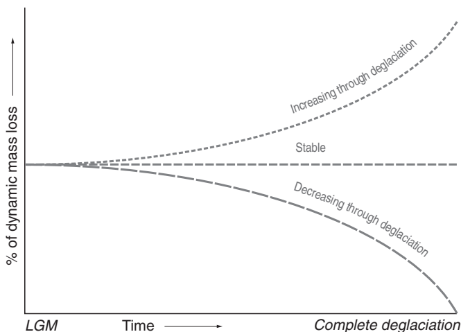
Fig. 19. Conceptual scenarios for the percentage of dynamic mass loss in the Laurentide Ice Sheet during deglaciation. Three possible scenarios are drawn: (1) the percentage of mass loss delivered by ice streams remained stable; (2) the percentage of mass loss delivered by ice streams decreased during deglaciation, with a proportionally increasing contribution from surface melt, (3) the percentage of mass loss through ice streams increased during deglaciation, perhaps hinting at non-linear feedbacks accelerating mass loss beyond that which might be expected from climate forcing alone.
