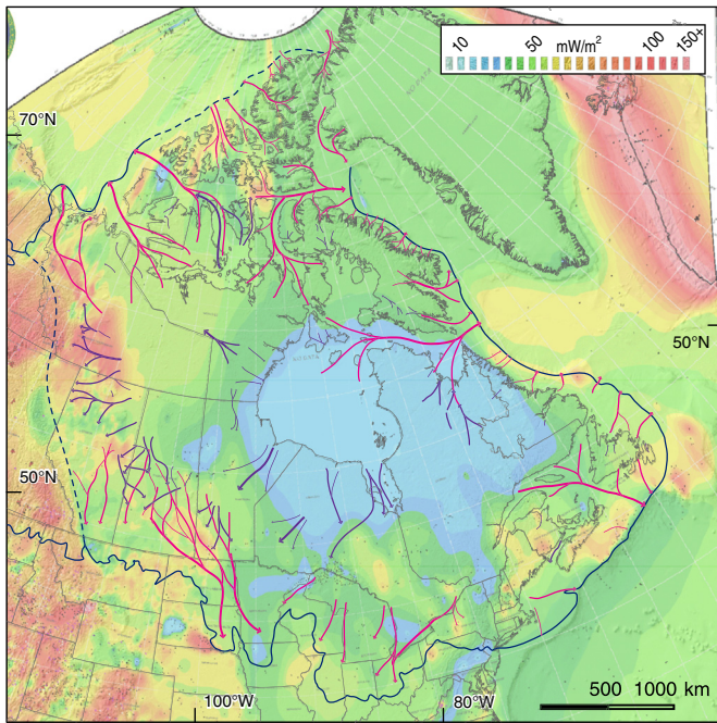
Fig. 18. Present-day geothermal heat flux for the area formerly covered by the Laurentide Ice Sheet (modified from Blackwell and Richards, 2004). Simplified Last Glacial Maximum extent is drawn after Shaw et al. (2006), Kleman et al. (2010), and Jakobsson et al. (2014). Ice streams are drawn by arrows; those inferred to be active at the Last Glacial Maximum are in pink; deglacial ice streams or those with unknown age are in purple (lighter and darker grey, respectively, if viewing a black and white version of the manuscript). (For interpretation of the references to colour in this figure legend, the reader is referred to the web version of this article.)
