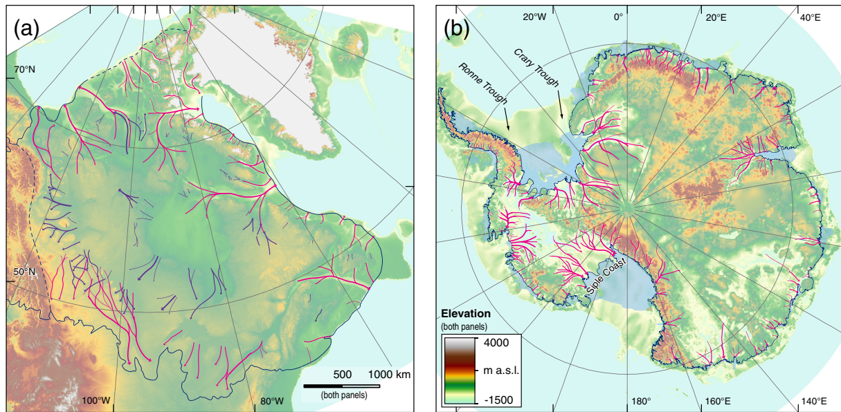
Fig. 14. Topography of ice sheet beds. (a) Present-day (isostatically uplifted) topography of the area covered by the Laurentide Ice Sheet. Simplified Last Glacial Maximum extent is drawn after Shaw et al. (2006), Kleman et al. (2010), Jakobsson et al. (2014). Ice streams are drawn by arrows; those inferred to be active at the Last Glacial Maximum are in pink; deglacial ice streams or those with unknown age are in purple (lighter and darker grey, respectively, if viewing a black and white version of the manuscript). Present day glaciation is marked in white. (b) Subglacial topography of Antarctica (data from Fretwell et al., 2013); ice streams are drawn in pink, ice shelves in transparent blue (shades of grey if viewing a black and white version of the manuscript). Troughs on the continental shelf mentioned in the text are marked. Both panels are drawn to the same scale and use the same hypsometric colour scale. (For interpretation of the references to colour in this figure legend, the reader is referred to the web version of this article.)
