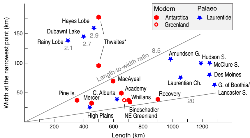
Fig. 16. Length-to-width ratio of large ice streams in present-day Antarctic and Greenland ice sheets and in the Laurentide Ice Sheet. *The Thwaites Glacier is shown twice because it appears to have an inner and outer lateral margin on both sides (see text in Section 5.2).
