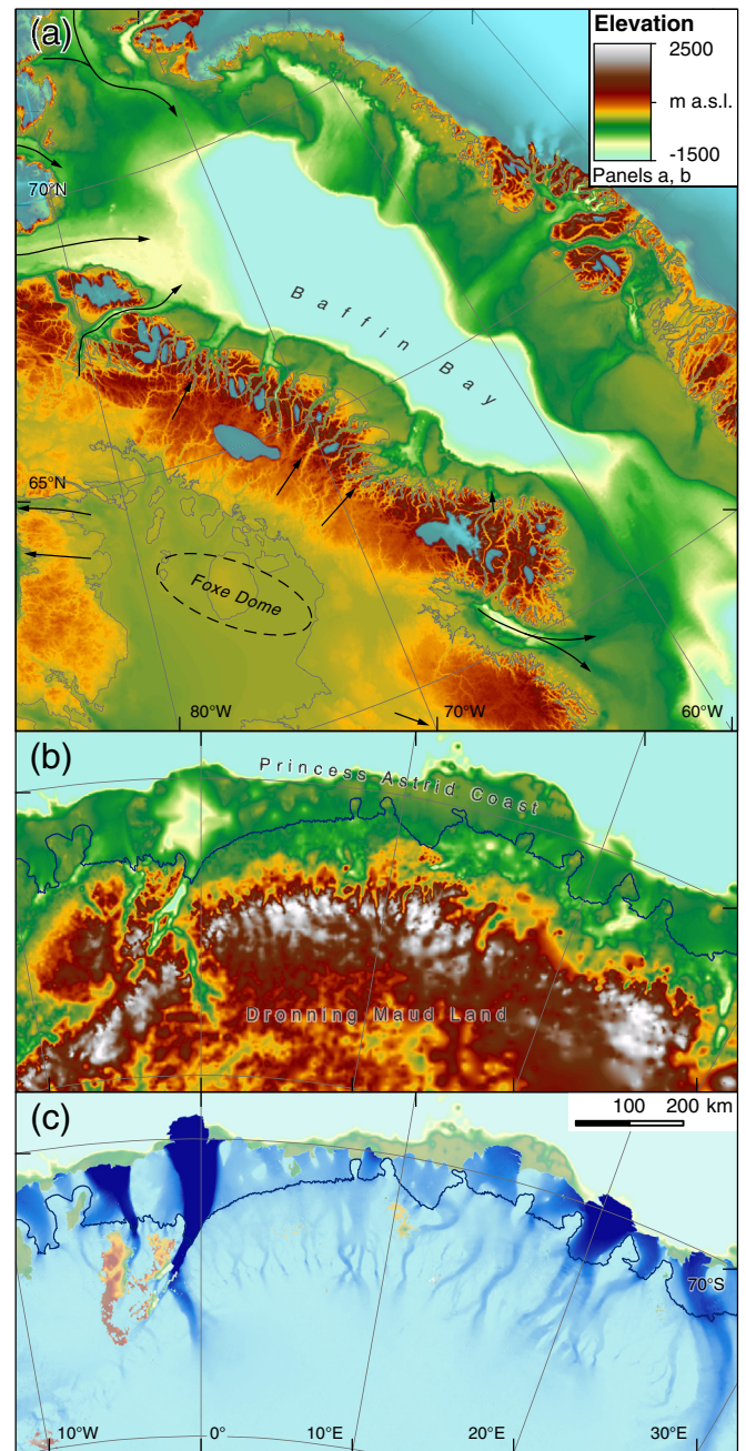
Fig. 7. High-relief coasts modified by selective linear erosion under ice sheet glaciation. (a) Topographic map of Foxe Basin, Baffin Island and Baffin Bay (IBCAO data from Jakobsson et al., 2000; location marked in Fig. 3). Glacial troughs on the continental shelf NE of the Baffin Island coast were incised by ice draining from the Foxe Dome across Baffin Island; ice-flow directions are shown by black arrows. Note the difference in the size and spacing of glacial troughs and sediment bulges along the Baffin and Greenland sides of Baffin Bay, which hints at some form of spatial self-organisation, i.e., many narrow and closely-spaced ice streams versus fewer, broader ice streams spaced further apart. Present-day glaciation is marked in a semi-transparent blue (grey if viewing a black and white version of the manuscript). (b) Subglacial topography of Dronning Maud Land and the Princess Astrid Coast in East Antarctica. Bedmap2 data from Fretwell et al. (2013) are significantly less detailed than the data used in panel a; location is marked in Fig. 1. (c) Ice-flow pattern for the area shown in panel b (data from Rignot et al., 2011c) – note the topographic steering of the major ice streams. All panels are drawn to the same scale and with the same hypsometric colour scale. (For interpretation of the references to colour in this figure legend, the reader is referred to the web version of this article.)
