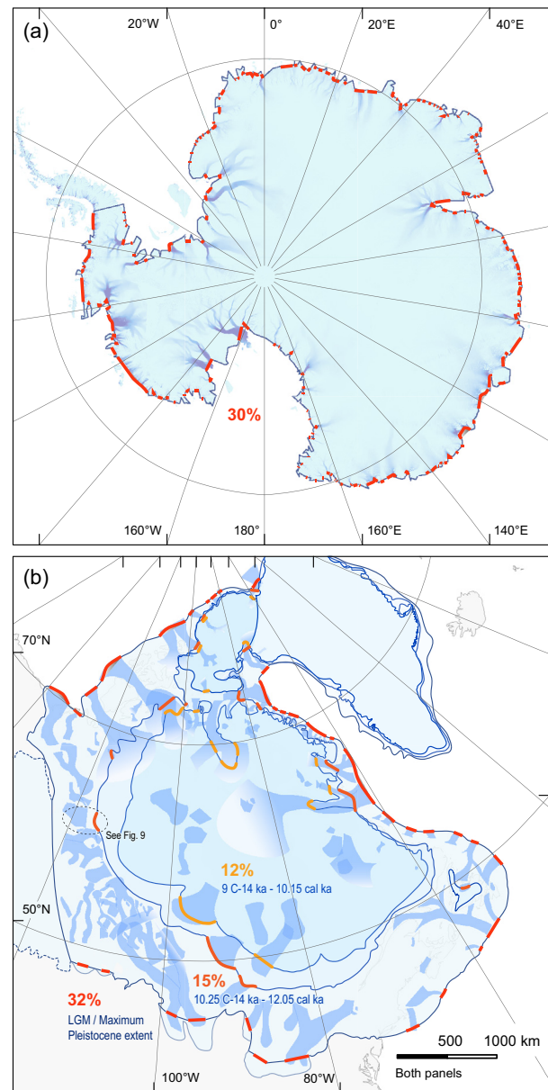
Fig. 20. Percentage of the streaming margin calculated for Antarctica (a) and the Laurentide Ice Sheet (b), using the definition of an ice stream as spatial partitioning of ice flow (see Section 3). Streaming margin was mapped manually for Antarctica from data by Rignot et al. (2011c) and ice streams reconstructed by Margold et al. (2015) were used for the Laurentide Ice Sheet. The Laurentide ice margin is straightened for the inclusion of the large lobes formed by terrestrially terminating ice streams. Note that the coarseness of the method used implies that the results can be used as a first estimate only.
