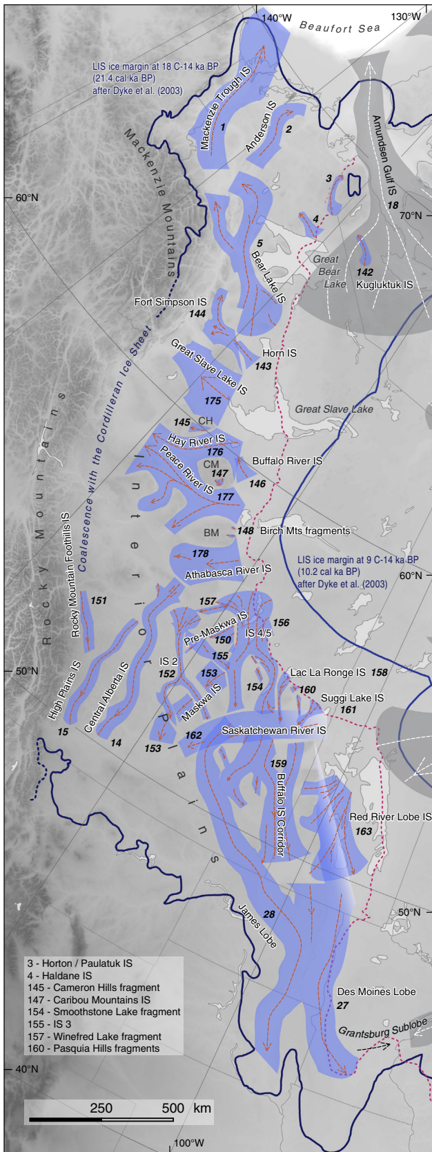
Fig. 9. Ice streams in the region of the Interior Plains (see Fig. 2 for location). Ice flow pattern of this ice sheet sector is described in Section 4.2 and more information about individual ice streams is available in Supplementary data. Boundary of the Canadian Shield is marked by a pink stippled line (medium grey if viewing a black and white version of the manuscript). Abbreviations: CH – Cameron Hills, CM – Caribou Mountains, BM – Birch Mountains. (For interpretation of the references to colour in this figure legend, the reader is referred to the web version of this article.)
