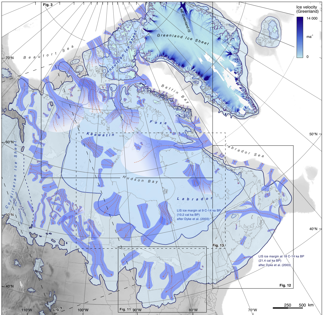
Fig. 2. Ice streams of the Laurentide Ice Sheet (LIS) drawn after Margold et al. (2015). LIS extent is shown for the Last Glacial Maximum (LGM) and at 10.2 ka BP, from Dyke et al. (2003). Note that the LIS has recently been shown to extend to the continental shelf at the LGM in many regions (e.g., Briner et al., 2006; Shaw et al., 2006; Kleman et al., 2010; Lakeman and England, 2012, 2013; Jakobsson et al., 2014; Nixon and England, 2014). The locations of Figs. 3, 9, 12, 11, and 13 are marked by black rectangles. Present-day glaciation is in light turquoise with ice margins in thin purple line (light grey with a dark grey margin if viewing a black and white version of the manuscript). Ice flow velocity for the Greenland Ice Sheet is reproduced from the data released by Joughin et al. (2010a); data coverage is not complete; missing data is shown in white. Present-day coastline and administrative boundaries are drawn in grey (applies also for subsequent figures). This figure is drawn to the same scale as Fig. 1. (For interpretation of the references to colour in this figure legend, the reader is referred to the web version of this article.)
