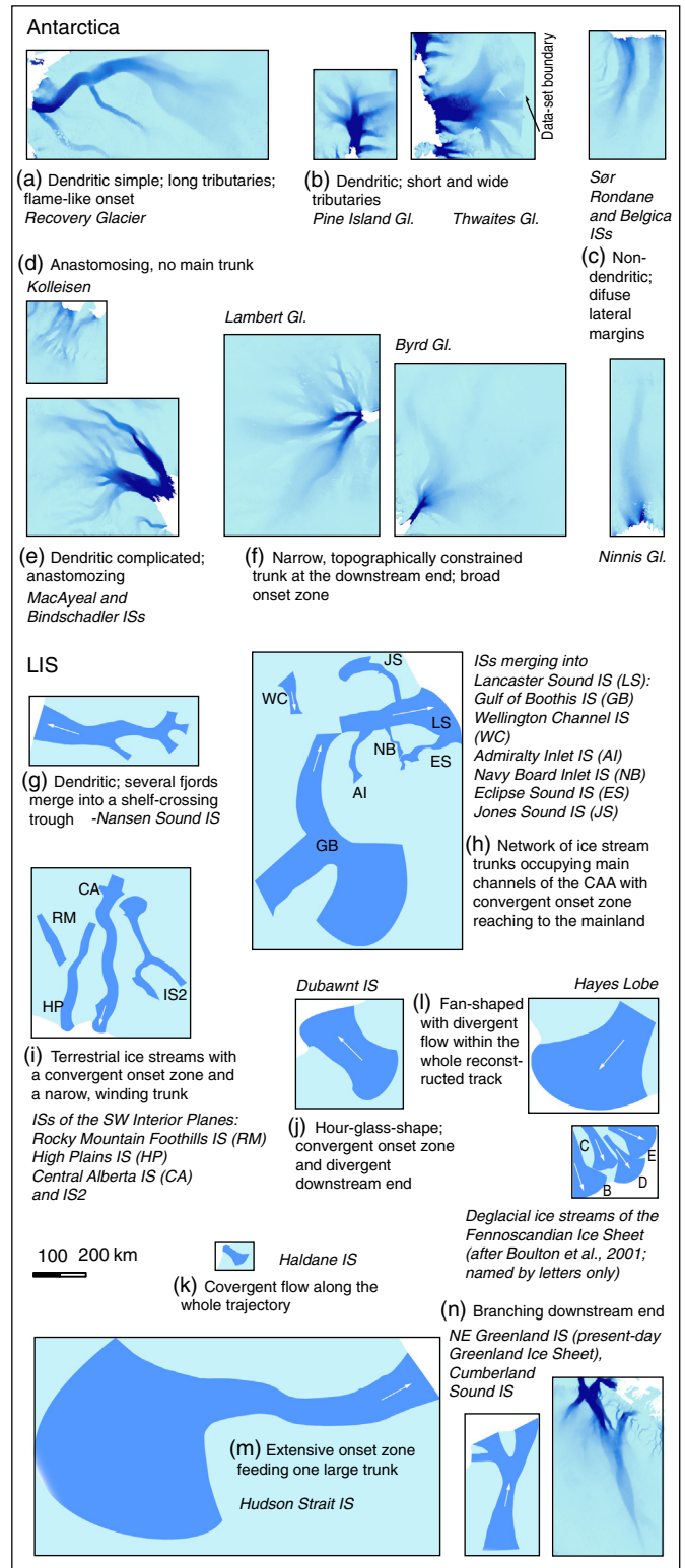
Fig. 15. Shapes of ice streams. Shapes of present-day Antarctic and Greenlandic ice streams (all data from Rignot et al., 2011c; panel (n) reproduced from data by Joughin et al., 2010a) compared to Laurentide palaeo-ice streams (Margold et al., 2015). Different ice stream shapes discussed in the text are drawn, all to the same scale. See Figs. 1, 2, 3, 9, 13 for locations. Similarities occur between modern ice streams in Antarctica and ice streams of the Laurentide Ice Sheet: branching and anastomosing patterns are present in both groups. Hour-glass-shaped and fan-shaped ice streams (panels (j) and (l)) are absent among modern ice streams, but occurred in the Fennoscandian Ice Sheet during deglaciation (redrawn from Boulton et al., 2001).
