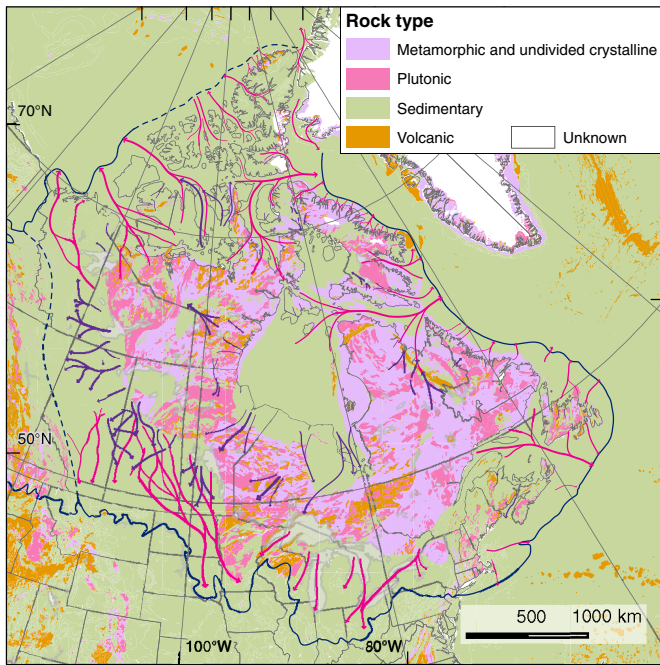
Fig. 8. Rock types on the Laurentide Ice Sheet bed. Ice streams are drawn by arrows; those inferred to be active at the Last Glacial Maximum are in pink; deglacial ice streams or those with unknown age are in purple (lighter and darker grey, respectively, if viewing a black and white version of the manuscript). Note the increased occurrence of ice streams beyond the edge of the Canadian Shield (regions in north-central Canada built of crystalline rocks). (For interpretation of the references to colour in this figure legend, the reader is referred to the web version of this article.)
