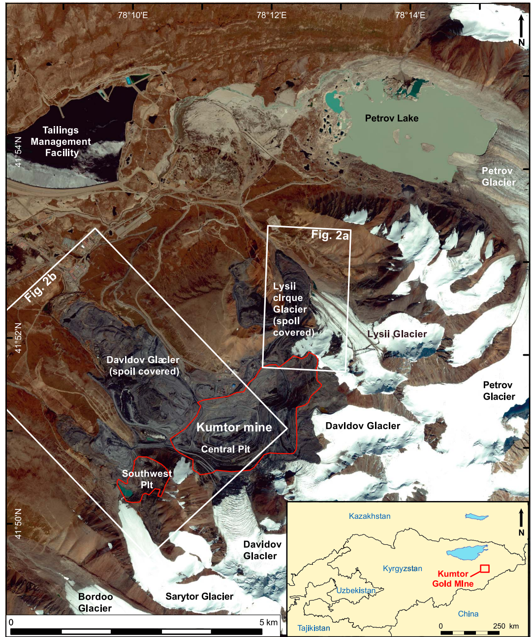
Figure 1. Location map of the Kumtor mine and the glaciers surrounding it in 2014. The background satellite data is a 0.5 m pan-sharpened image from Digital Globe’s WorldView-2 platform. The inset shows the mine location in Kyrgyzstan.
