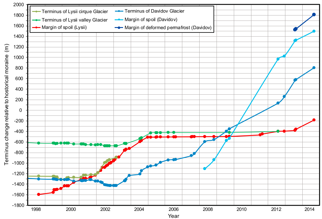
Figure 4. Glacier terminus and spoil margin position for the Lysii cirque Glacier, Lysii valley Glacier, and Davidov Glacier. Dots represent the time of measurement using both high-resolution satellite imagery and available Landsat and Aster imagery where high-resolution data were not available. Positions are measured relative to the fronts of the most prominent historical moraines in the Davidov or Lysii Valleys.
