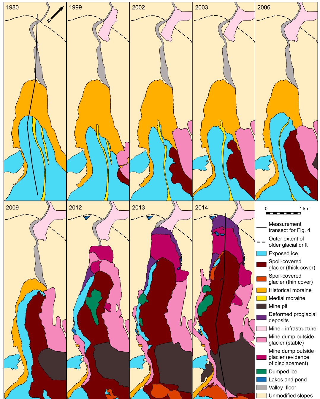
Figure 7. Time series of landcover classification for Davidov Glacier from 1980 to 2014. Additional images are used in the analysis of terminus position (Table 1 and Figures 4 and 6).
