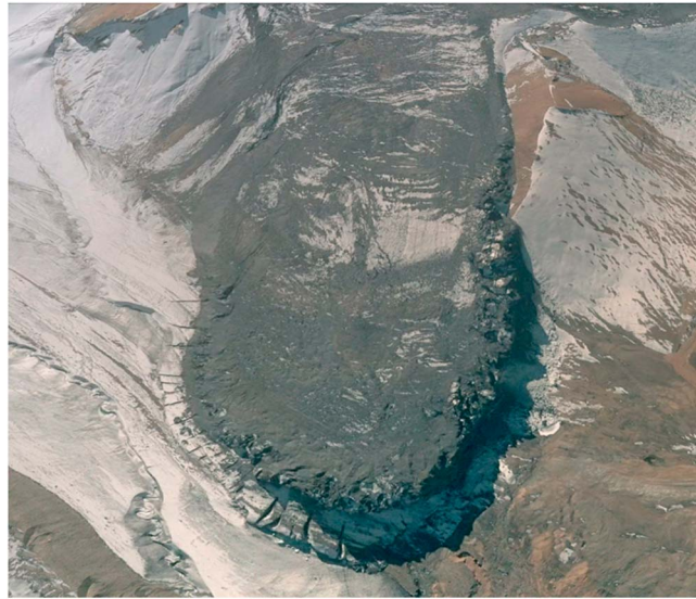
Figure 5. Oblique 2.4 m resolution Quickbird image of the Lysii cirque Glacier front in 2002 during the initial advance of the dual lobate surge front. The stacked debris-poor and spoil covered lobes and their radial crevasses are clearly visible at this time. For scale, the lobe is 300–350 m wide.
