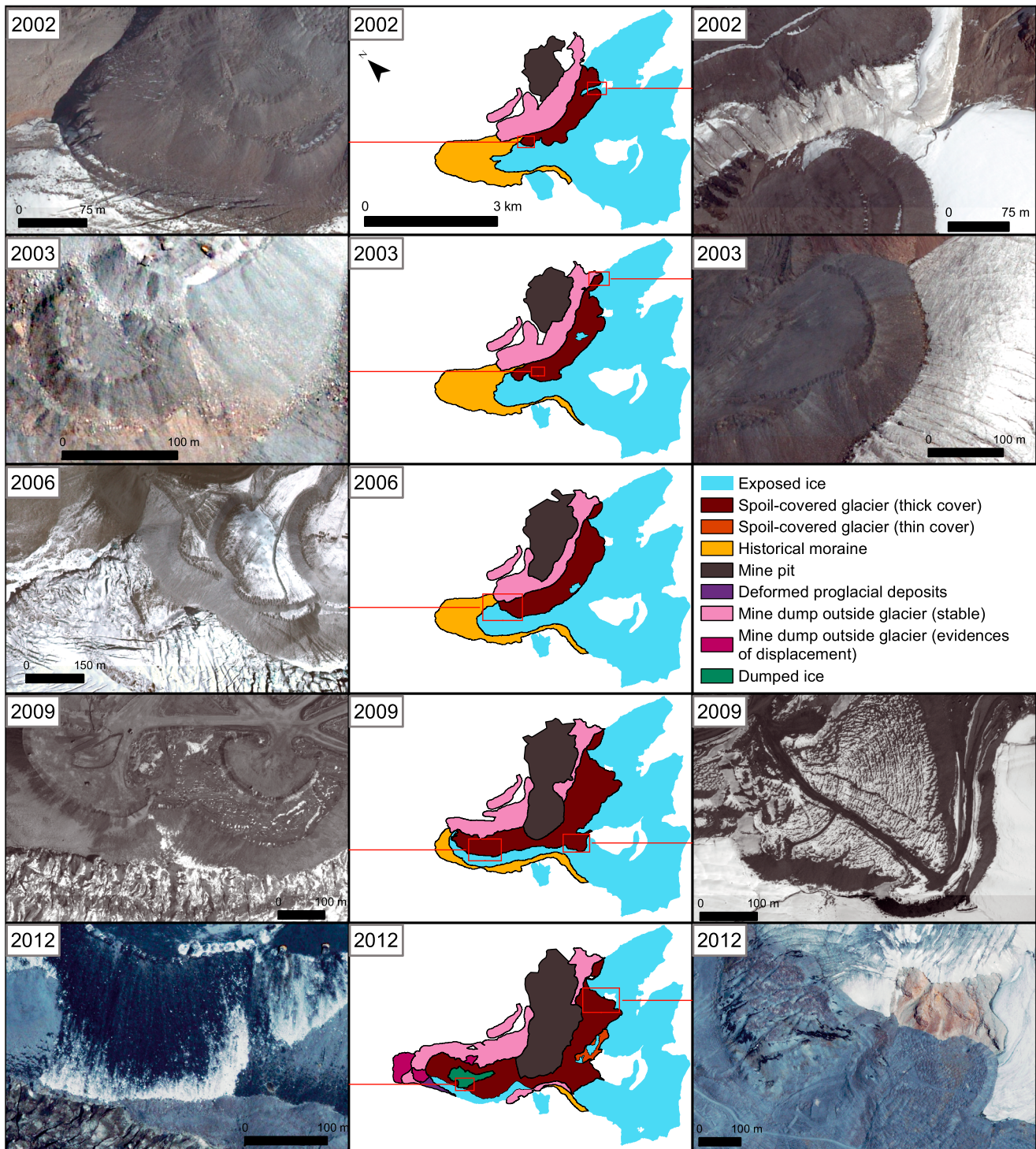
Figure 8. Time series of thin, thick, and laterally dumped spoil distributions in the Davidov Valley. The central panels show the distributions, and the left and right images demonstrate how spoil rests on the glacier in a range of areas. These show that thick spoil is being dumped both at the side and on top of the glacier. The bottom left image from 2012 demonstrates dumping of glacier ice from the trucks.
