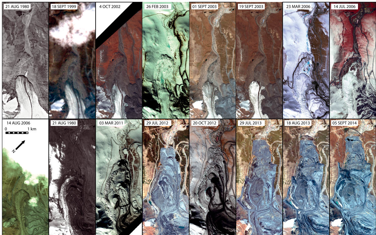
Figure 6. Time series of satellite imagery for Davidov Glacier showing the change in terminus position and the extent of the spoil dumps and mine pit.
