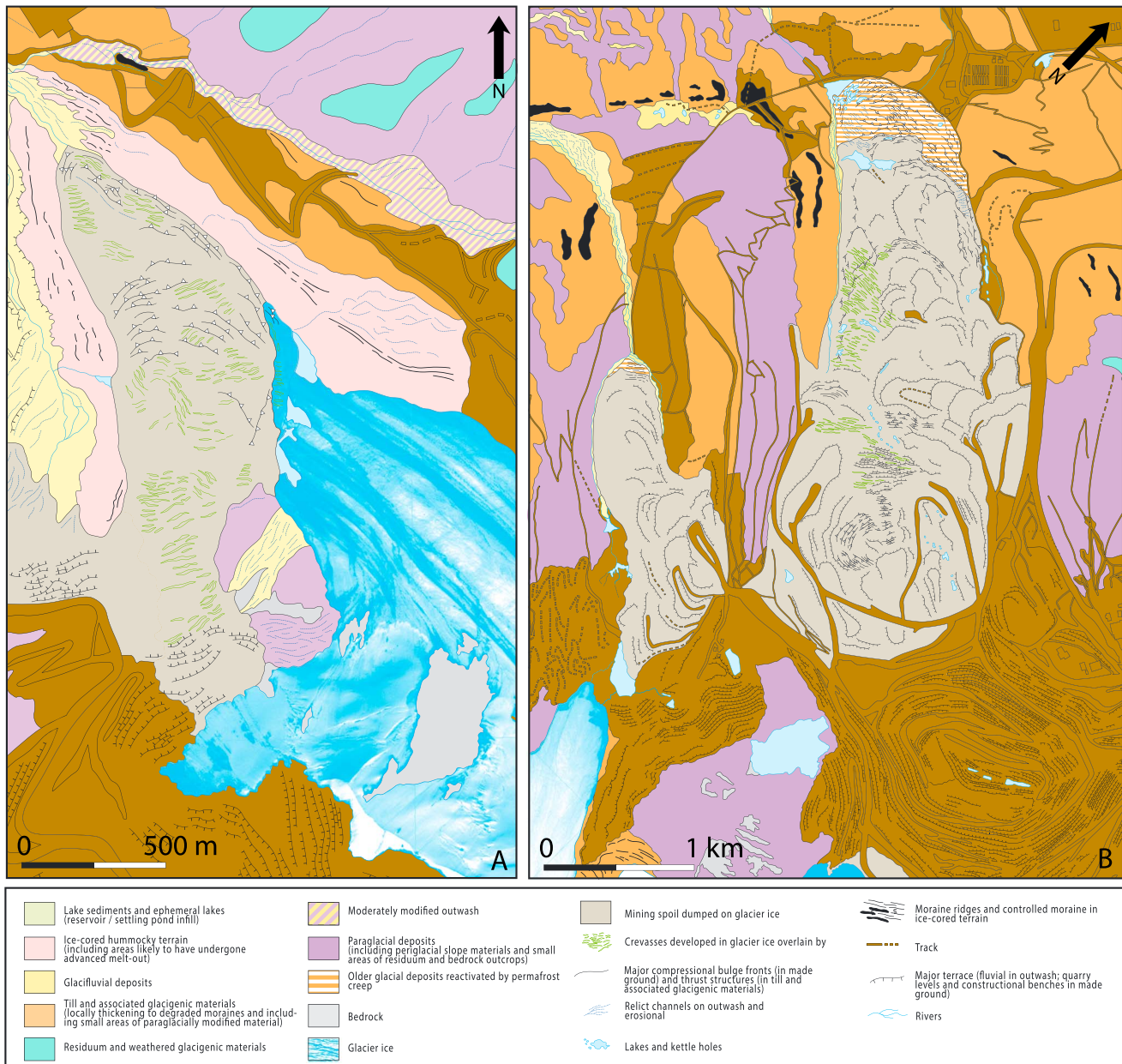
Figure 2. The surficial geology and geomorphology map of the (a) Lysii cirque and (b) Davidov Glaciers and their forelands. The map was compiled from a 0.5 m pan-sharpened image from Digital Globe’s WorldView-2 platform dating to the 5th of September 2014.
