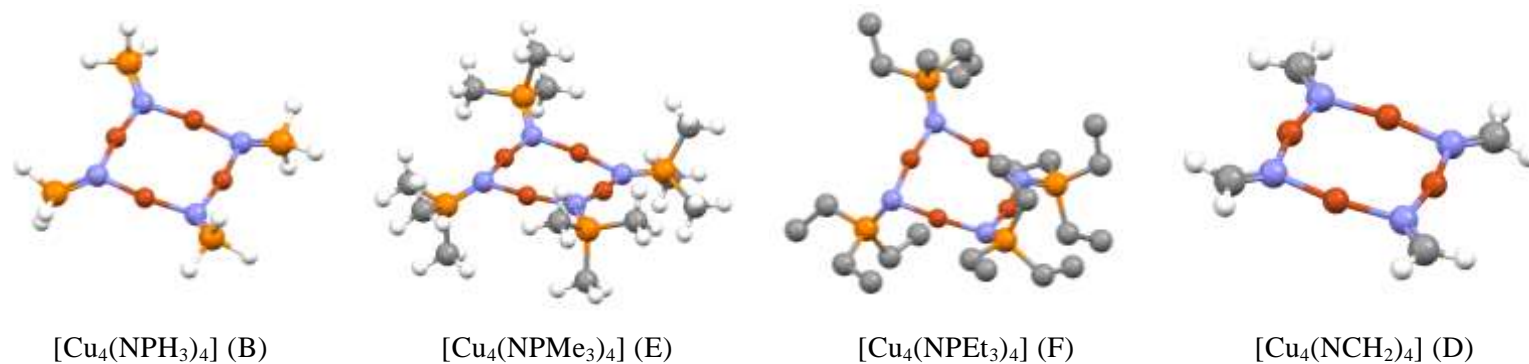
Figure 7. Diagrams showing the optimised molecular geometries of selected complexes containing 3-coordinate nitrogen ligands in {Cu 4 N 4 } clusters. In the case of [Cu 4 (NPEt 3 ) 4 ] hydrogen atoms have been omitted for clarity.
