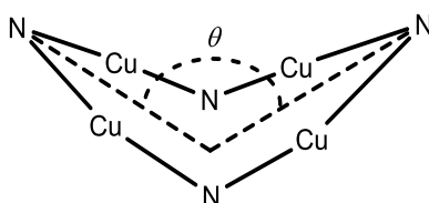
Figure 5. One saddle angle ( \theta ) shown of two possible within the \{\text{Cu}_4\text{N}_4\} ring.
