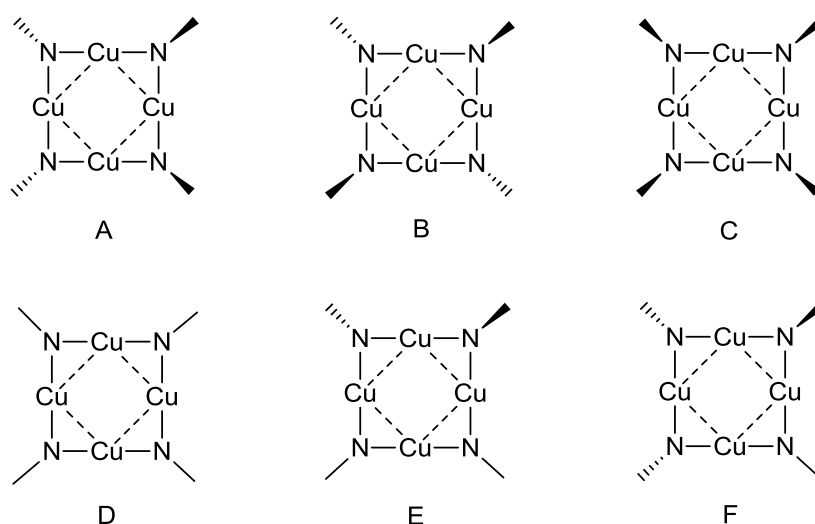
Figure 4. Conformers for \{\text{Cu}_4\text{N}_4\} complexes with N atoms in pyramidal and/or planar coordinations
