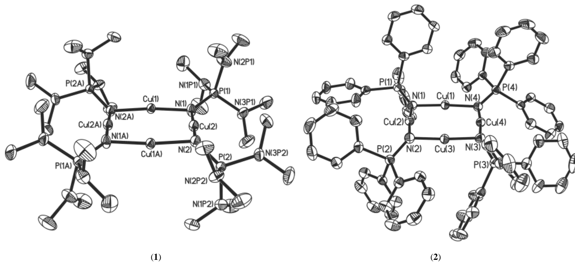
Figure 2. Molecular structures of the complexes 1 and 2 (50% probability ellipsoids). Hydrogen atoms in 1 and 2 have been omitted for clarity. Symmetry transformations used to generate equivalent atoms in 1 : -X, -Y+1, -Z+1 .
