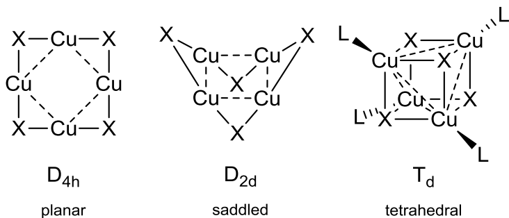
Figure 3. Geometries for Cu 4 X 4 and Cu 4 X 4 L 4 clusters
