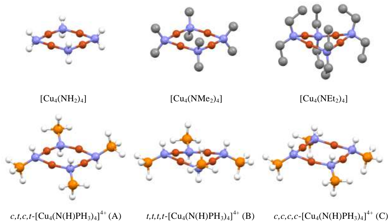
Figure 6. Diagrams showing the optimised molecular geometries of selected complexes containing 4-coordinate nitrogen ligands in \{\text{Cu}_4\text{N}_4\} clusters. In the case of [\text{Cu}_4(\text{NMe}_2)_4] and [\text{Cu}_4(\text{NEt}_2)_4] hydrogen atoms have been omitted for clarity.
