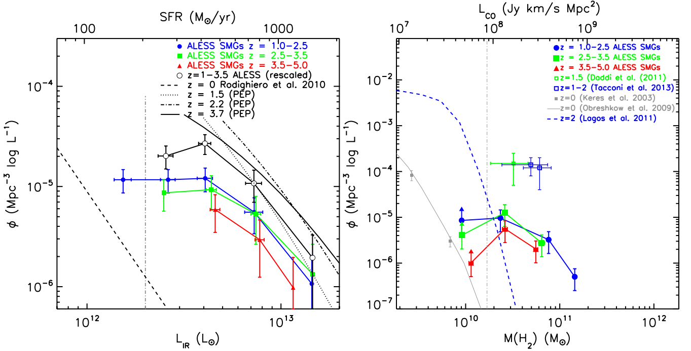
Figure 8. Left: the far-IR luminosity function for ALESS SMGs split into three bins of photometric redshift. In this plot, the error bars are derived by bootstrap resampling for uncertainties in the luminosities and photometric redshifts. Since the ECDFS has been shown to be underdense in bright sub-mm sources (Weiß et al. 2009), to match the 870 \mu\text{m} number counts in other extragalactic survey fields, we also re-scaled the z = 1.5-3.5 luminosity function by a factor 2\times (black solid line). The vertical dot-dashed line shows the approximate ALESS completeness limit. We also show the z = 0 luminosity function from Rodighiero et al. (2010) as well as the z \sim 1.5, 2.2 and 3.7 IR luminosity function of 100 \mu\text{m} and 160 \mu\text{m} selected galaxies from the PEP survey from Gruppioni et al. (2013) which are well matched to the (rescaled) ALESS SMGs. Right: the \text{H}_2 mass function for SMGs compared to local data and theoretical models. In this plot, we have adopted a gas-to-dust ratio of appropriate for each galaxy given its SFR and stellar mass, and applied the correction factor for the underdensity of bright sub-mm sources in ECDFS. We compare the results for the ALESS SMGs with z = 0 which shows that at a fixed gas mass (or equivalently, \text{CO}(1-0) line luminosity) there are \sim 100\times more galaxies at z = 2 than z = 0 . We also include on the plot the space density of ‘main-sequence’ starburst galaxies (BzKs and BX/BMs) from Daddi et al. (2010) and Tacconi et al. (2012). The dashed line shows the predicted z = 2 gas mass function from Lagos et al. (2011).
