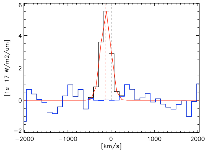
Figure 1. The FIR [\text{C II}]\lambda 157 \mu\text{m} line obtained from the central spaxel ( 9.4 \times 9.4 \text{ arcsec}^2 ) of the Herschel PACS rebinned data cube. The mean line centroid is blueshifted with respect to M87 (at z = 0.004360 ) by v = -123 \pm 5 \text{ km s}^{-1} . The blue line indicates the detector noise.
