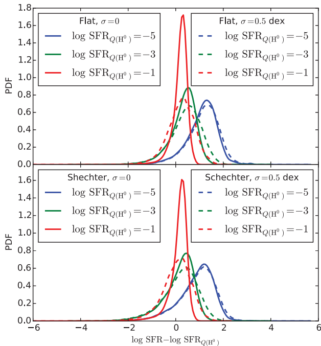
Figure 11. Posterior probability distributions for the logarithmic SFR based on measurements of the ionizing flux, computed with SFR_SLUG . The quantity plotted on the x -axis is the offset between the true log SFR and the value that would be predicted by the ‘point mass’ estimate where one ignores stochastic effects and simply uses the naive conversion factor between ionizing luminosity and SFR. Thus a value centred around zero indicates that the point mass estimate returns a reasonable prediction for the most likely SFR, while a value offset from zero indicates a systematic error in the point mass estimate. In the top panel, solid curves show the posterior PDF for a flat prior probability distribution and no photometric errors ( \sigma = 0 ), with the three colours corresponding to point mass estimates of \log \text{SFR}_{Q(\text{H}^0)} = -5 , -3 , and -1 based on the ionizing flux. The dashed lines show the same central values, but with assumed errors of \sigma = 0.5 dex in the measured ionizing flux. In the bottom panel, we show the same quantities, but computed using a Schechter function prior distribution rather than a flat one (see main text for details).
