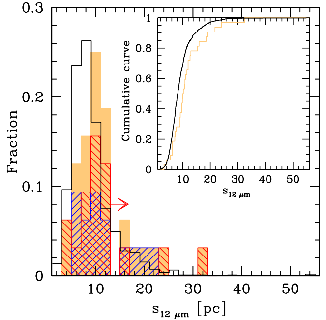
Figure 7. Distribution of the sizes (in parsec) of the 12 \mu\text{m} emitter for our sample (orange filled histogram) and for the control sample of typical QSOs (black open histogram). The two histograms are normalized to the total number of sources in the two samples. The red hatched histogram is the s_{12 \mu\text{m}} distribution of our sample with E(B - V)_{\text{qso}} \geq 0.1 (18 objects), while the blue hatched histogram is for our sample with E(B - V)_{\text{qso}} < 0.1 (14 objects).
