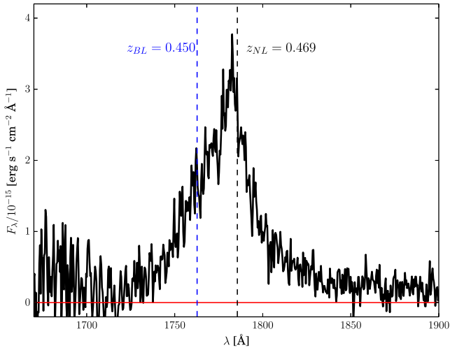
Figure 3. HST /COS ultraviolet spectrum of J1154+0134 displaying Ly \alpha emission. The red solid line denotes the zero level, while the two vertical dashed lines mark the broad-line (blue) and narrow-line (black) redshift.
