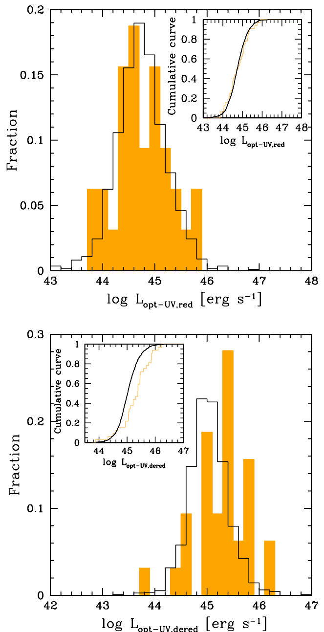
Figure 5. Disc luminosity distribution for our sample (orange filled histogram) and for the control sample of typical QSOs (black open histogram). The two histograms are normalized to the total number of sources in the two samples. The internal panels show the cumulative distributions for our sample (orange line) the control sample (black line). Top panel: Best-fitting disc luminosity before applying the reddening correction (host galaxy contamination removed). Bottom panel: Best-fitting disc luminosity after applying the reddening correction (host galaxy contamination removed).
