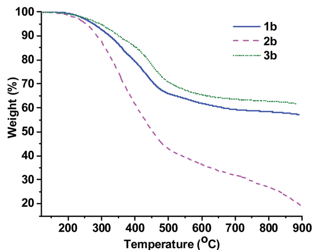
Fig. 2 TGA data of 1b (blue line), 2b (magenta dashed line) and 3b (green dotted line). Data were recorded in flowing He ( 20\text{ mL min}^{-1} ) at a ramp rate of 10\text{ °C min}^{-1} to 900 °C after being held at 120 °C for 30 min to remove any residual solvent.
