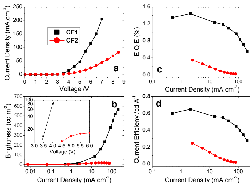
Figure 3. Plots of (a) J - V curves. (b) Luminance vs. J . (c) EQE vs. J . (d) Device Efficiency vs. J for the polymers CF1 and CF2 . Inset to (b) shows the low turn-on voltages for the two devices in a plot of luminance vs. V . The device structure is stated in Table 2, footnote a .
