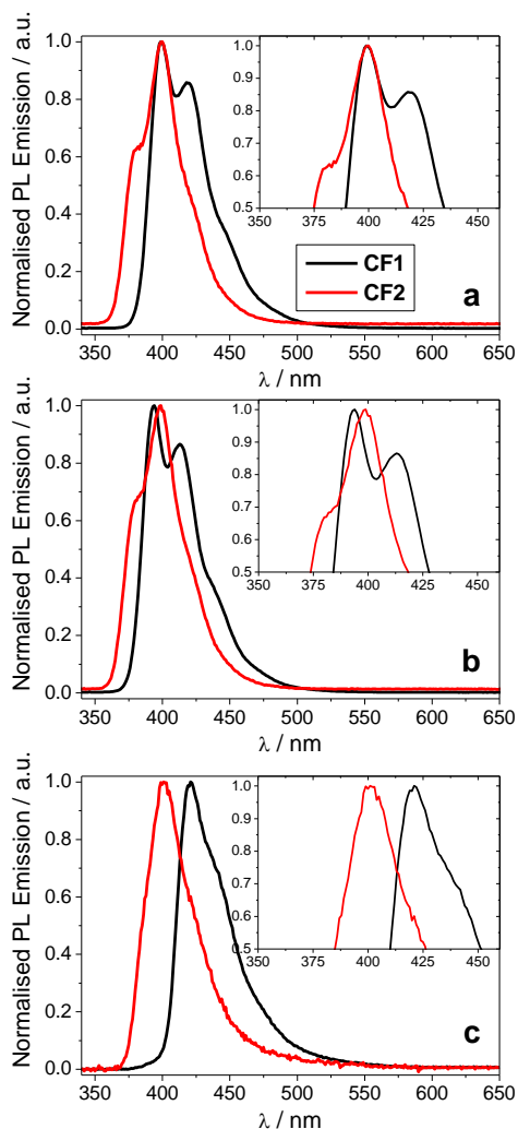
Fig. 2: Normalised PL emission spectra for polymers CF1 and CF2 (a) in ethyl acetate; (b) in cyclohexane; (c) in thin film. The insets show a magnification of the \lambda_{\text{max}} region.
