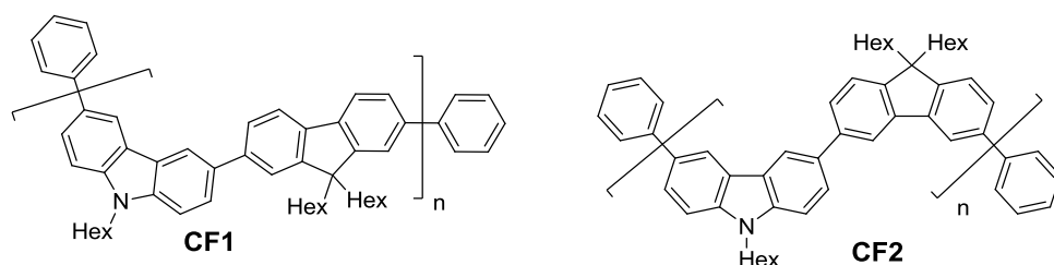
Fig. 1 Structures of the new deep blue / violet emitting carbazole- alt -fluorene copolymers studied in this work.
