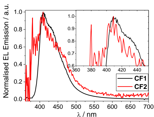
Figure 4. Normalised EL emission spectra for polymers CF1 and CF2 devices. Inset shows a magnification of the \lambda_{\text{max}} region. The device structure is stated in Table 2, footnote a .
