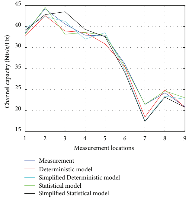
FIGURE 14: Channel capacity in downlink.
