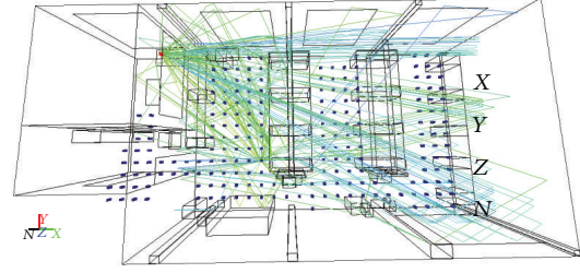
FIGURE 3: Ray-launching in an indoor environment.
