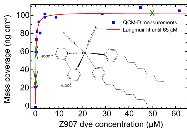
Figure 2. QCM-D area mass uptake over concentration of sensitizing dye solution with a Langmuir isotherm fitted to the data. Blue data points are taken from previously published experiments 27 . Green crosses mark the three concentrations of dye solutions used for staining the AFM samples and indicate their corresponding mass coverage. The insert shows the structure of the Z907 ruthenium dye.
