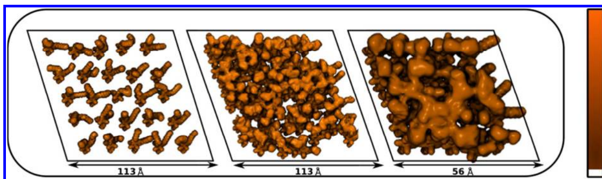
Figure 6 . The simulated AFM pictures for different mass coverage (33%, 66%, and 100% from left to right, respectively). Map of the weighted atomic density of dye molecules. The map is done by replacing each dye atom with a normalized Gaussian distribution of width (standard deviation) equal to the atomic radius. The Gaussian distribution for each atom is then weighted with the occupancy. The various Gaussians are added and distributed on a grid (orange color). The isosurface value is 0.01. The same map with restriction to the parts of dye molecules that are 13-25 Å away from the TiO 2 surface is shown in the supporting information Figure S7.
