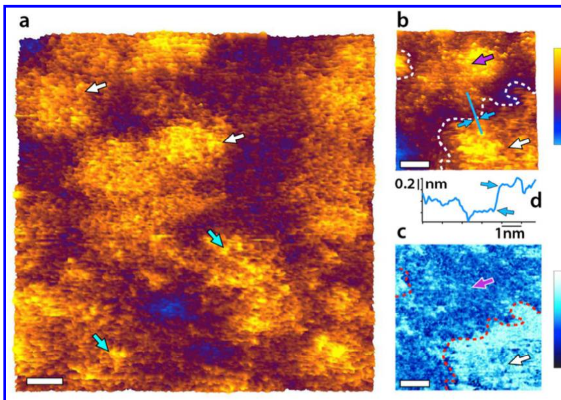
Figure 3. AFM micrographs of a \text{TiO}_2 surface covered with Z907 ruthenium dye (30 % mass coverage). (a) A low magnification (100 nm) topographic image shows almost uniform coverage by the dye apart for a few higher dye domains (blue arrows). The \sim 20 nm wide protrusions (white arrows) are related to the substrate roughness. Higher resolution topographic (b) and phase (c) images of the surface reveal a sponge-like structure of the dye layer (white arrow). The substrate can also be exposed by scratching with the AFM tip (b-c) revealing a \sim 0.6 nm dye layer thickness. The exposed \text{TiO}_2 substrate (purple arrow) exhibit a clear phase contrast (dotted red line) with the lighter Z907 domains. A topographic profile (d) taken over the \text{TiO}_2 -Z907 border (blue line in b) indicates a thickness of \sim 0.4 nm for the Z907 dye layer. The topographic images are always represented with an orange-blue color scale and the phase images in blue-black throughout the paper. The scale bars are 10 nm (a) and 3 nm (b, c). The colour bars are 3 nm (a, b) and 15^\circ (c).
