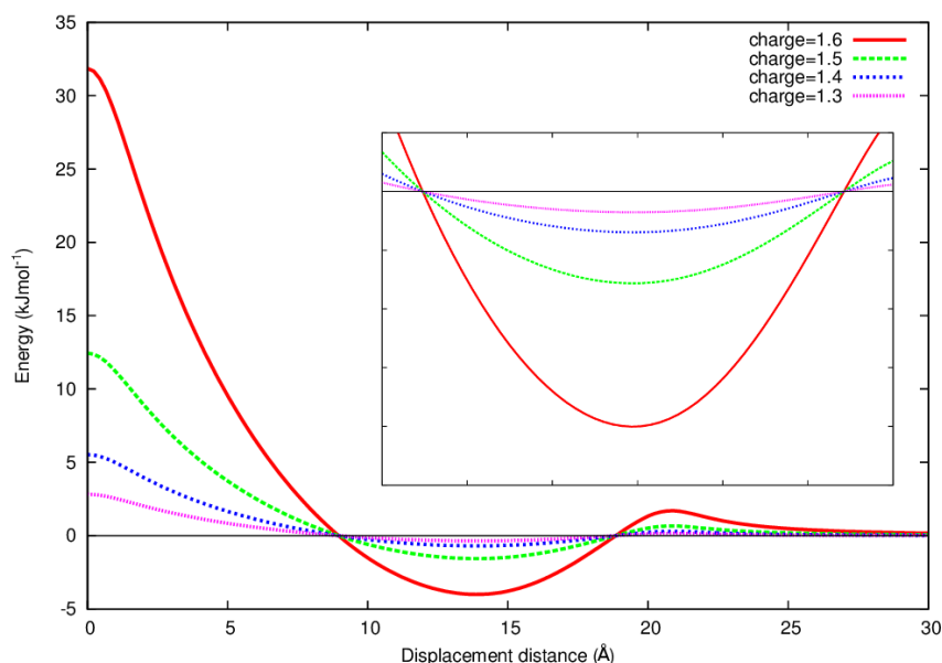
Figure 5. Graph showing the dependence of potential on the magnitude of the charge on the core (and counter charge on the corona) for z = 3.6 \text{ \AA} . The inset shows an expanded section of the potential between the two roots. The charge refers to the excess electron present in the core ( 1e \equiv 1.602 \times 10^{-19} \text{ C} ).
