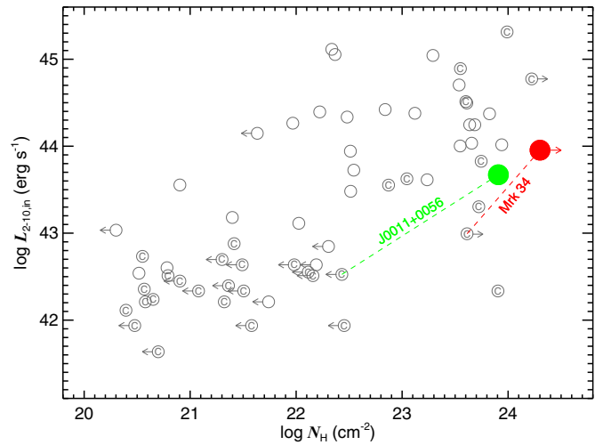
Figure 6. N_H vs. L_{2-10, \text{in}} for all X-ray-detected SDSS QSO2s (gray), based only on direct continuum modeling of X-ray data below 10 keV, collated from Vignali et al. (2006, 2010), Jia et al. (2013), and LaMassa et al. (2014). N_H upper limits are denoted by arrows and CT candidates are denoted with “C.” Recall that CT candidacy is often based on indirect multiwavelength indicators, and direct continuum fitting to low-energy X-ray data of faint, obscured AGNs is very inefficient at securely identifying CT sources. This is why many CT candidates have apparent N_H \ll 10^{24} \text{ cm}^{-2} at present, and their plotted values of L_{2-10, \text{in}} are also likely to be underestimates. The large filled points are the updated values from NuSTAR modeling for the two NuSTAR -detected sources (Mrk 34 in red and SDSS J0011+0056 in green, respectively, where the latter is reported in Lansbury et al. 2014).
