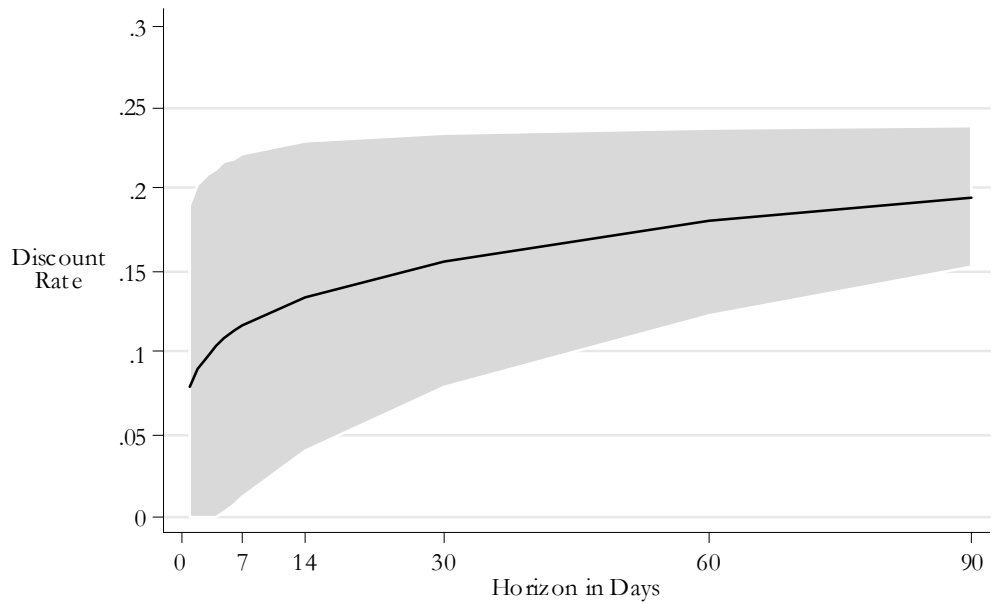
Figure F2: Weibull Discount Rates from Mixture Model Point estimate and 95% confidence interval
