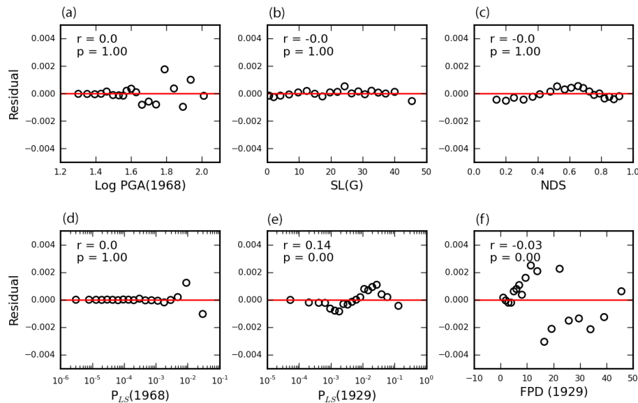
Figure 13. Distributions of P_{LS} residuals for the 1968 earthquake, hindcast using Eq. (6). Panels (a)–(c) show the residuals for this model (observed P_{LS} minus predicted P_{LS} ) plotted against each of the model predictors. Panel (d) shows the model residuals plotted against the predicted P_{LS} . Panels (e) and (f) show the model residuals plotted against predicted P_{LS} for the 1929 earthquake and distance from the 1929 coseismic fault, respectively. All residuals are calculated by aggregating probabilities across 20 equal quantile bins of the x variable. Positive residuals indicate that the model under-predicts P_{LS} and negative residuals indicate that the model over-predicts P_{LS} . Note that the amplitude of the plotted residuals varies due to binning and aggregating probabilities with the different predictor variables. For each plot, the coefficient ( r ) and significance ( p ) of correlation in the residuals are given. These were derived by adding each x variable into a logistic regression analysis of P_{LS} predicted using Eq. (6) and observed landsliding. In this respect we test the coupled significance of SL and G as they feature in the model.
