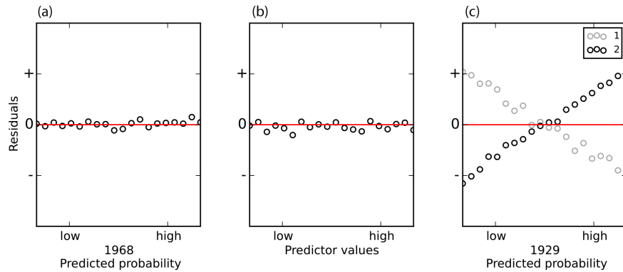
Figure 9. Hypothetical output of hillslope failure conditional probability analysis for the 1929 and 1968 earthquakes. This illustrates how the model residuals (observed P_{LS} minus predicted P_{LS} ) would be distributed if conditional probability models, which account for the full subset of spatial, time-independent factors (i.e. those not associated with previous events) influencing landslide occurrence, have been fitted and used to hindcast P_{LS} . (a) 1968 model residuals are uncorrelated with predicted P_{LS} . (b) Model residuals are uncorrelated with values of individual model predictors. (c) Model residuals are correlated with P_{LS} hindcast for the 1929 earthquake either negatively (model 1) – indicating preconditioning of hillslopes against failure – or positively (model 2) – indicating preconditioning of hillslopes for failure. The residuals are calculated by aggregating probabilities across equal quantile bins of the x variable. Note that positive and negative residuals are relative to the prediction of a model that does not explicitly consider the effect of hillslope preconditioning but is fitted using landslide data that are subject to the effect of hillslope preconditioning. Therefore it is the direction of the trend, rather than the absolute (positive or negative) residual values, that is of importance in the test of preconditioning.
