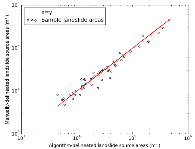
Figure B2. Comparison of manually and algorithm-delineated source areas, for a sample of 51 landslides. Manually and automatically delineated areas fall near the 1 : 1 line, showing that this technique can provide an accurate approximation of the landslide source area.
