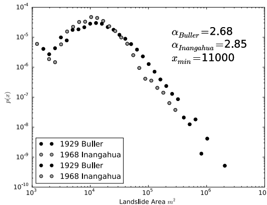
Figure 8. Probability densities of landslide areas as a function of landslide area for the 1929 Buller and 1968 Inangahua earthquake landslide inventories. Power-law scaling exponents ( \alpha ) have been derived using the method of Clauset et al. (2009), for areas > 11\,000\text{ m}^2 .
