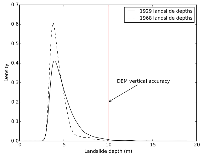
Figure D1. Distribution of landslide depths for the 1929 and 1968 earthquakes, estimated using global best-fit relationship between landslide area and volume (Larsen et al., 2010). Vertical accuracy of elevation data is indicated in red.
