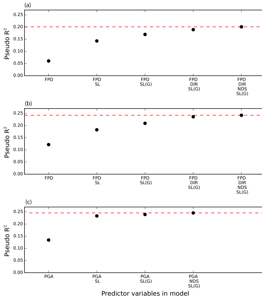
Figure 12. Relative contributions of predictor variables to the fit of the 1929 and 1968 hillslope failure probability models. Sequence of model input predictors and resulting pseudo- R^2 goodness of fit values, produced by sequentially removing the least contributing predictor variable. (a) Results from Eq. (5) for the 1929 earthquake, (b) results from Eq. (5) for the 1968 earthquake, and (c) results from Eq. (6) for the 1968 earthquake.
