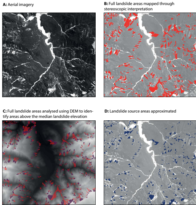
Figure B1. Illustration of landslide source area extraction technique for a 10 \times 10 km sample area, showing landslides triggered by the 1929 Buller earthquake.
