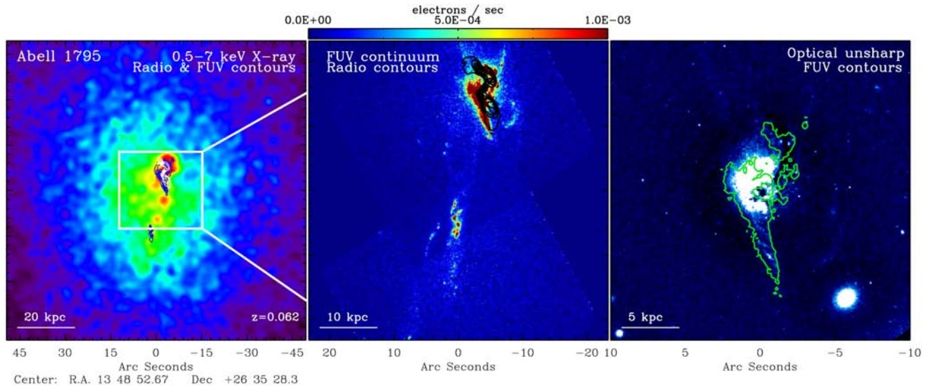
Figure A4. The Abell 1795 BCG ( z = 0.0625 ). The X-ray, FUV continuum, and broad-band optical unsharp mask images are shown in the left-hand, centre, and right-hand panels, respectively. FUV contours are overlaid in blue and green on the X-ray and optical panels, respectively. The radio source is shown in white and black contours on the X-ray and FUV panels, respectively. Note the remarkable spatial correspondence between the FUV continuum emission and the radio source. The FUV colour bar can be scaled to a flux density by the inverse sensitivity 2.173 \times 10^{-17} \text{ erg cm}^{-2} \text{ \AA}^{-1} \text{ electron}^{-1} . The centroids of all panels are aligned, with east left and north up.
