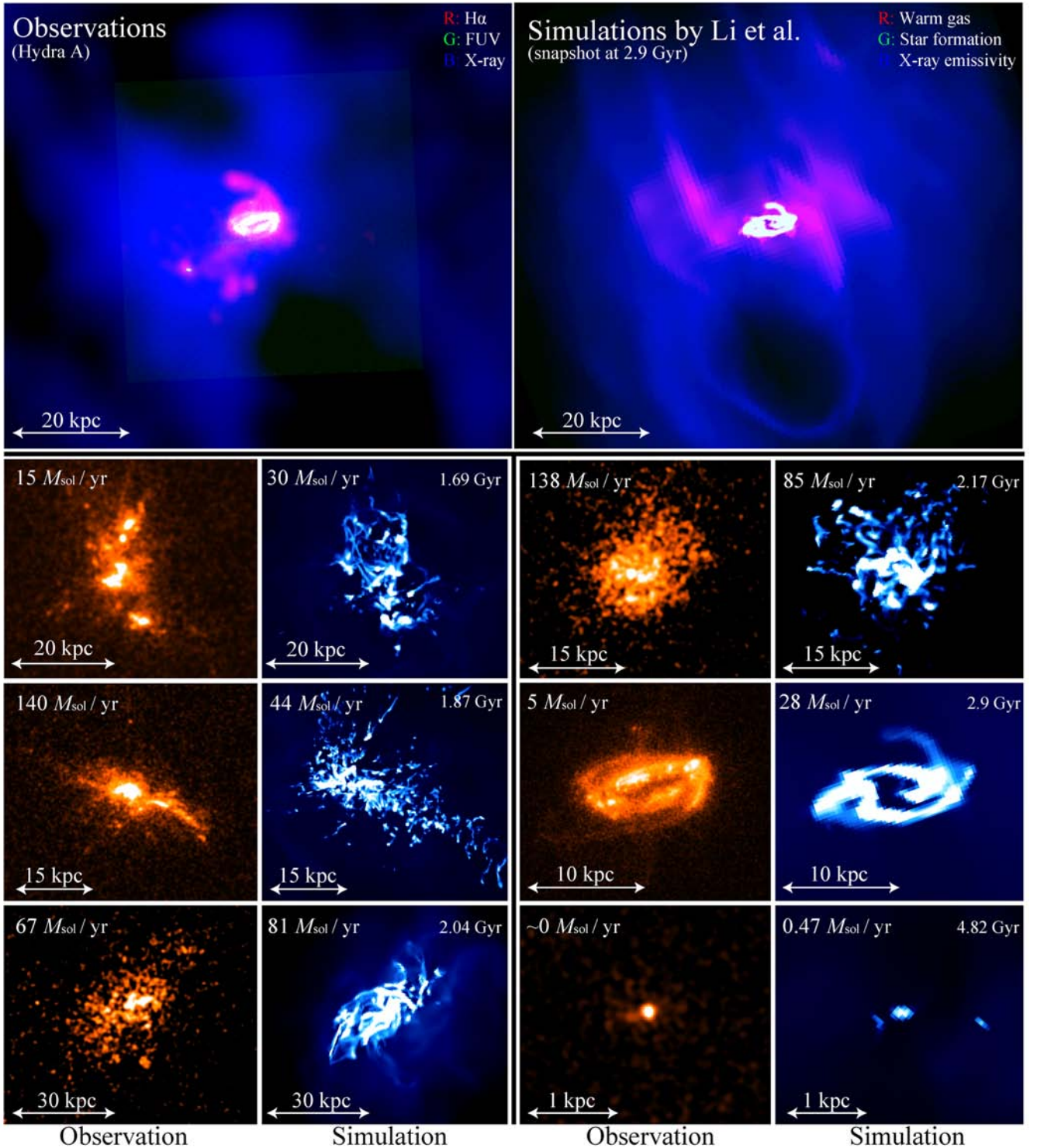
Figure 14. Observations compared with simulations by Y. Li and collaborators (e.g. Li & Bryan 2014a,b; Li et al. 2015). Top panels: a multiwavelength (X-ray, FUV, and \text{H}\alpha ) composite of Hydra A, compared with a single snapshot of the Li et al. (2015) simulation at 2.9 Gyr. The RGB channels are set to roughly simulate \text{H}\alpha , FUV, and X-ray emissivities, respectively, though two ‘cheats’ have been used: the green channel shows cold, dense gas where star formation appears in the simulation – the assumption, then, is that FUV emission from these young stars would roughly show the same morphology. The red channel does not explicitly show simulated \text{H}\alpha , but rather intermediate temperature gas whose morphology closely matches a rough scaling to simulate collisionally ionized (but not photoionized) \text{H}\alpha . It should therefore be treated as a very rough approximation. Bottom panels: selected FUV images from our sample are shown in orange, and projected density-weighted density snapshots from the simulation are shown in blue. The bright knots and filaments show the high-density low-temperature clouds that are forming stars in the simulation (see Li et al. 2015 for details). Our sample’s redshift range spans \sim 3 Gyr of cosmic history. The simulation is capable of producing star-forming structures similar in axial ratio, physical extent, and star formation rate within the same \sim 3 Gyr temporal slice of the simulated cluster’s evolution.
