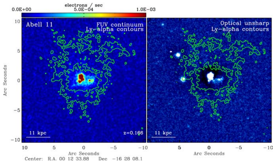
Figure A1. The Abell 11 BCG ( z = 0.1660 ). The FUV continuum image and broad-band optical unsharp mask are shown in the left- and right-hand panels, respectively. Ly \alpha contours are overlaid in green. The radio source is unresolved. The FUV colour bar can be scaled to a flux density by the inverse sensitivity 4.392 \times 10^{-17} \text{ erg cm}^{-2} \text{ \AA}^{-1} \text{ electron}^{-1} . The centroids of both panels are aligned, with east left and north up.
