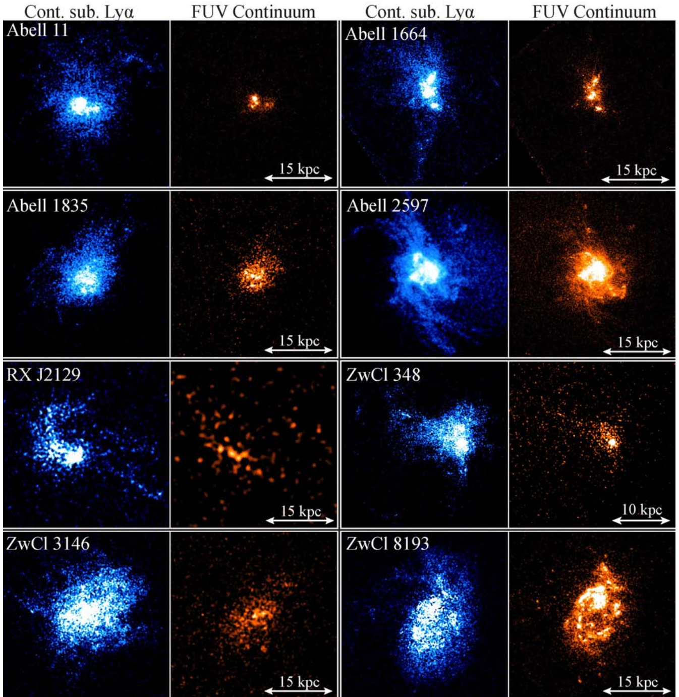
Figure 2. A comparison of Ly \alpha and FUV continuum morphologies for a subset of our sample. In blue, we show the HST /ACS SBC continuum-subtracted Ly \alpha images from O’Dea et al. (2010), and in orange we show the FUV continuum images. While the general morphologies are very similar, the Ly \alpha emission is far more extended than the underlying FUV continuum. This result is unsurprising given the sensitivity of Ly \alpha emission to resonant scattering. O’Dea et al. (2010) demonstrated that the underlying FUV continuum strength was sufficient to fully account for production of the observed Ly \alpha emission via stellar photoionization. All image pairs are aligned and shown on a common spatial scale, with east left and north up.
