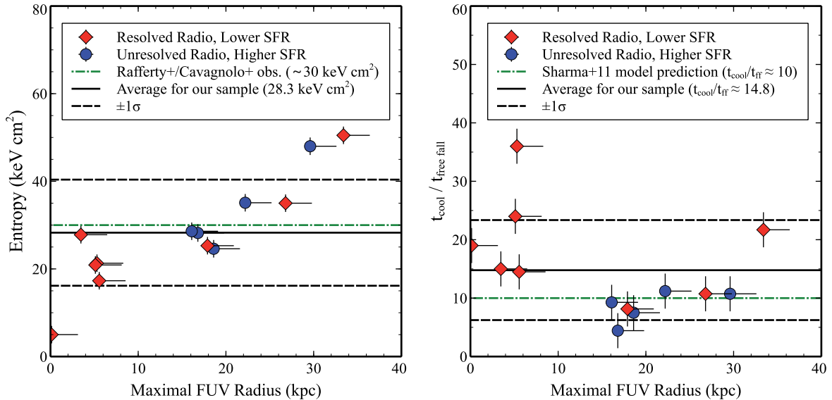
Figure 13. Here, we compare the maximal FUV radius with the X-ray entropy (left) and cooling-to-dynamical time ratios (right) measured at that same cluster-centric radius. Assuming (a) that the star formation in our sources is indeed powered by a cooling flow and (b) there is no non-detected star formation beyond the largest measured FUV radius, the maximal radius within which FUV emission is observed serves as a rough observable tracer of the radial threshold for the onset of cooling flow powered star formation. Within our sample, the average maximal radius (and its \pm 1\sigma interval) within which FUV continuum emission is detected is 14.7 \pm 10.14 kpc. At this average radius, the average (and \pm 1\sigma ) cooling time, entropy, and cooling-to-dynamical time ratio is 1.09 \pm 0.68 Gyr, 28.27 \pm 12.12 keV cm 2 , and 14.78 \pm 8.57 , respectively. These average values and their \pm 1\sigma intervals are marked by the black solid and dashed lines (respectively) on both panels. Blue and red points are used to differentiate between those sources with unresolved radio sources (and higher SFRs) and resolved radio sources (and lower SFRs). As entropy rises with radius, the points on the leftmost panel of course also rise (i.e. larger local entropies will be found at larger maximal FUV radii). Both results are found to be roughly consistent (although with large scatter) with the respective predictions by Cavagnolo et al. (2008) and Sharma et al. (2012a), which are marked by the green dashed line on both plots.
