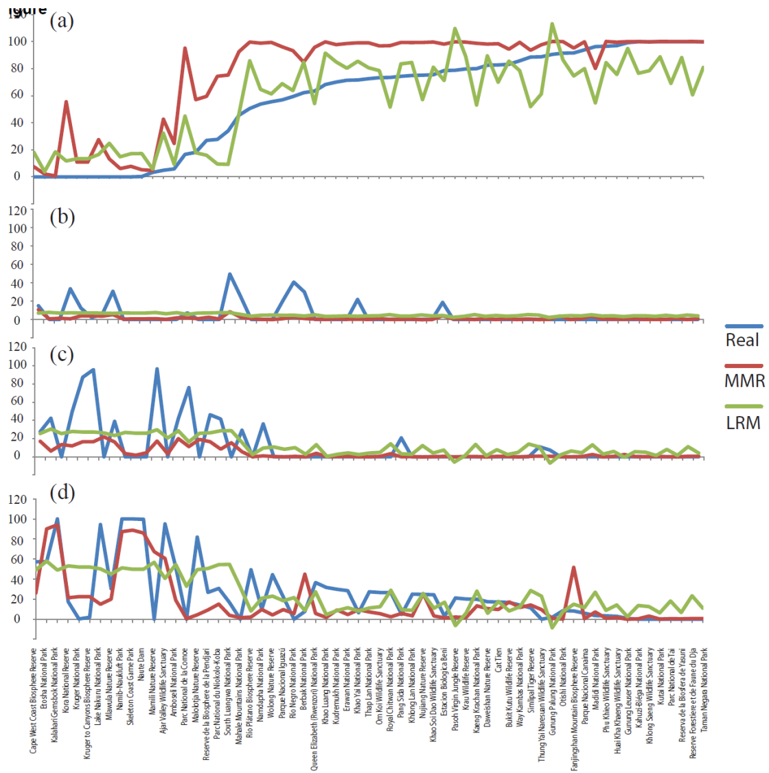
Figure 2. Comparisons between real and modelled values for each vegetation category. MMR represents the multiple multivariate regression of standardised values, LRM the linear regression of the principal components of the ecospace. (a) heavy tree cover [%Heavy]; (b) moderate tree cover [%Moderate]; (c) light tree cover [%Light]; (d) no tree cover [%Absent]. National protected areas are listed in order of increasing proportion of heavy tree cover over the 625km 2 sampled.
