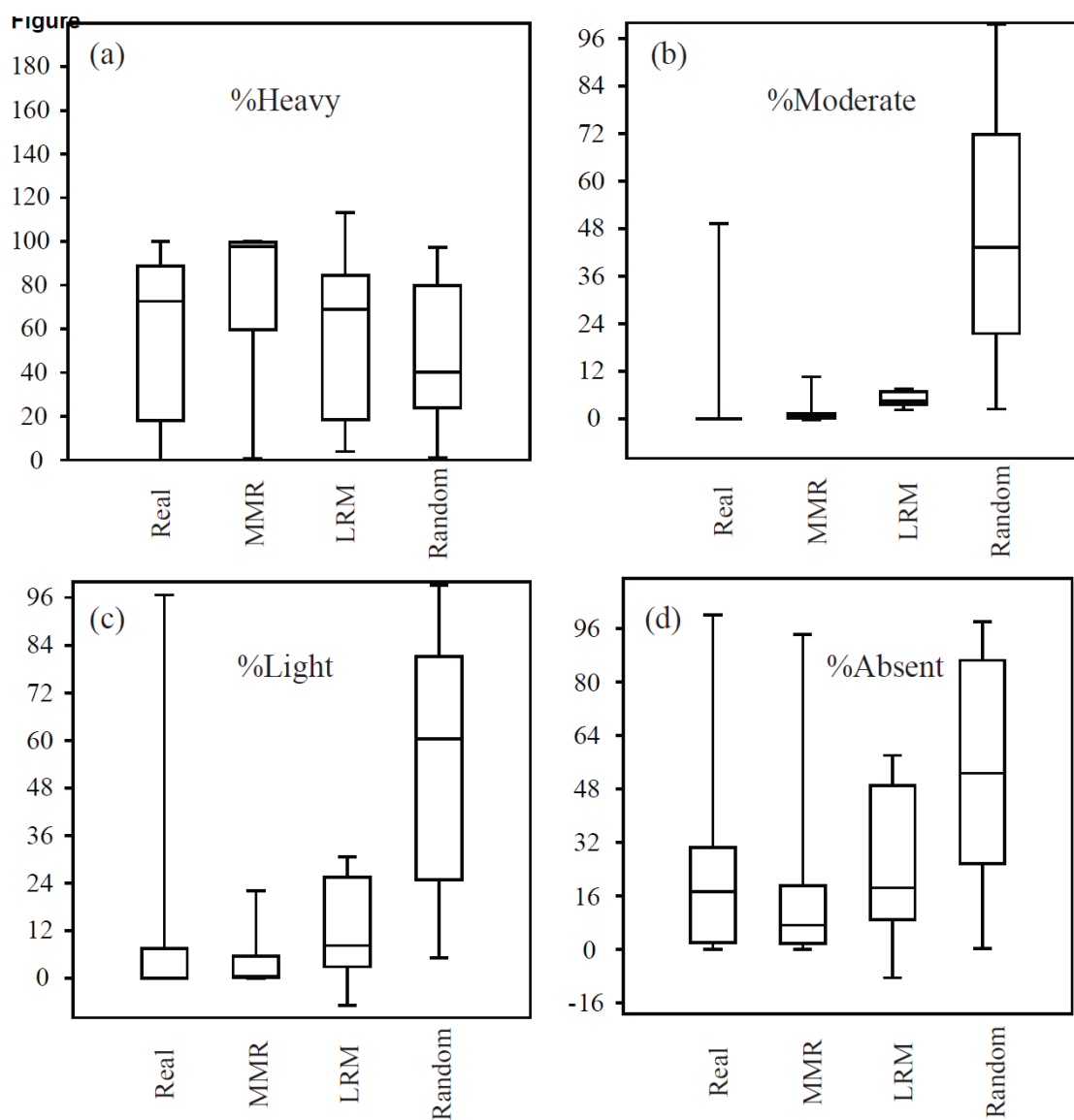
Figure 3. Box plot of real, modelled and random vegetation proportions. MMR represents the multiple multivariate regression of standardised values, LRM the linear regression of the principal components of the ecospace. (a) heavy tree cover [%Heavy]; (b) moderate tree cover [%Moderate]; (c) light tree cover [%Light]; (d) no tree cover [%Absent]. For each vegetation category, the 25-75% quartiles are drawn using the box, the median is shown with a horizontal bar inside said box, and maximum and minimum values are shown by the accompanying whiskers.
