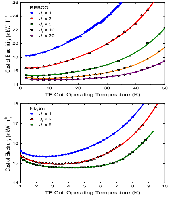
Figure 2: The cost of electricity in 1990 $ that has been found by minimising the major radius of a 500 MW net electricity tokamak operating at a given coolant temperature. The TF coils are constructed using the superconductors (a) REBCO and (b) Nb 3 Sn. The effect of increasing the critical current density in both superconductors is shown.
