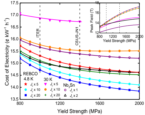
Figure 3: The cost of electricity in 1990 $ of a 500 MW fusion power plant as a function of the yield strength of the steel used to construct the TF coil casing. Results are plotted for Nb 3 Sn and for REBCO at different values of J_c (where J_c \times 2 refers to twice its current value). The peak operating field for the different superconductors is shown in the top right corner. The yield strength of structural materials for ITER is shown as well as the yield strength of the cryogenic steel, CSUS-JN1 [9].
