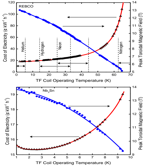
Figure 1: The cost of electricity in 1990 $ that has been found by minimising the major radius of a 500 MW net electricity tokamak operating at a given coolant temperature. The equivalent peak toroidal magnetic field is also shown. The TF coils are constructed using the superconductors (a) REBCO and (b) Nb 3 Sn. For (a) the temperature range over which some cryogenes are liquid is shown.
