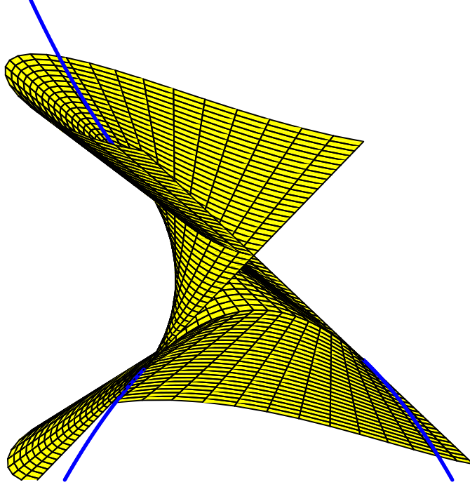
FIGURE 3. A cross section through the holy grill.
