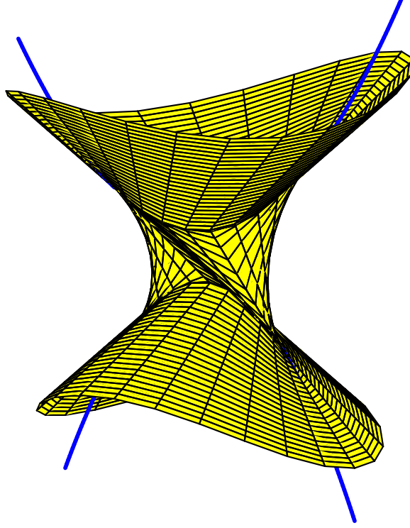
FIGURE 2. The holy grail. Here points of \mathbb{R}^3 have coordinates (\Re(\tau), \Im(\tau), \sigma) .
