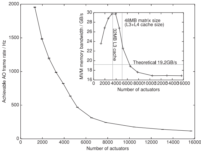
Figure 2. Maximum achievable RTCS frame rate as a function of number of actuators controlled for a 40 \times 40 subaperture system. Inset is shown the corresponding memory bandwidth required by the MVM to achieve this frame rate.
