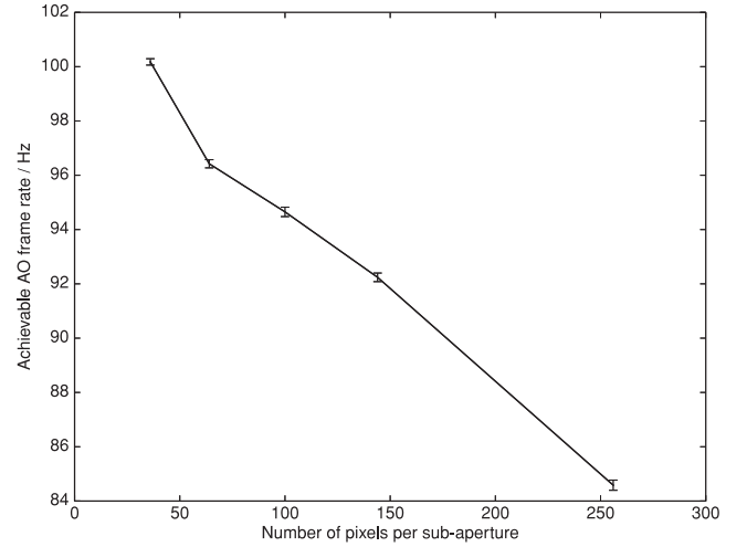
Figure 3. Maximum AO frame-rate as a function of number of pixels per subaperture (with 80 \times 80 square subapertures).
