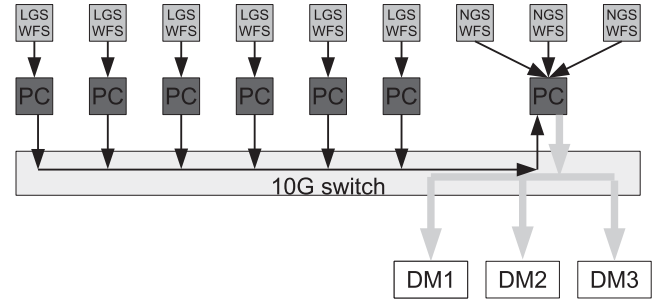
Figure 7. A schematic design showing components for a ELT MCAO real-time control system, and the links between them. WFSs are connected individually to a POWER8 server, which computes partial DM demands. These are then summed before being sent to the DM.
