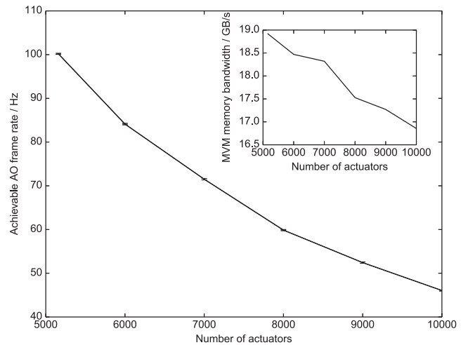
Figure 6. Maximum AO frame rate as a function of number of actuators controlled with 80 × 80 subapertures. Inset is shown the memory bandwidth required reach this frame rate for a given matrix size.
