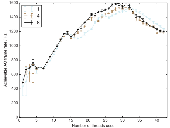
Figure 5. A figure showing achievable AO RTCS frame rates as a function of thread count on the low-end POWER8 system when wavefront reconstruction is not performed, for an ELT-scale SCAO system (80 × 80 subapertures).
