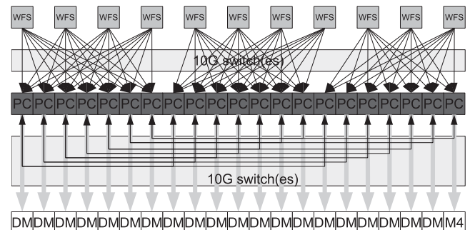
Figure 8. A schematic design showing components for a ELT MOAO real-time control system, and the links between them. Four WFSs are connected to a server, which computes slope measurements, and shares these with two other servers. Each server then has access to all WFS slope measurements, and computes DM demands for a single DM.
