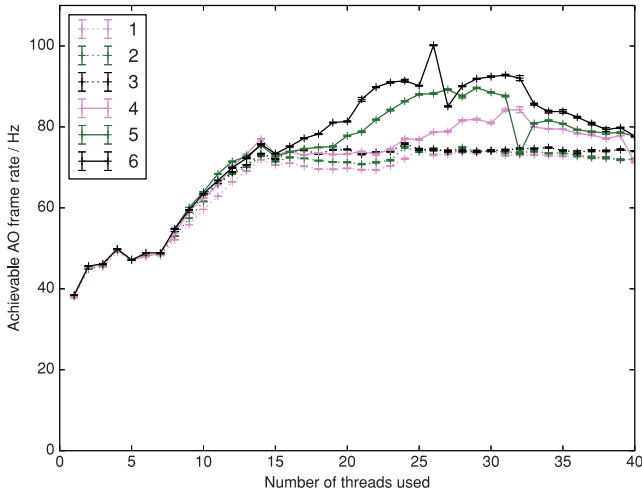
Figure 4. A figure showing how maximum achievable AO frame-rate is dependent on the number of processing threads used. The individual lines represent the number of times (given by the legend) threads are reused each frame.
