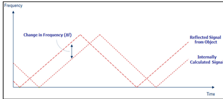
Figure 3: The Saw Tooth Wave of base Frequency 200THz that enables \Delta f to be calculated due to a fixed wavelength of 1500nm
