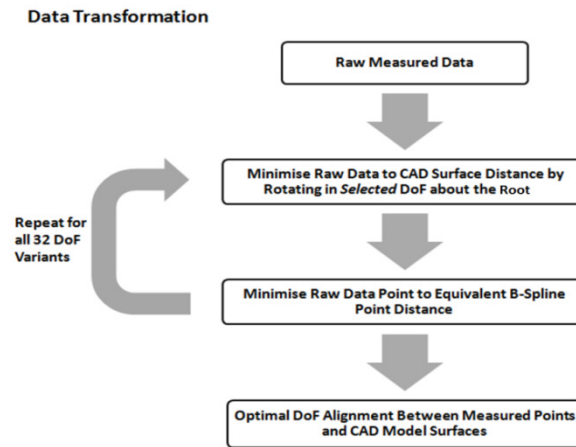
Figure 11: Blade test data transformation procedure
