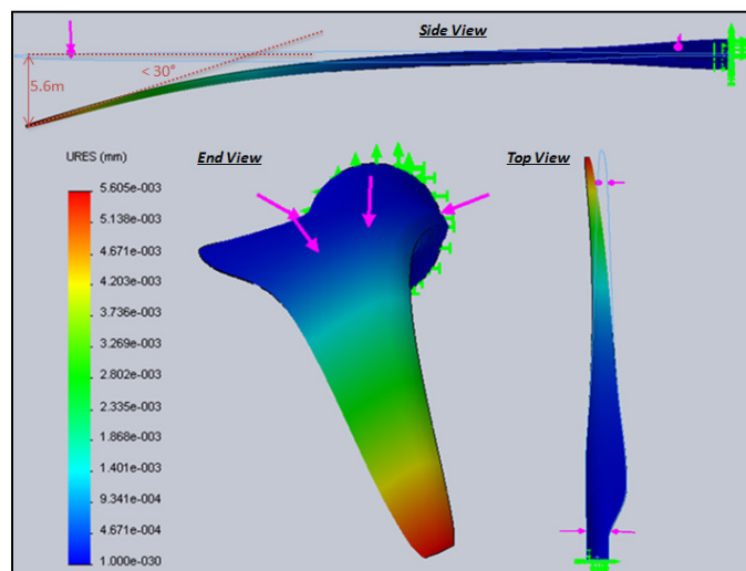
Figure 7: SolidWorks flex of blade analysis
