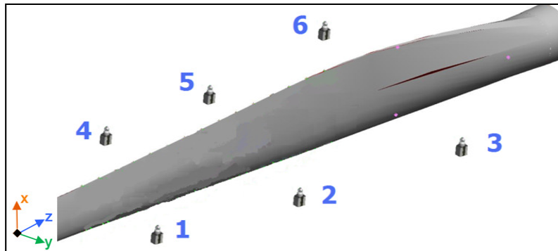
Figure 4: Inspection locations required for complete inspection of a 60m blade using LR
