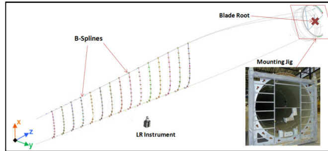
Figure 5: B-Spline generation about the blade chord and the Z-axis constraining mounting jig
