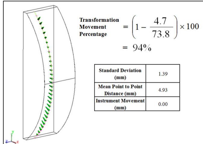
Figure 14: Optimum Experiment 2 alignment accuracy results. Shown in SA ( left ), the Transformation Movement Percentage and in performance raw data form ( right ).
