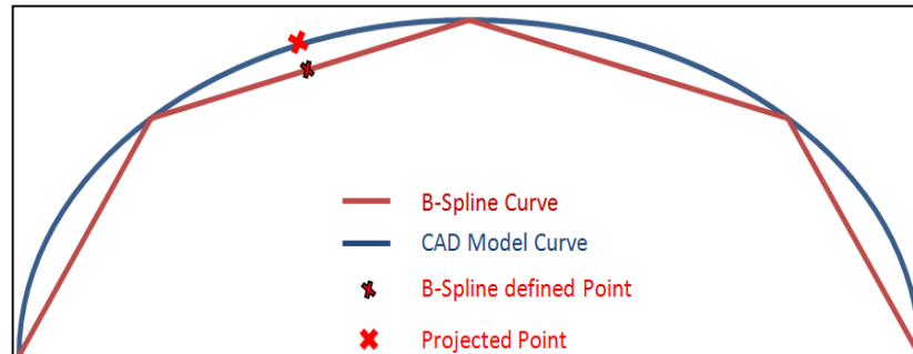
Figure 6: Illustration of the point location error caused by the difference in CAD model surface curve and B-Spline construction
