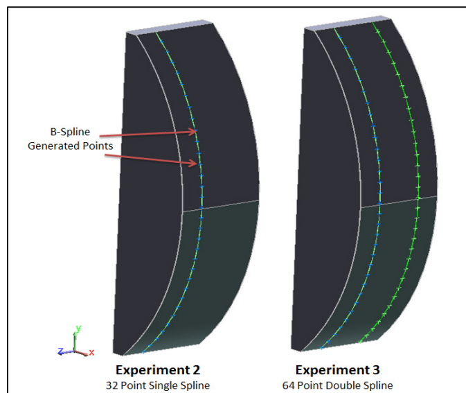
Figure 12: Experiment 2 and Experiment 3 B-Splines points, generated within SA
