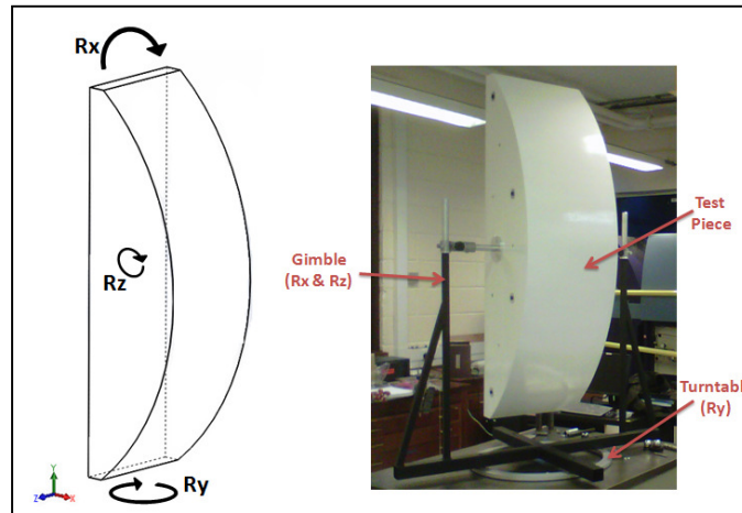
Figure 9: Left, the CAD model of the test piece with rotational DoF marked. Right, the test piece within the laboratory
