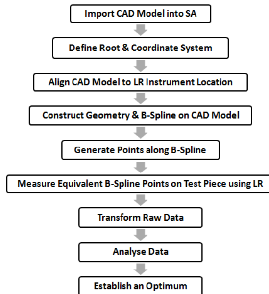
Figure 10: Blade test experimental procedure
