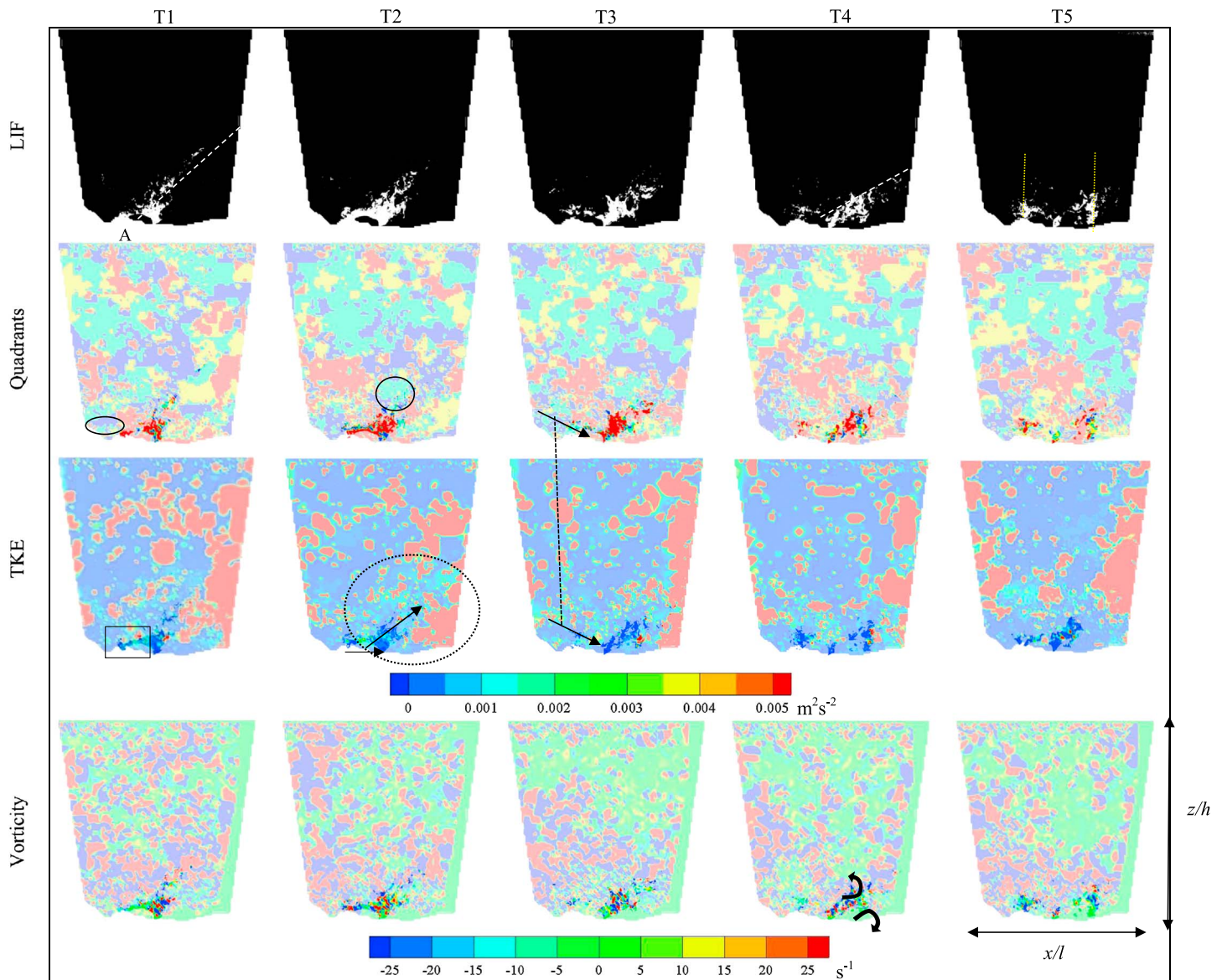
Figure 2. A time series of images 0.06 s apart taken from the flow conditions of Re\ 132\ 000 . (row 1) The identified flow structure is shown through processed (binary) images. Flow is analyzed through (row 2) instantaneous nonthresholded quadrants (Q1 (outward interactions) blue, Q2 (ejections) green, Q3 (inward interactions) yellow, and Q4 (sweeps) red), (row 3) turbulent kinetic energy (TKE), and (row 4) vorticity ( x - z ) where the flow structure is in full color and the surrounding flow has been plotted with 70% translucency. The lines, arrows, and ellipses identify regions of the flow discussed in detail in the text. The flow is from left to right.
