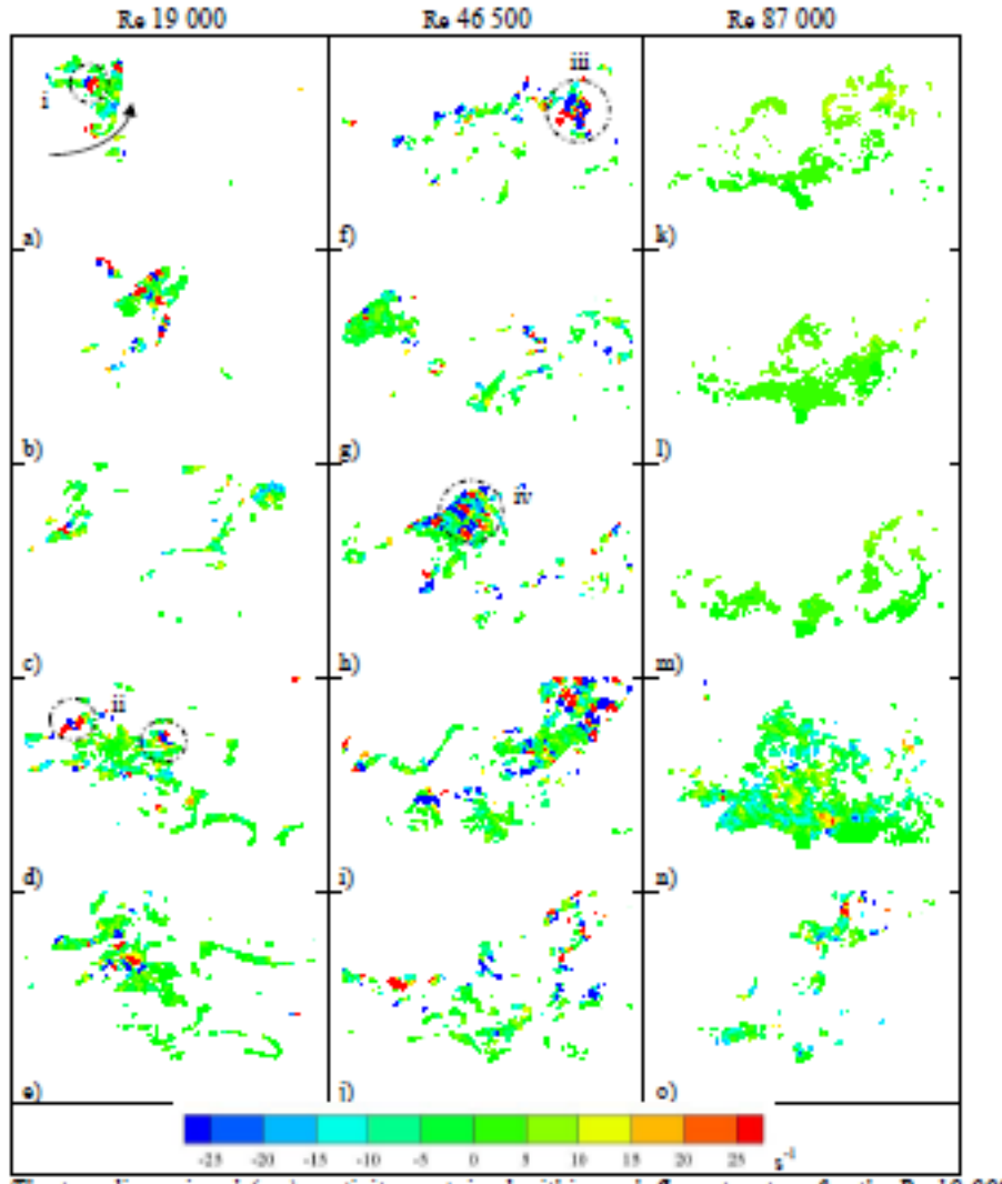
Figure 7: The two dimensional ( x - z ) vorticity contained within each flow structure for the Re 19 000 (a-e), the Re 46 500 (f-j) and the Re 87 000 experiment (k-o). The flow structures used are those identified in Figure 4. The images have been cropped in order to identify local vorticity and the relative scale of the structure can be seen in Figure 4. The arrows, and ellipses identify regions of the flow discussed in detail in the text. The flow is from left to right.
