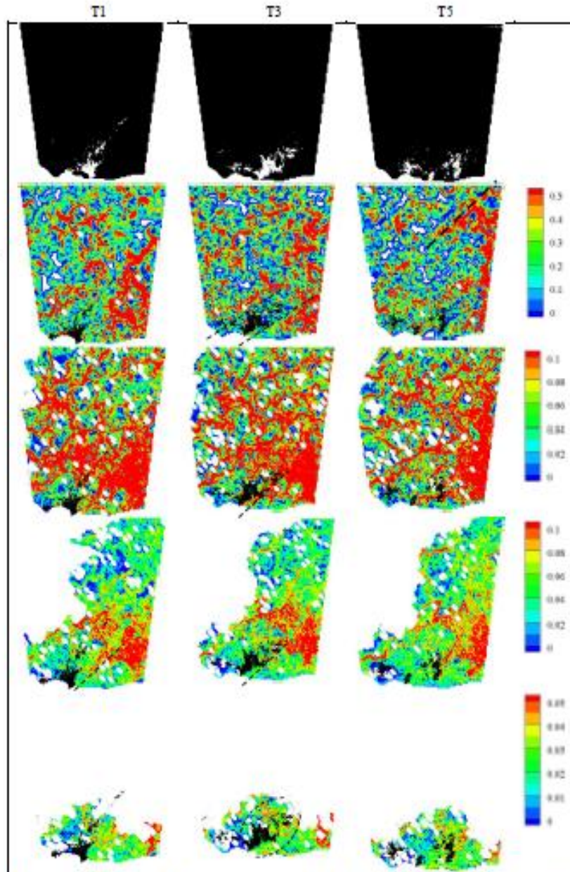
Figure 3: Finite-time Lyapunov exponents (FTLE) plots for T1, T3 and T5 (as shown in Figure 2) for the Re 132 000 experiment. The identified flow structure is shown through processed (binary) images in row 1. The FTLE is shown with a track back of 0.05 s (row2), 0.5 s (row3), 1 s (row3) and 2s (row4). The CFS is shown in black in the FTLE images, while the blank area shows either areas where no significant structures are identified. The lines and ellipse identify regions of the flow discussed in detail in the text. The flow is from left to right.
