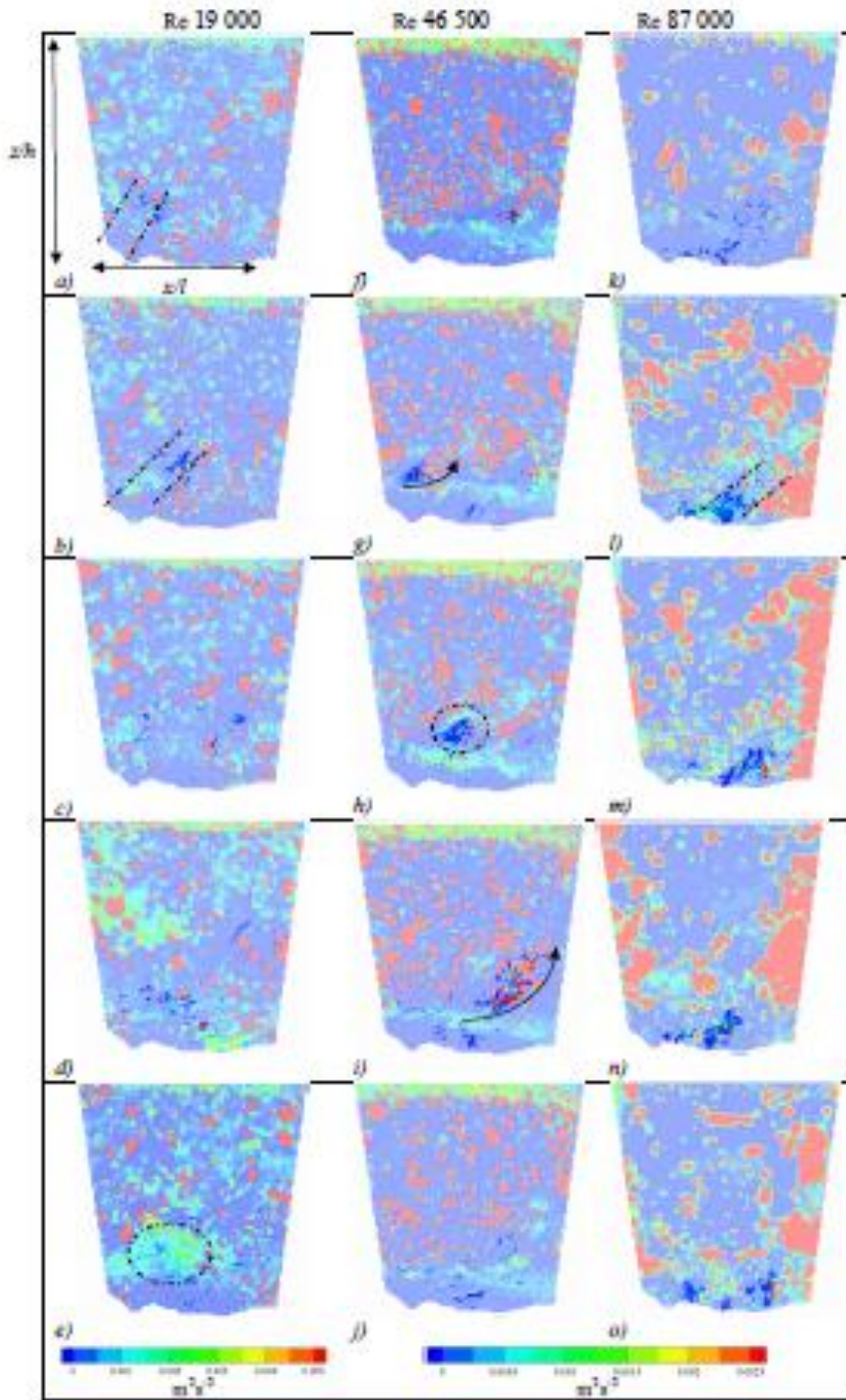
Figure 6: Turbulent Kinetic Energy for the Re 19 000 (Column 1), the Re 46 500 (Column 2) and the Re 87 000 experiment (Column 3). The full illumination is the identified flow structure, while the 70% translucent image is the rest of the flow field. The flow structures used are those identified in Figure 4. z/h and x/l represents the dimensional height and length of the field of view. The lines, arrows, and ellipses identify regions of the flow discussed in detail in the text. The flow is from left to right.
