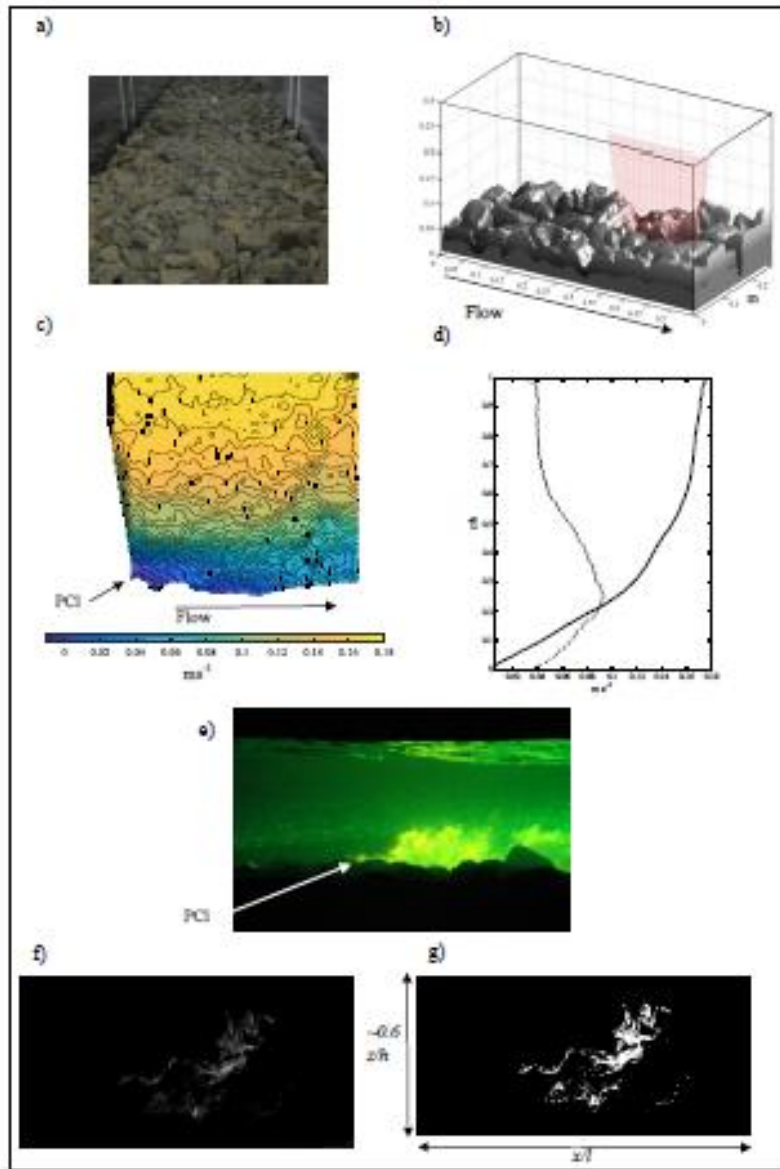
Figure 1: The experimental set up: a) the gravel in the flume. The grain size distribution has a D_{50} of 44 mm and a D_{84} of 66 mm; b) A DEM collected through Terrestrial Laser Scanning. The red shaded area demonstrates the area illuminated by laser; c) The mean downstream ( u -) velocity component for the Re 132 000 experiment demonstrating the whole flow measurement with the PIV; d) An example of a mean velocity (solid line) and turbulence intensity (dotted line) profile extracted from the Re 132 000 experiment e) a side on view of the flume where the flow is illuminated by the laser, PIV seeding is illuminated and the coherent flow structures can be identified by the Rhodamine 6G dye; f) a raw LIF image. Length of abscissa axis is equal to 0.35 metres whilst the ordinate axis is equal to 0.285 meters. g) An example of the conversion of a raw LIF image into a binary image using the Otsu (1979) image conversion algorithm, which determines the mask for the coherent turbulent flow structure PIV data. PCI in c and f identify the protruding clast.
