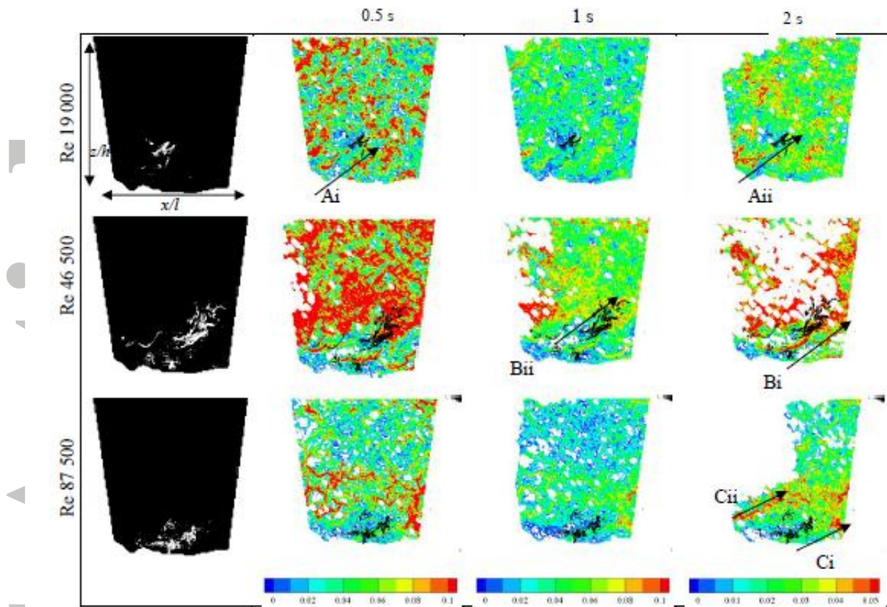
Figure 8: Vortex detection using FTLE for selected flow structures. The structure is shown (Column 1) and then tracked back using FTLE for 0.5 seconds (Column 2), 1 second (Column 3) and 2 seconds (Column 4) for the Re 19 000 experiment (Row 1), Re 46 500 experiment (Row 2) and Re 87 500 experiment (row 3). The images chosen (column 1) have been previously analysed and correspond to: Re 19 000 (Figure 4b); Re 46 500 (Figure 4i) and; Re 87 500 (Figure 4l). The blank area shows either areas where no significant structures are identified. z/h and x/l represents the dimensional height and length of the field of view. The lines, arrows, and ellipses identify regions of the flow discussed in detail in the text. The flow is from left to right.
