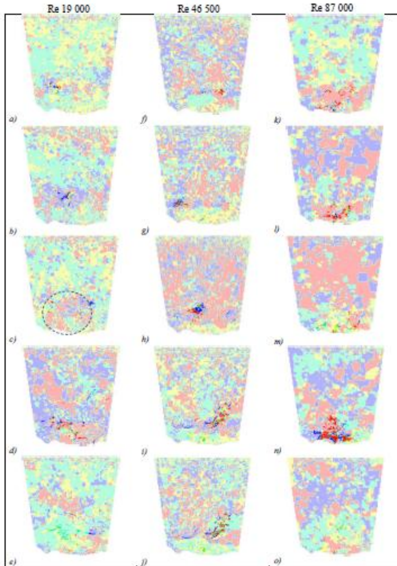
Figure 5: Quadrant plot for the Re 19 000 (a-e), the Re 46 500 (f-j) and the Re 87 000 experiment (k-o). The full illumination is the identified flow structure, while the 70 % translucent image is the rest of the flow field. The flow structures used are those identified in Figure 4. Quadrant 1 (Outward Interactions) = Blue; Quadrant 2 (Ejections)= Green; Quadrant 3 (Inward Interactions)= Yellow; Quadrant 4 (Sweeps)= Red. The ellipse identifies regions of the flow discussed in detail in the text. The flow is from left to right.
