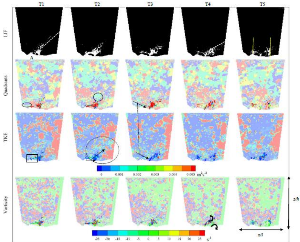
Figure 2: A time series of images 0.06 seconds apart taken from the flow conditions of Re 132 000. The identified flow structure is shown through processed (binary) images in row 1. Flow is analysed through i) Instantaneous non-thresholded quadrants ( Q1 (Outward Interactions) blue; Q2 (Ejections) green; Q3 (Inward Interactions) yellow; & Q4 (sweeps) red), (Row 2); ii) Turbulent Kinetic Energy (TKE), (Row 3) and; iii) Vorticity ( x - z ) (Row 4) where the flow structure is in full colour and the surrounding flow has been plotted with 70% translucency. The lines, arrows, and ellipses identify regions of the flow discussed in detail in the text. The flow is from left to right.
