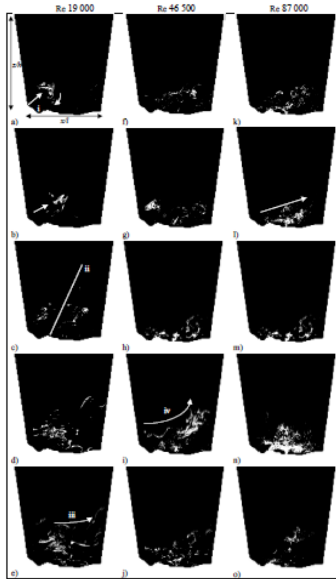
Figure 4: A series of CFS detected by the LIF for the Re 19 000 (a-e), the Re 46 500 (f-j) and the Re 87 000 experiment (k-o). The images have been converted into binary using the Otsu (1979) algorithm. The lines and arrows identify regions of the flow discussed in detail in the text. The flow is from left to right.
