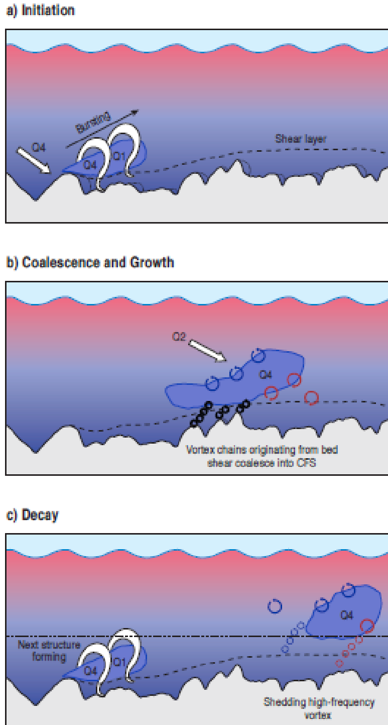
Figure 9: A conceptual model for the initiation (A), growth (B) and decay (C) of a large-scale coherent flow structure over a gravel bed. The black line represents the topography used in the experiments, while the black dashed line represents the shear layer formed through the interaction with the large topographic protrusion to the left of the cartoon, and as previously observed in Hardy et al. [2009]. The CFS detected by the LIF is coloured blue; red arrows represent clockwise vorticity; blue arrows represent anticlockwise vorticity; black arrows represent vortex chains, with their diameter being a schematic indication of their size. Q refers to the dominant quadrant structure identified following the definition of Lu and Willmarth [1972]. Initiation of the structure (A) occurs through generation of horseshoe-
