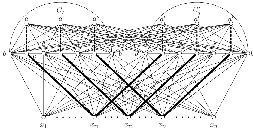
Fig. 2. The graph G for the clause C_j = \{x_{i_1}, x_{i_2}, x_{i_3}\} .
