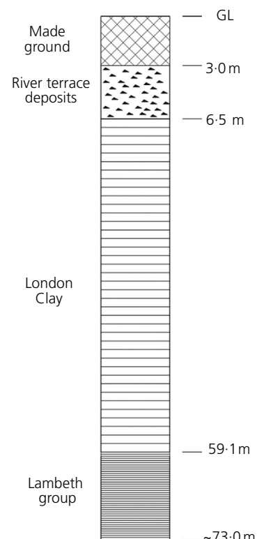
Figure 1. Ground profile at Crossrail Paddington
