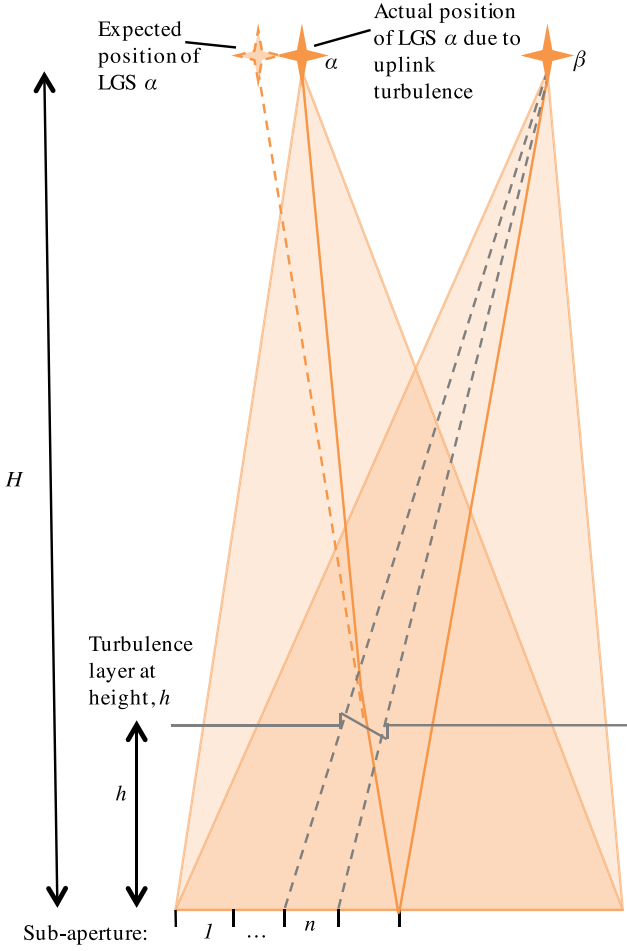
Figure 2. The geometry of the LGS system under consideration. One turbulent layer is shown, which features only a tilt at the point that LGS \alpha overlaps with the FOV of sub-aperture n on WFS \beta .
