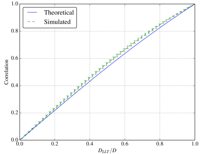
Figure 1. Theoretical and simulated correlation of phase perturbations in Kolmogorov turbulence between concentric tip-tilt modes as a function LLT diameter, D_{\text{LLT}} , as a fraction of the telescope diameter, D .
