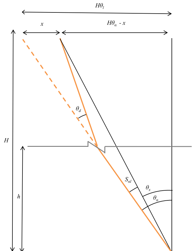
Figure A1. The displacement on LGS \alpha caused by a turbulence encountered on up-link.
