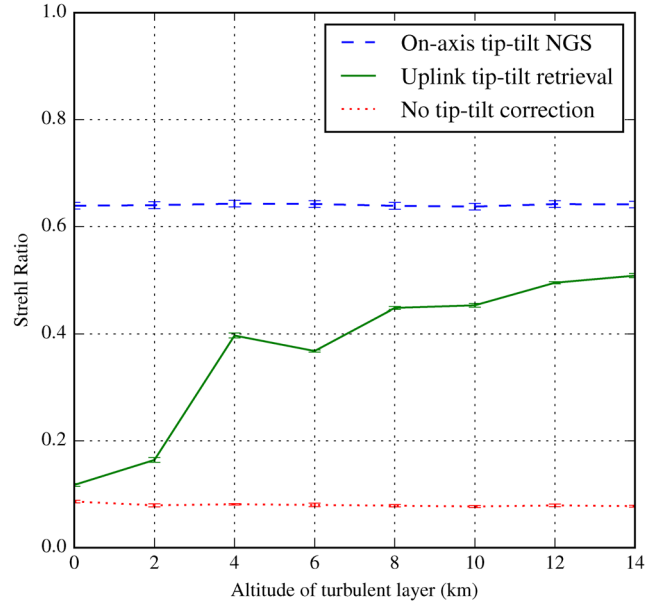
Figure 4. The Strehl ratio of tomographic LGS AO with a NGS tip-tilt sensor (dashed), the tip-tilt retrieval method (solid) and no tip-tilt correction (dotted) versus the altitude of a single turbulence layer. The LGS up-link tip-tilt determination performance increases sharply as the layer altitude increases.
