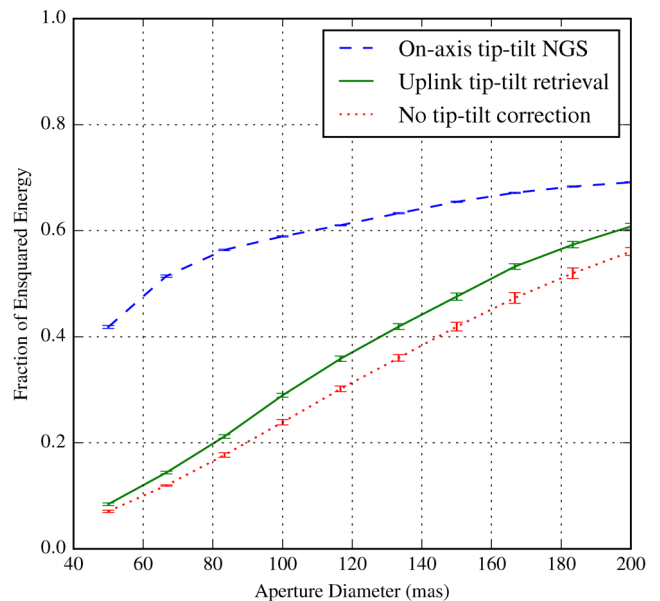
Figure 7. Ensquared energy versus aperture size of LTAO with an on-axis tip-tilt NGS (dashed), with no NGS and the tip-tilt retrieval (solid) and with no tip-tilt correction (dotted). Though never approaching that of LTAO with an on-axis NGS, the tip-tilt retrieval improves throughput over the case when no tip-tilt correction is performed.
