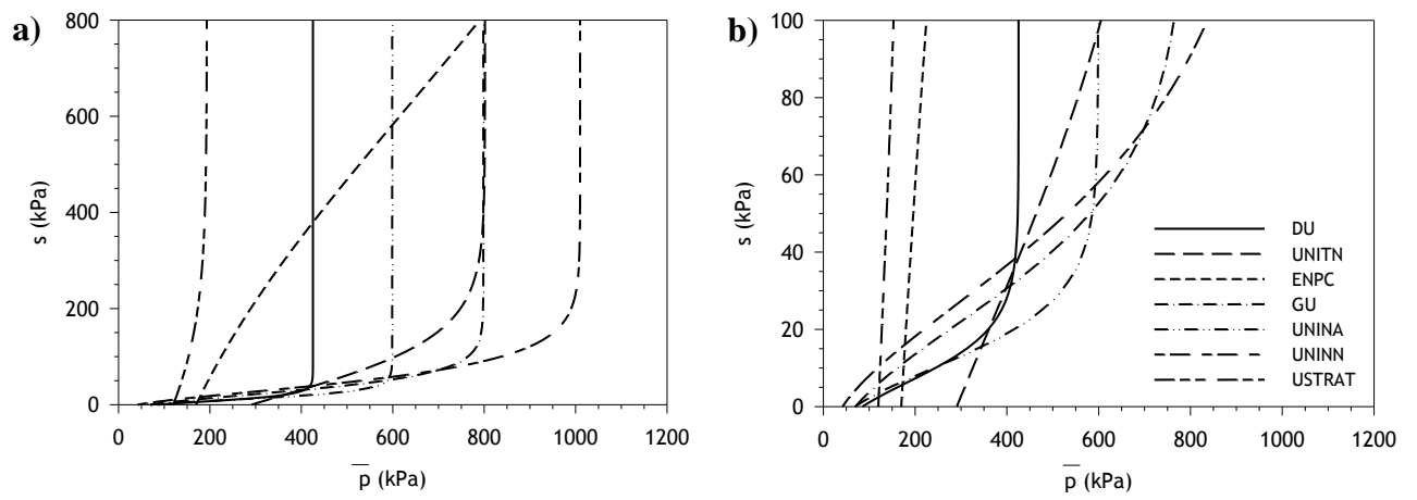
Fig. 9. Initial form of LC yield curve predicted by different teams: (a) full suction range; (b) magnified view of low suction range.
