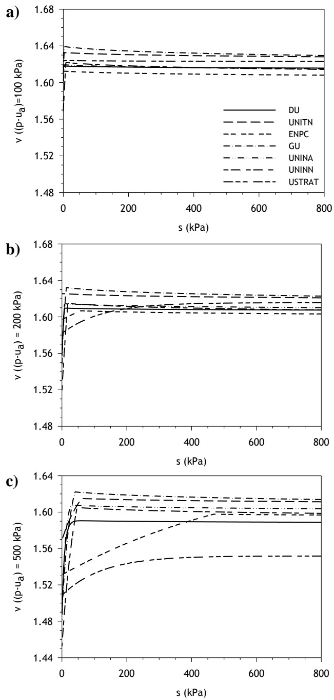
Fig. 17. Predicted variation of specific volume during wetting at a mean net stress of: (a) 100 kPa; (b) 200 kPa; (c) 500 kPa.
