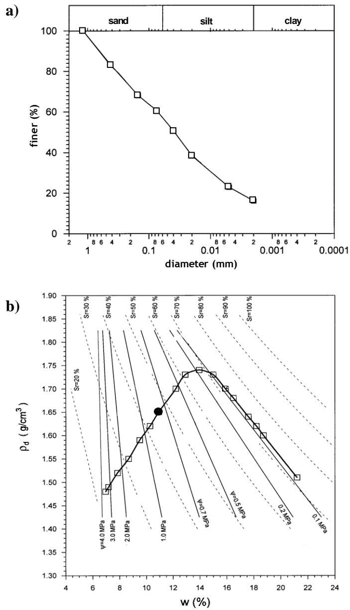
Fig. 1. (a) Particle size distribution; (b) compaction curve.
