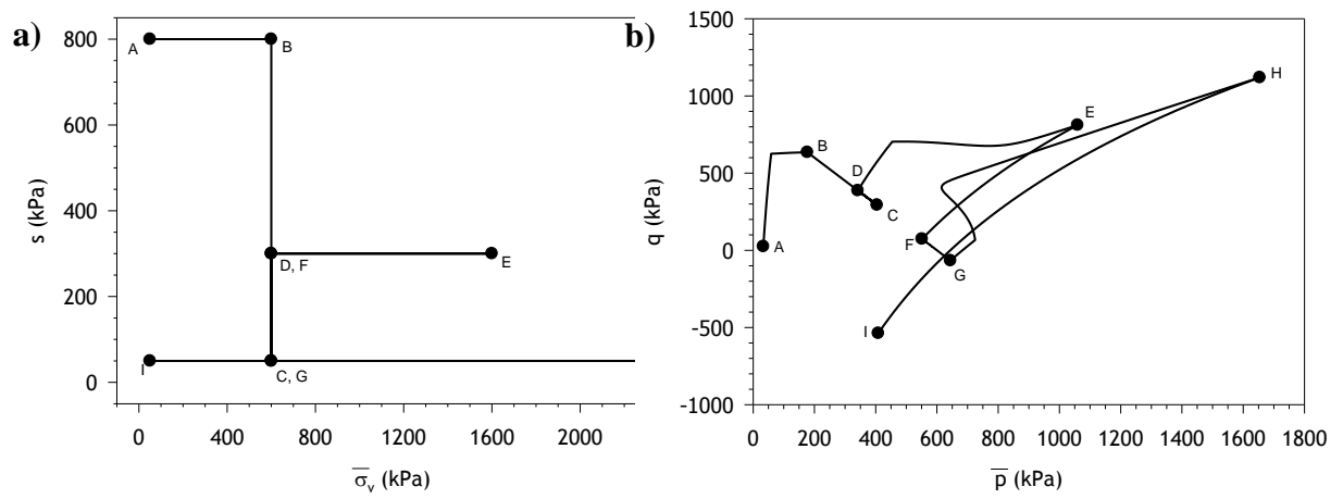
Fig. 14. Oedometer test EDO-1 (a) stress path in s - \bar{\sigma}_v plane; (b) stress path in q - \bar{p} plane predicted by ENPC.
