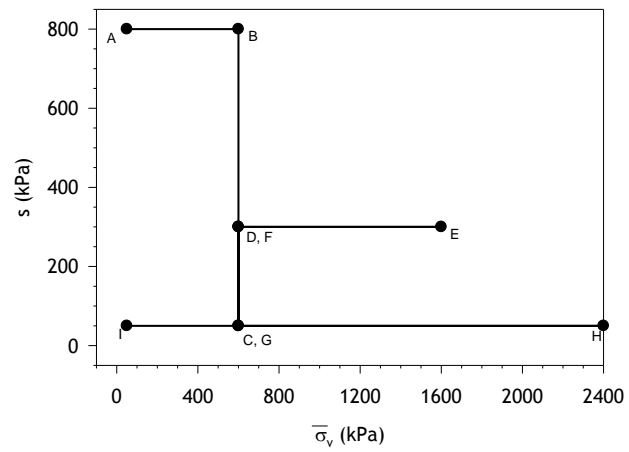
Fig. 4. Stress path for suction-controlled oedometer test EDO-1.
