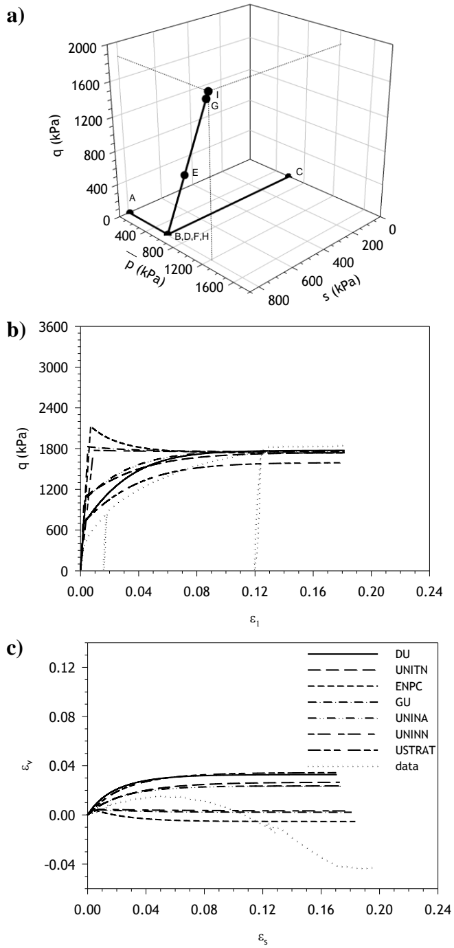
Fig. 13. Suction-controlled triaxial test IWS-OC-01: (a) stress path; (b,c) Simulations and experimental data for shearing stage D-I.
