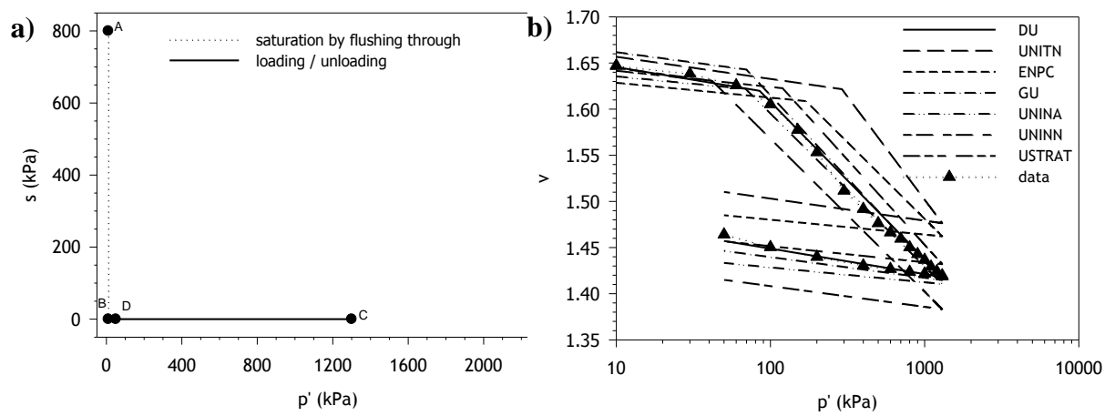
Fig. 10. Saturated isotropic test SAT-1: (a) stress path; (b) simulations and experimental data.
