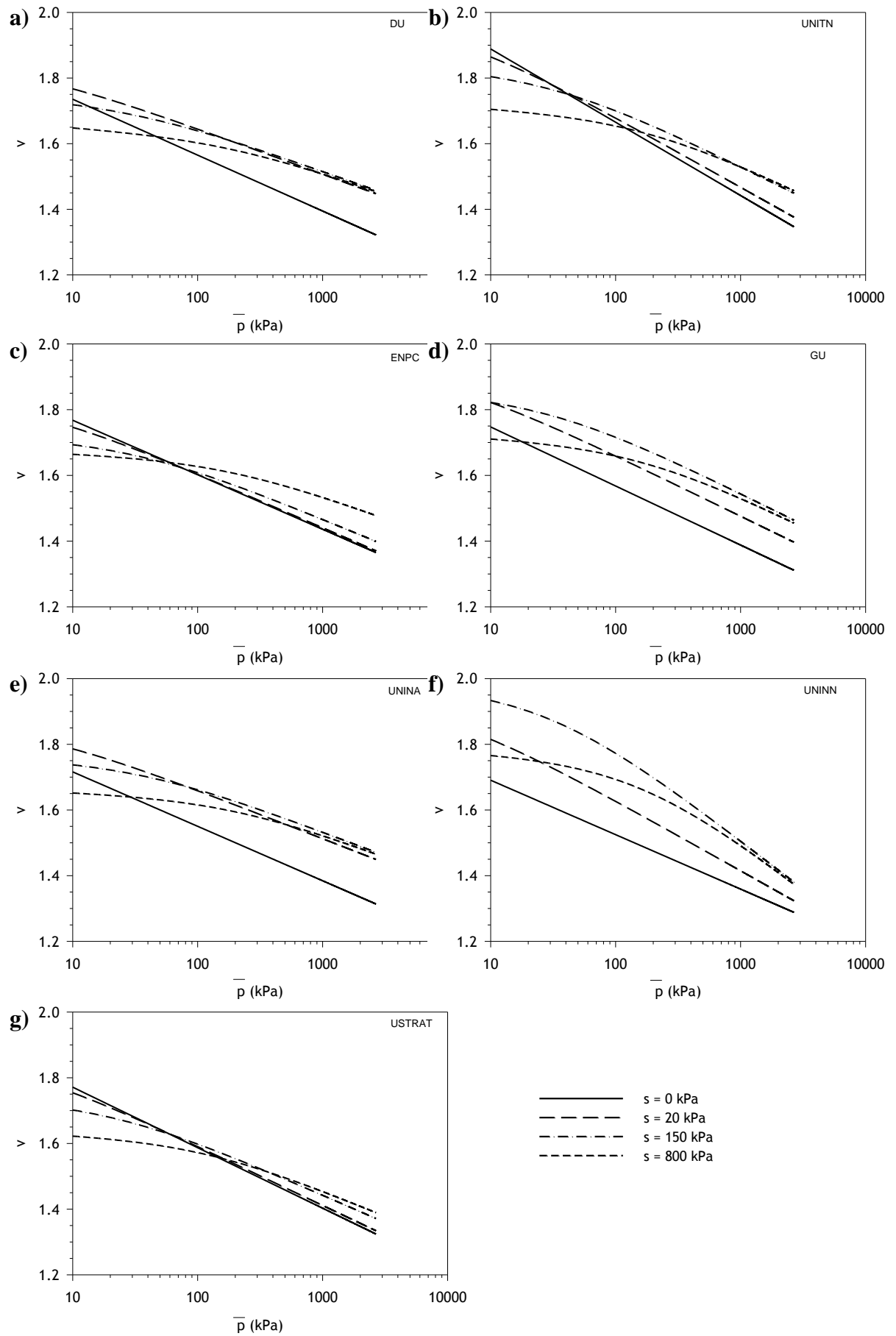
Fig. 8. Predicted critical state lines for different values of suctions in v : \ln p plane.
