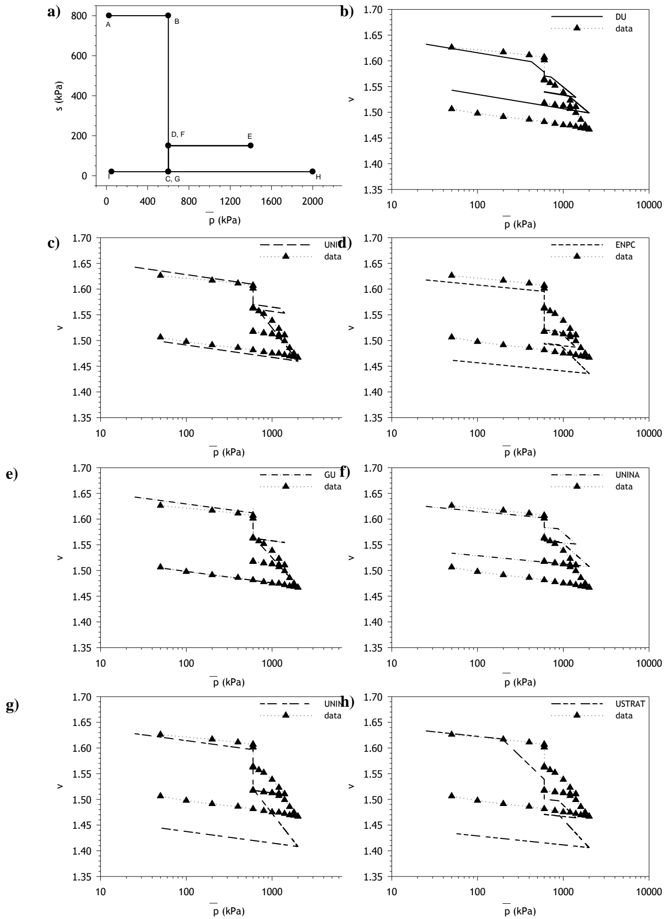
Fig. 11. Suction-controlled isotropic test TISO-1: (a) stress path; (b)-(h) simulations and
