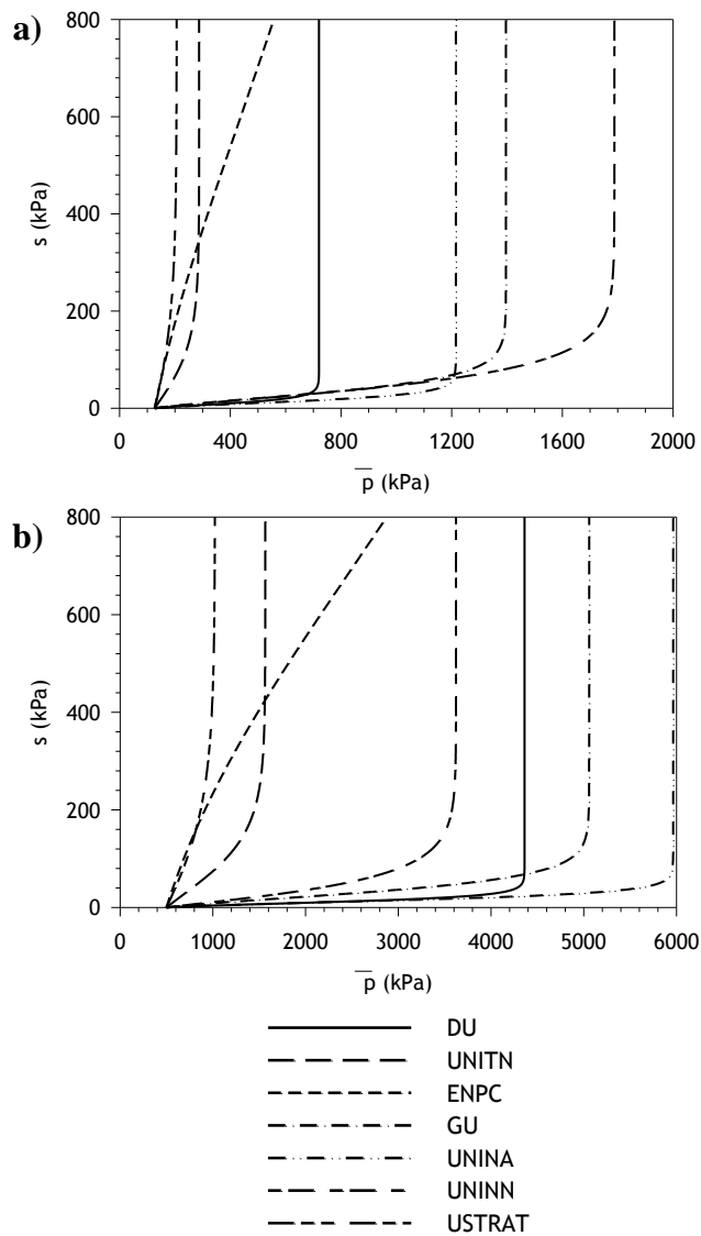
Fig. 16. LC yield curve predicted by different teams for: (a) \bar{p}(0) = 120 kPa; (b) \bar{p}(0) = 500 kPa.
