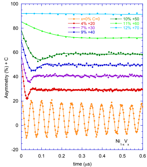
Figure 2. Asymmetry of \text{Ni}_{1-x}\text{V}_x vs time for different V-concentrations x , ranging from x = 0 to x = 12.3\% at low temperatures ( 1.5\text{K} < T < T_c/4 ). Each is shifted by a constant C for clarity. The line represents a fit to the oscillator model with P_{osci} .
