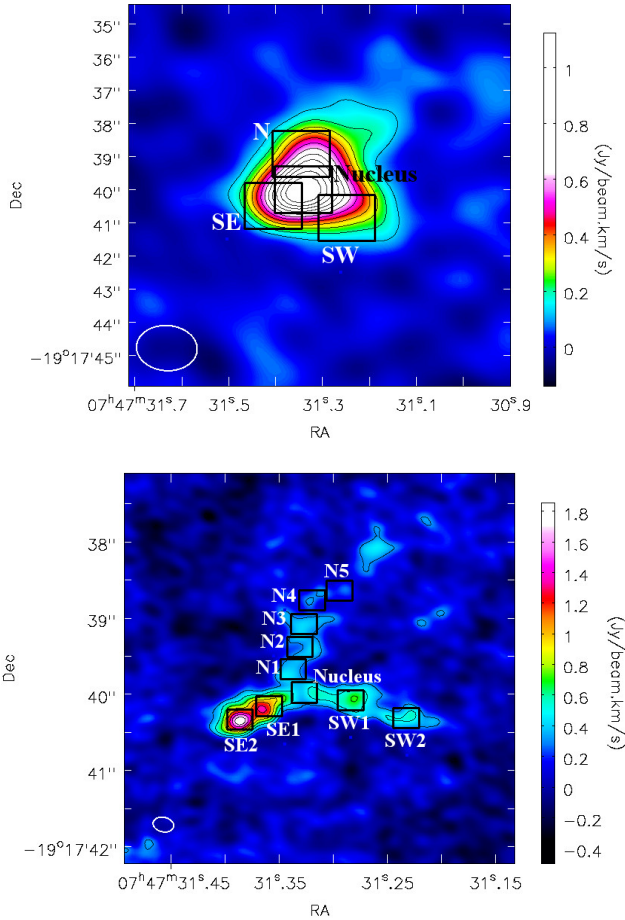
Figure 5. PKA 0745-191 CO(1-0) (top) and CO(3-2) (bottom) integrated intensity maps (as shown in Fig. 2) with regions overlaid corresponding to the spectra shown in Figs. 6 and 7.
