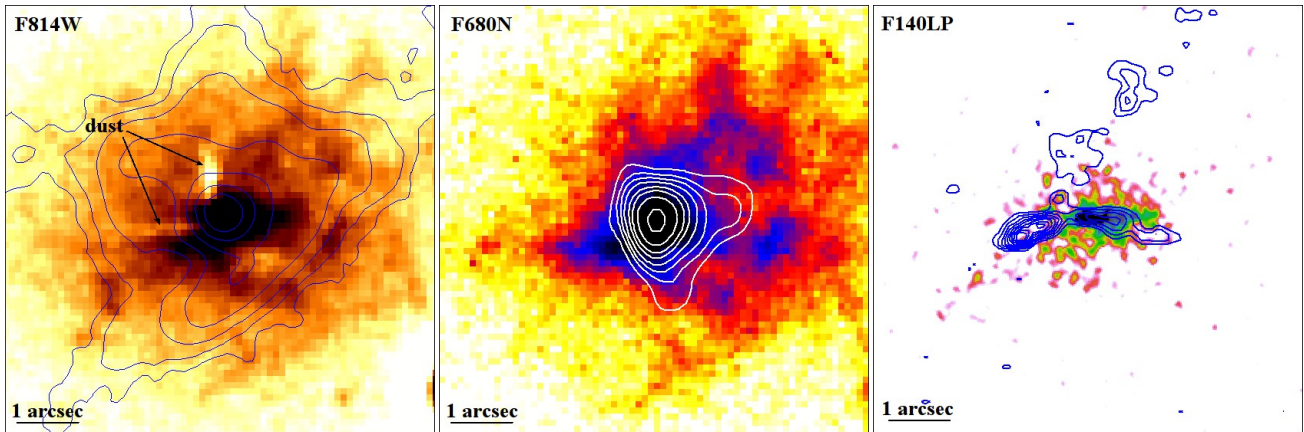
Figure 9. Left: HST F814W image of the brightest cluster galaxy showing the old stellar population and H\alpha + [NII] emission (Sand et al. 2005; Mittal, Whelan & Combes 2015; Tremblay et al. 2015). A smooth model has been subtracted to show the dust lanes extending to the N and E of the nucleus. Contours show the 5 GHz VLA radio emission from Baum & O’Dea (1991). Centre: Narrow band image covering the H\alpha + [NII] emission (Donahue et al. 2000) with the 14.9 GHz VLA B array contours overlaid (Baum & O’Dea 1991). Right: F140LP SBC image of FUV continuum emission from massive, young stars (Mittal, Whelan & Combes 2015; Tremblay et al. 2015) with ALMA CO(3-2) integrated intensity contours overlaid. All images are centred on the nuclear continuum point source emission (section 2).
