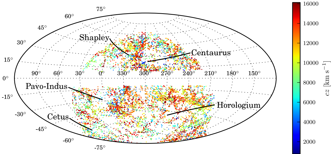
Figure 1. Distribution of 6dFGSv galaxies in Galactic latitude ( l ) and longitude ( b ), shown in an equal-area Aitoff projection. Individual galaxies are colour-coded by their redshift. The 6dFGSv galaxies fill the Southern hemisphere apart from \pm 10^\circ about the Galactic plane. Some of the large-scale structures in the 6dFGSv volume are also indicated.
