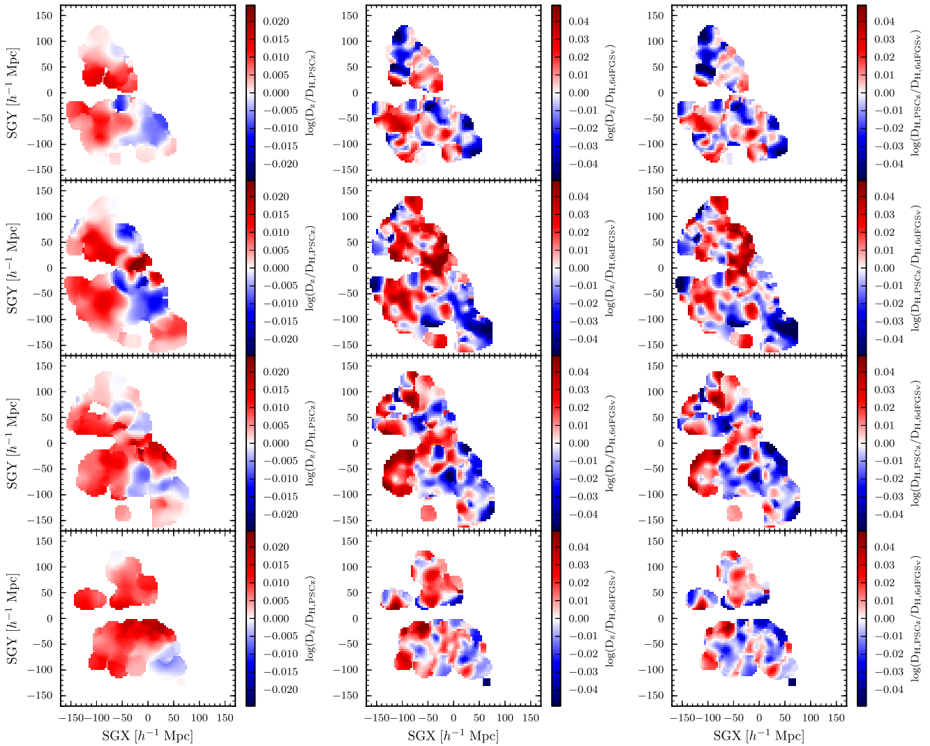
Figure 10. Same as Fig. 9, but with the PSCz velocity field (Branchini et al. 1999) in place of the 2MRS field.
