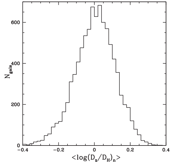
Figure 7. Distribution of \langle \Delta d_n \rangle = \langle \log(D_z/D_H)_n \rangle , the expectation values of the logarithm of the ratio of redshift distance to Hubble distance \Delta d_n for each of the 8885 galaxies in the 6dFGSv sample.
