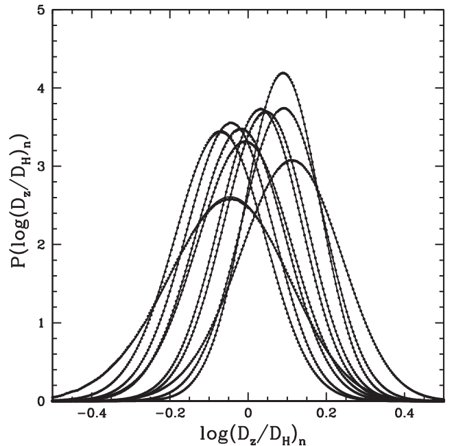
Figure 6. For 10 randomly chosen galaxies in 6dFGSv, we show the probability density distribution of \Delta d_n = \log(D_z/D_H)_n , which is the logarithm of the ratio of the comoving distance associated with galaxy n 's redshift to the true comoving distance of the galaxy. The exact probability distributions are represented by circles, whereas the approximations from equation (21) are represented by solid lines.
