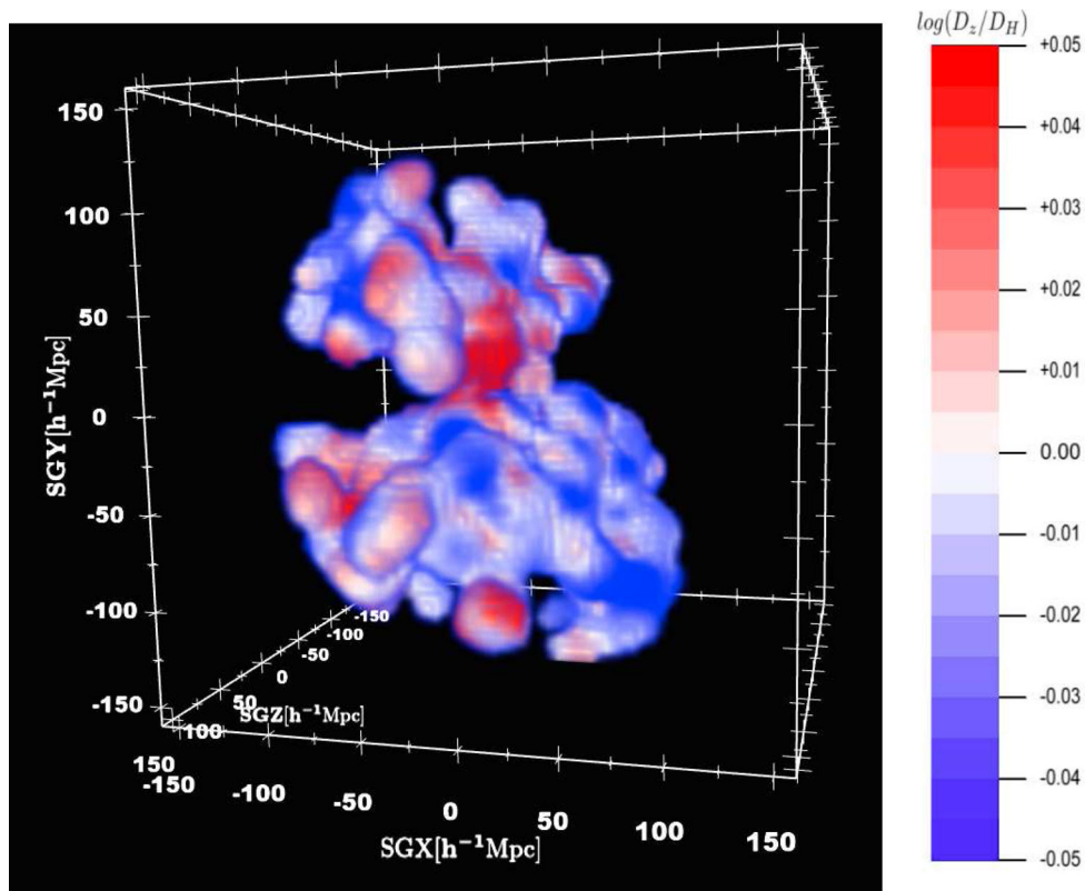
Figure 11. The smoothed 6dFGSv peculiar velocity field in 3D, plotted on a grid in supergalactic Cartesian coordinates, with gridpoints colour-coded by the value of \Delta d = \log(D_z/D_H) . Adobe Reader version 8.0 or higher enables interactive 3D views of the plot, allowing rotation and zoom.
