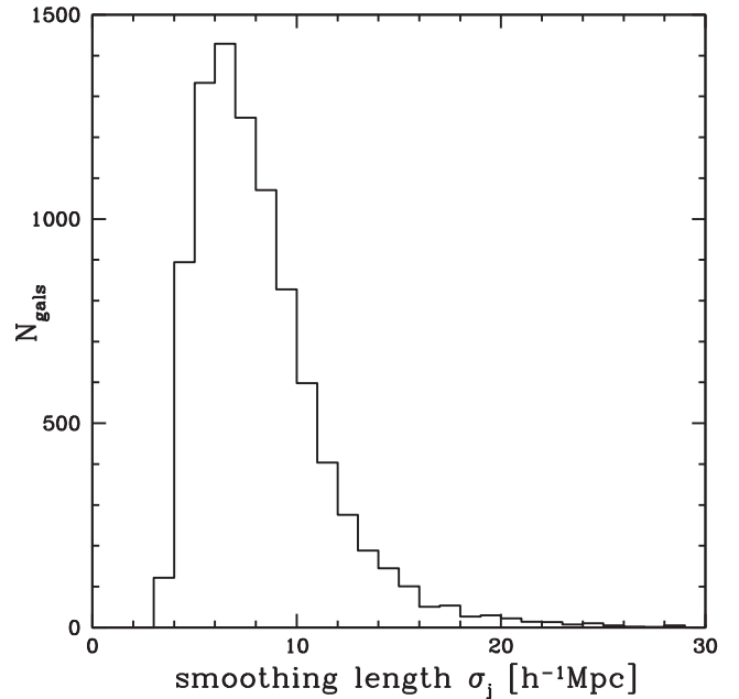
Figure 8. Distribution of smoothing lengths, \sigma_j , for all 6dFGSv galaxies, following equation (24).
