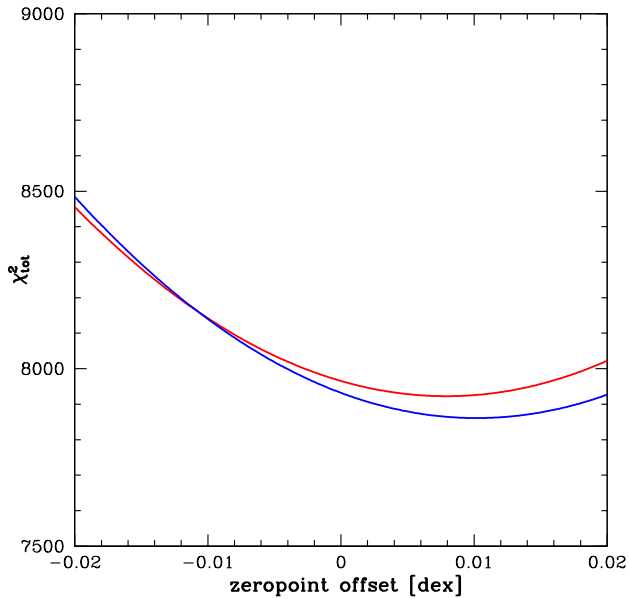
Figure 14. \chi_{\text{tot}}^2 as a function of the zero-point offset for 2MRS (red) and PSCz (blue). The best-fitting zero-point offsets are +0.0080 and +0.0102 dex for 2MRS and PSCz, respectively. These mean that the values of \Delta d would be shifted correspondingly lower in each case.
