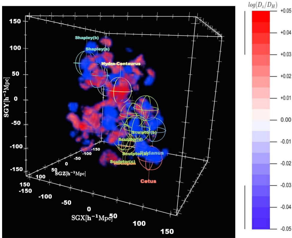
Figure 12. Same as Fig. 11, except that we only show gridpoints with \Delta d = \log(D_z/D_H) either greater than +0.03 or less than -0.03, in order to highlight the regions with the most extreme values. We also label each of the features of large-scale structure labelled in Fig. 3. Though they are outside the survey volume, we include labels for the Vela and Horologium-Reticulum superclusters, as they exert influence on the local velocity field. To toggle the visibility of individual superclusters in the interactive figure (Adobe Reader), open the Model Tree, expand the root model, and select the required supercluster name.
