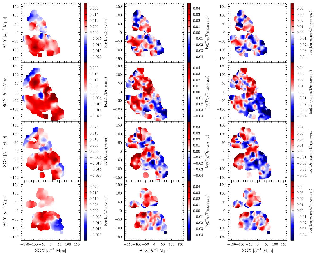
Figure 9. Adaptively smoothed versions of the reconstructed 2MRS velocity field, as derived by Erdoğan et al. (2014) (left), the observed 6dFGS velocity field (centre) and the observed 6dFGS field minus the 2MRS reconstruction (right), in the same four slices of SGZ that are displayed in Fig. 3. In each case, the velocity field is given in logarithmic distance units ( \Delta d = \log(D_z/D_H) ), in the nomenclature of Section 4.1), as the logarithm of the ratio between the redshift distance and the true Hubble distance. As shown in the colour bars for each panel, redder (bluer) colours correspond to more positive (negative) values of \Delta d , and thus more positive (negative) peculiar velocities. Gridpoints are spaced 4 h^{-1} Mpc apart.
