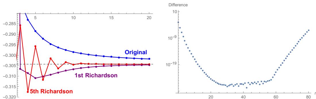
Figure 3. (Left) We show the convergence behavior of the original sequence a_\ell^{(1)} , its first and fifth Richardson transforms by the blue, purple and red curves, respectively. The black dashed line is the expected convergence value \mathcal{A}_1 . The Richardson extrapolation accelerates the convergence. (Right) The difference |1 - \mathcal{R}_n[a_{180-n}^{(1)}]/\mathcal{A}_1| is shown as a function of n . In this case, the Richardson extrapolation is especially good for the range 20 \lesssim n \lesssim 60 .
