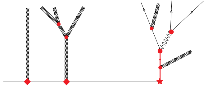
FIG. 1 (color online). Shower history for a top quark jet. The hard interaction is indicated by a star. Initial state emissions are indicated by diamonds. Parton decays are indicated by large filled circles and QCD splittings are indicated by small filled circles.
