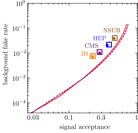
FIG. 5 (color online). Results using HERWIG++ compared to those using PYTHIA from Fig. 4. The solid curve is the F versus A curve from shower deconstruction using events generated with PYTHIA; the dashed curve uses events generated with HERWIG++. The solid circles show F versus A results for the top taggers using events generated with PYTHIA; the open squares use events generated with HERWIG++.
