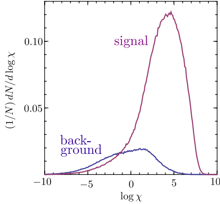
FIG. 3 (color online). (1/N)dN/d \log \chi for signal events (upper curve) and (1/N)dN/d \log \chi for background events (lower curve) for samples of signal and background events generated by PYTHIA. We use the cuts described in Sec. IVA.
