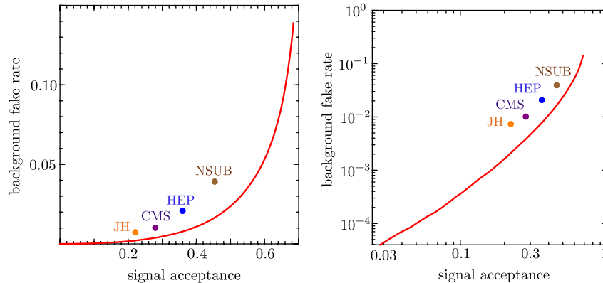
FIG. 4 (color online). Background fake rate F as a function of signal acceptance A for shower deconstruction with the signal and background event samples described in Sec. IVA. The curve for shower deconstruction is compared to F versus A points for the JH top tagger, the top tagger of the CMS group (CMS), the HEP top tagger, and the use of NSUB as a top tagger. We show the results on a linear scale (left) and on a logarithmic scale (right).
