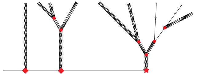
FIG. 2 (color online). Shower history for a QCD jet.
