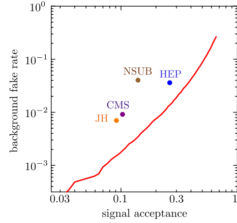
FIG. 6 (color online). Background fake rate F as a function of signal acceptance A for shower deconstruction with the signal and background event samples using a 200 GeV cut on jet P_T and a fat jet cone size of R = 1.5 , as described in Sec. V. The curve for shower deconstruction is compared to F versus A points for the JH top tagger, the top tagger of the CMS group (CMS), the HEP top tagger, and the use of NSUB as a top tagger.
