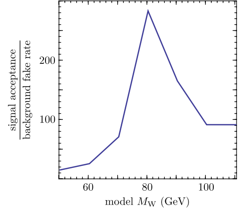
FIG. 8 (color online). Signal acceptance divided by background fake rate for a cut \chi > 384 as a function of the W mass, M_W^{\text{model}} , used in the shower deconstruction algorithm. There is a peak at the true W mass.
