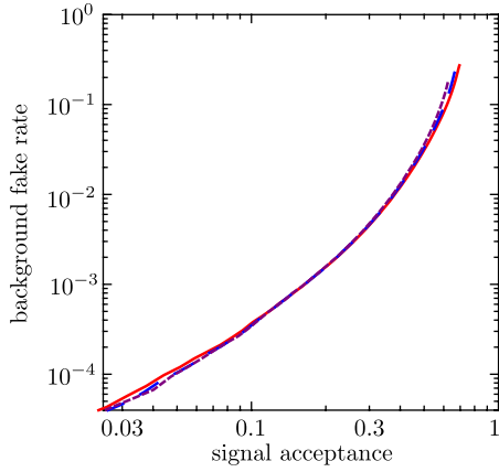
FIG. 7 (color online). Shower deconstruction results for highly boosted jets ( P_T > 800 GeV) showing the dependence on the cone size of the fat jet. The solid curve is the F versus A curve from shower deconstruction for fat jets defined with R = 1.50 ; the long dashed curve uses jets with R = 1.25 ; the short dashed curve uses jets with R = 1.00 .
