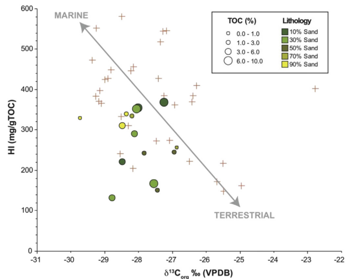
Figure 8. HI (kerogen and maturity dependent) plot versus carbon isotope ratios of organic matter from core depths between 3500–4300 m (UK Quadrant 16, South Viking Graben). Red crosses are from equivalent public data in adjacent Norwegian wells (NPD 2015). (For interpretation of the references to colour in this figure legend, the reader is referred to the web version of this article.)
