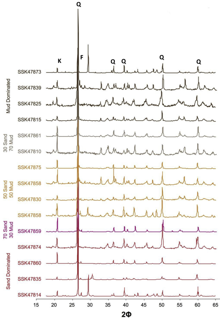
Figure 6. X-ray diffraction (XRD) pattern (Cu K \alpha radiation) of sandstone and mudstones samples. Q = Quartz, K = Kaolinite, F = Plagioclase Feldspar.
