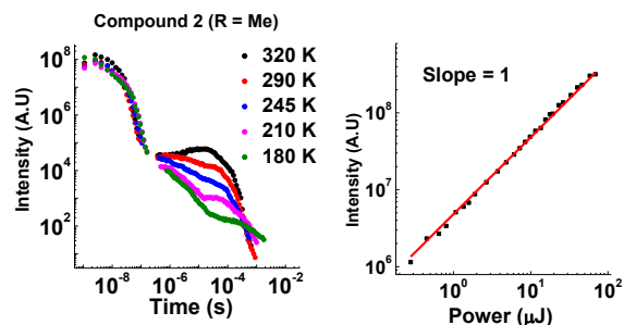
Fig. 5 Left: Temperature dependence of emission decay in toluene for 2 . Right: Power dependence of DF emission in toluene for 2 (400 ns delay and 50 \mu\text{s} integration time).
