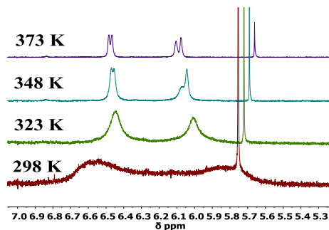
Fig 3 500 MHz Variable temperature ^1\text{H} NMR experiments for 4 from 298 – 373 K in \text{DMSO-d}_6 .
