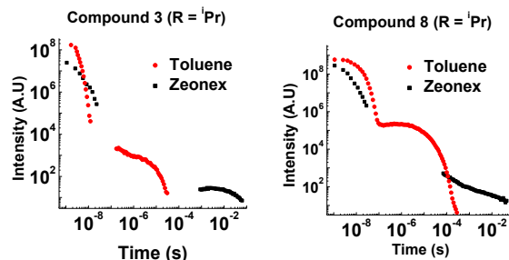
Fig 7. Time-resolved emission decay for 3 and 8 at 290 K (355 nm excitation).
