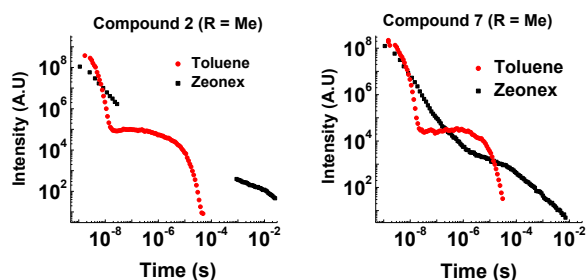
Fig 4. Time-resolved emission decay for 2 and 7 at 290 K (355 nm excitation).
