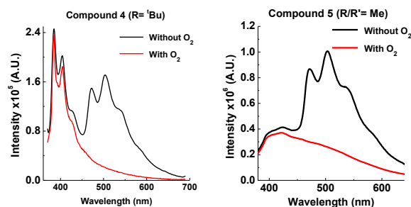
Fig. 9 Emission of 4 and 5 at 290 K in zeonex (excited at 355 nm).
