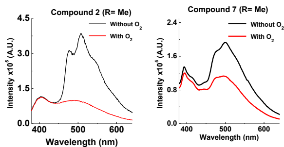
Fig. 6 Emission of 2 and 7 at 290 K in zeonex (excited at 355 nm).
