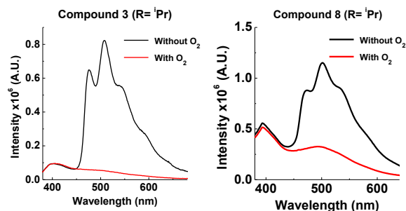
Fig. 8 Emission of 3 and 8 at 290 K in zeonex (excited at 355 nm).
