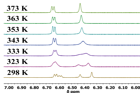
Fig. 2 500 MHz Variable temperature 1 H NMR experiments for 3 from 298 – 373 K in DMSO- d 6 .
