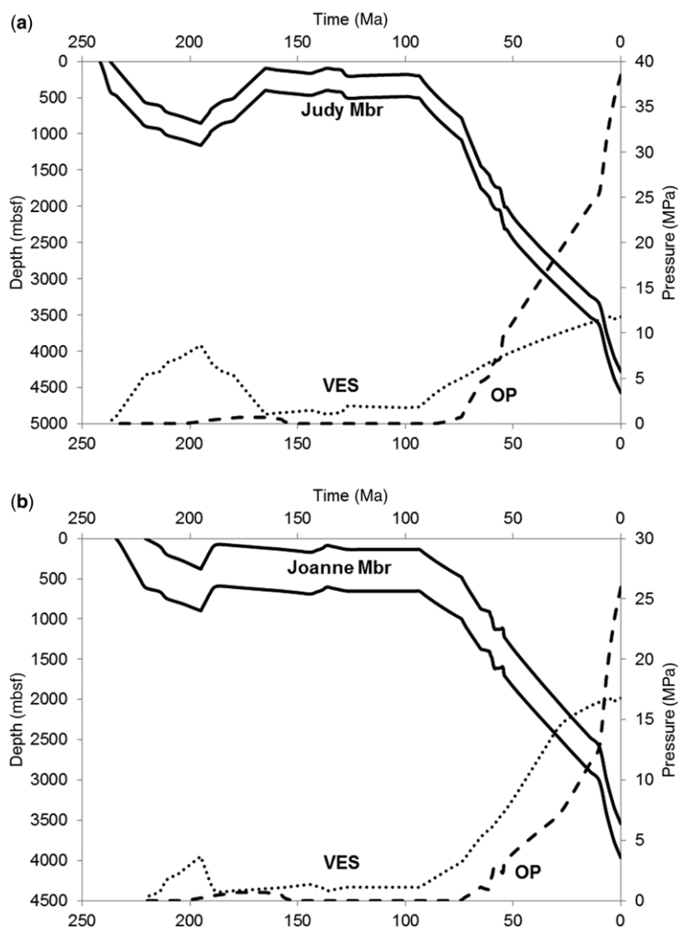
Fig. 12. Burial history (solid lines), pore fluid overpressure (OP; dashed lines) and vertical effective stress (VES; dotted lines) development for (a) the Judy Sandstone Member, the uppermost succession within the Skagerrak Formation in the Heron well (22/29-5) and (b) the Joanne Sandstone Member, the uppermost succession within the Skagerrak Formation in the Judy well (30/7a-9).
