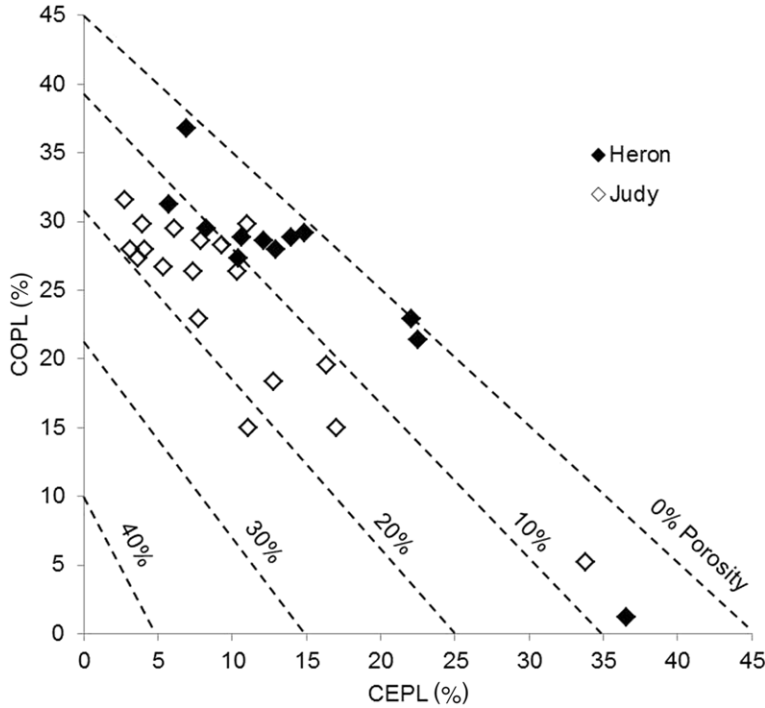
Fig. 10. Mechanical compaction (COPL) and cementational (CEPL) porosity loss for the Heron and the Judy sample set. After Lundegard (1992).
