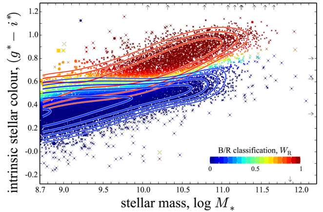
Figure 11. Illustrating our objective B/R classifications, based on the intrinsic (g^* - i^*) CMD. All symbols and their meanings are analogous to Fig. 10. Note how, particularly at higher masses, the R population is more unambiguously distinguished in the (g^* - i^*) CMD than the (g - i) CMD shown in Fig. 10; only a small fraction of galaxies have ambiguous classifications (i.e. intermediate values of W_R ). As discussed in Sections 7.2 and 7.3, this means that our empirical determinations of the MFs for B/R classified galaxies are not strongly dependent on the quality of our fits. At lower masses, and particularly around \log M_* \sim 9.5 , the populations are inferred to overlap to the extent that up to \sim 20 per cent of galaxies in the blue sequence are members of the R population. The overlap between the two populations in this figure, as well as Fig. 10 demonstrate the importance of accounting for scatter around the CMR when characterizing the two populations.
