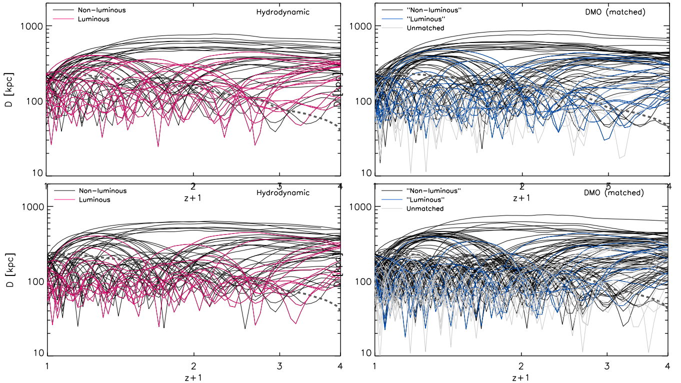
Figure 9. Evolution of galactocentric distance for dark and luminous satellites of the simulated ‘Milky Way’, as identified directly in the hydrodynamic simulation (left column), or as matched from the DMO simulation (right column) at resolution L1. Satellite haloes are selected by present-day mass in the range 10^8 – 10^9 M_\odot (top row) or present v_{\max} in the range 12 – 20 \text{ km s}^{-1} (bottom row). In each panel, the grey dashed line shows the evolution of the host halo’s virial radius, r_{200} , in both simulations. Within this range of mass or v_{\max} , the orbits of luminous and dark haloes differ significantly. Also note the lower number of objects in the hydrodynamic simulation compared to the DMO simulation, due to the reduction of v_{\max} and mass of individual haloes by baryonic effects.
