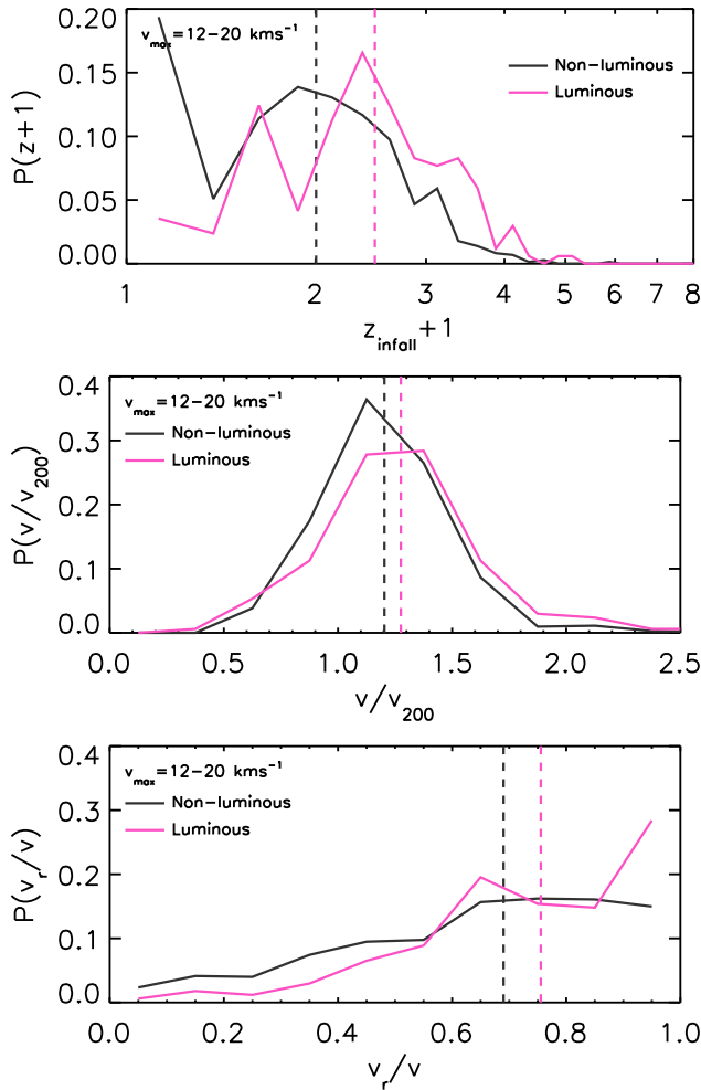
Figure 10. Top panel: distribution of infall redshifts of luminous and non-luminous satellites in the present-day v_{\max} range of 12\text{--}20\text{ km s}^{-1} , from 12 volumes at resolution L2. Middle panel: distributions of infall velocities of satellites in the divided by v_{200} of the host halo at the time of infall. Bottom panel: distributions of the ratio between the radial component and the total infall velocity. Dashed lines indicate the median values on all panels. Luminous haloes in this v_{\max} range fell in significantly earlier, with higher velocities and on more radial orbits compared to non-luminous haloes.
