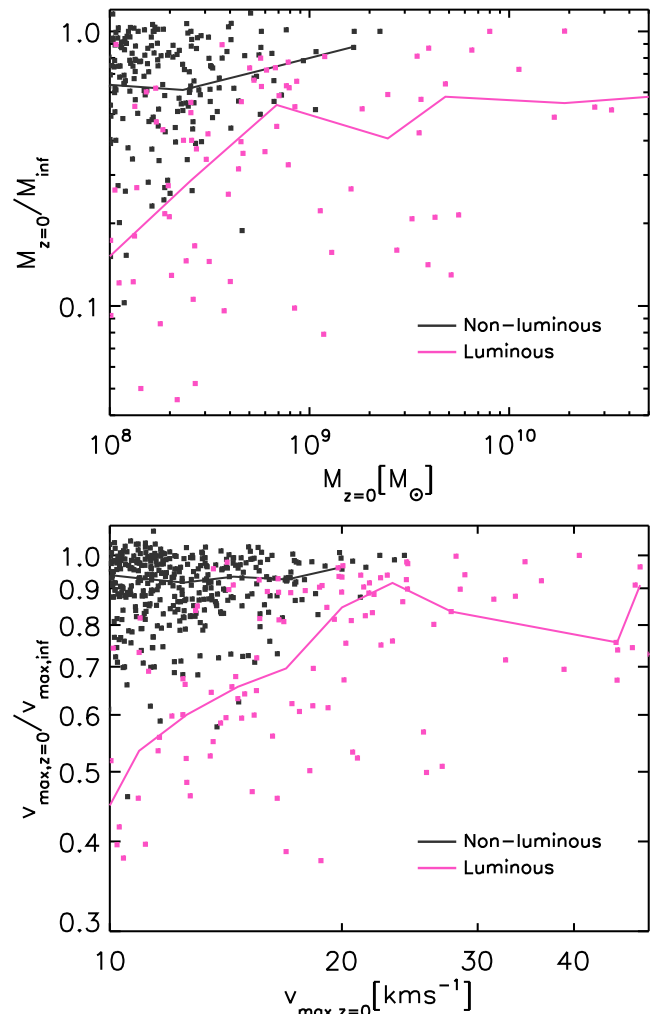
Figure 11. Change in mass relative to mass at z_{\text{infall}} as a function of present mass (top panel), and change in v_{\max} relative to v_{\max} at z_{\text{infall}} as a function of present v_{\max} (bottom panel), for luminous and non-luminous satellite haloes of the parent halo shown in Fig. 9, at resolution L1. Lines indicate the median values. As haloes with infall masses < 10^{9.5} M_{\odot} or v_{\max} < 25\text{ km s}^{-1} are unlikely to host galaxies, luminous haloes with such lower present values are likely to have experienced a much more significant decrease in mass and v_{\max} from their peak values compared to non-luminous haloes.
